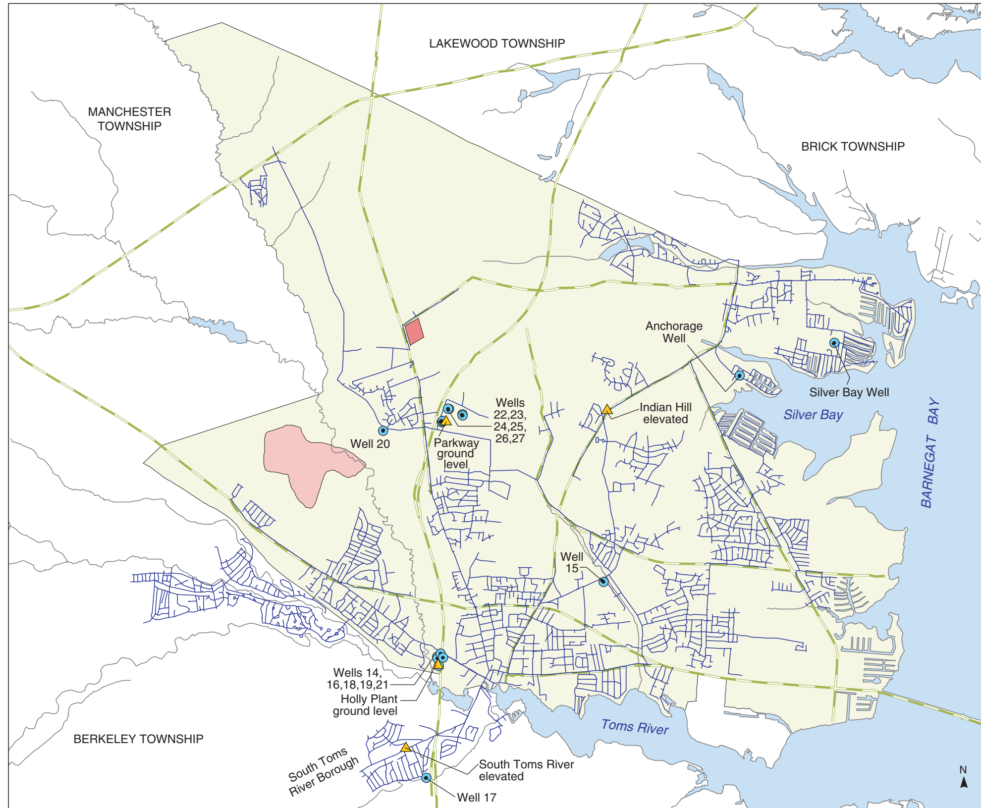
PLATE 15. WATER-DISTRIBUTION SYSTEM SERVING THE DOVER TOWNSHIP AREA, NEW JERSEY, 1974 By Morris L. Maslia, Jason B. Sautner, Mustafa M. Aral, Richard E. Gillig, Juan J. Reyes, and Robert C. Williams
