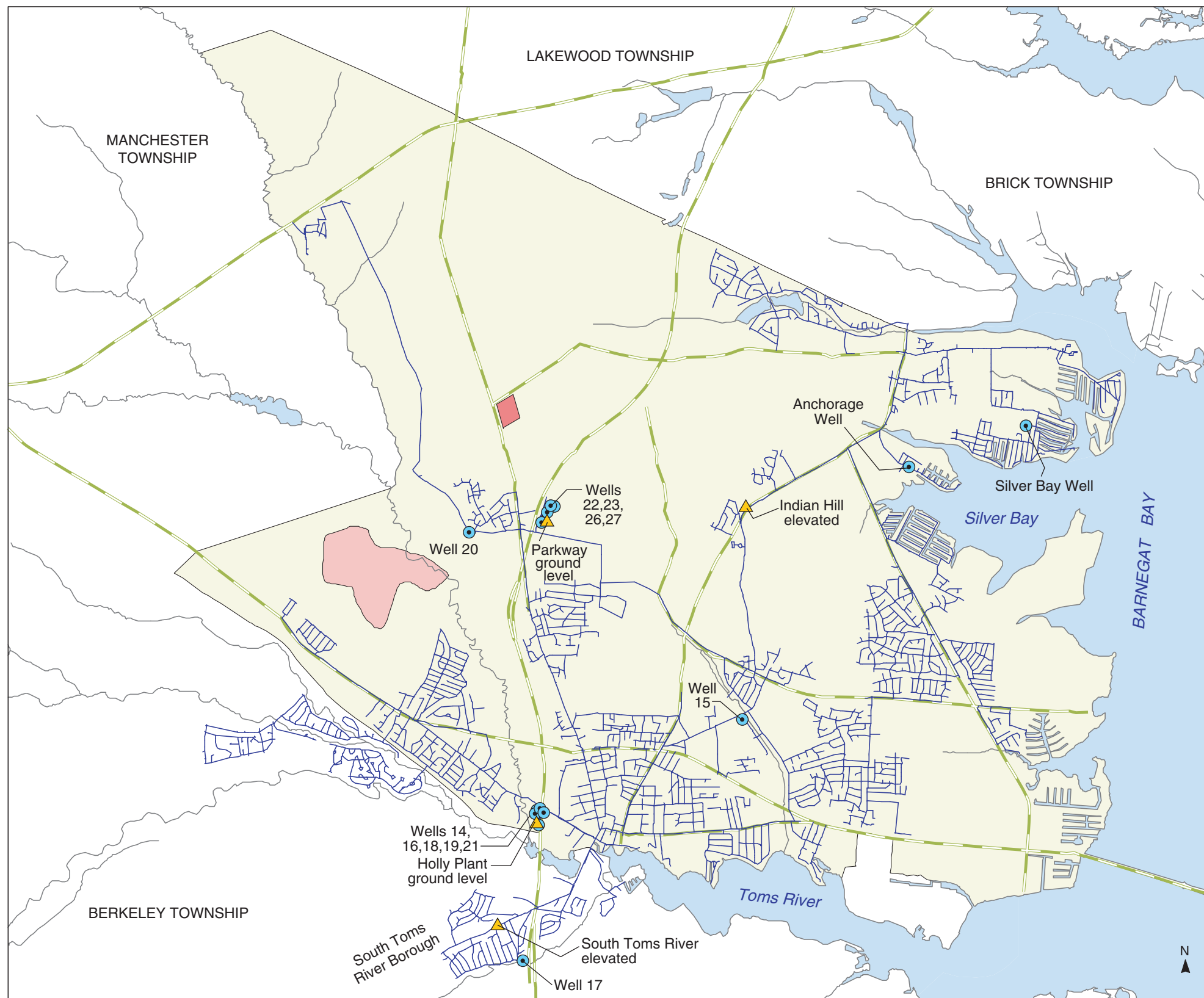
PLATE 12. WATER-DISTRIBUTION SYSTEM SERVING THE DOVER TOWNSHIP AREA, NEW JERSEY, 1971 By Morris L. Maslia, Jason B. Sautner, Mustafa M. Aral, Richard E. Gillig, Juan J. Reyes, and Robert C. Williams
