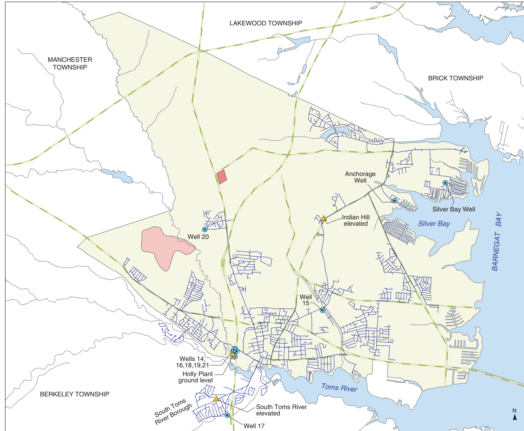
PLATE 10. WATER-DISTRIBUTION SYSTEM SERVING THE DOVER TOWNSHIP AREA, NEW JERSEY, 1969
