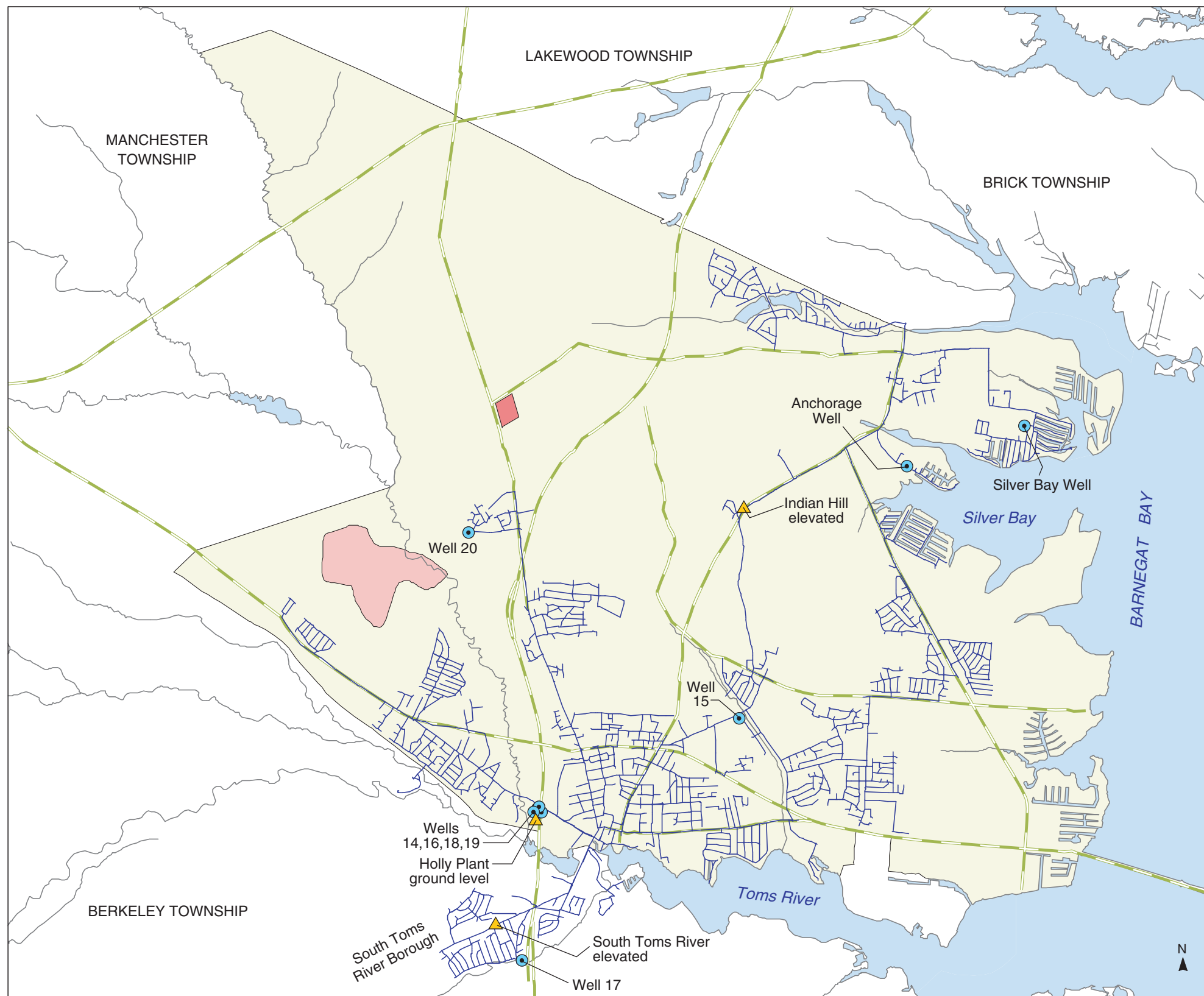
PLATE 9. WATER-DISTRIBUTION SYSTEM SERVING THE DOVER TOWNSHIP AREA, NEW JERSEY, 1968 By Morris L. Maslia, Jason B. Sautner, Mustafa M. Aral, Richard E. Gillig, Juan J. Reyes, and Robert C. Williams
