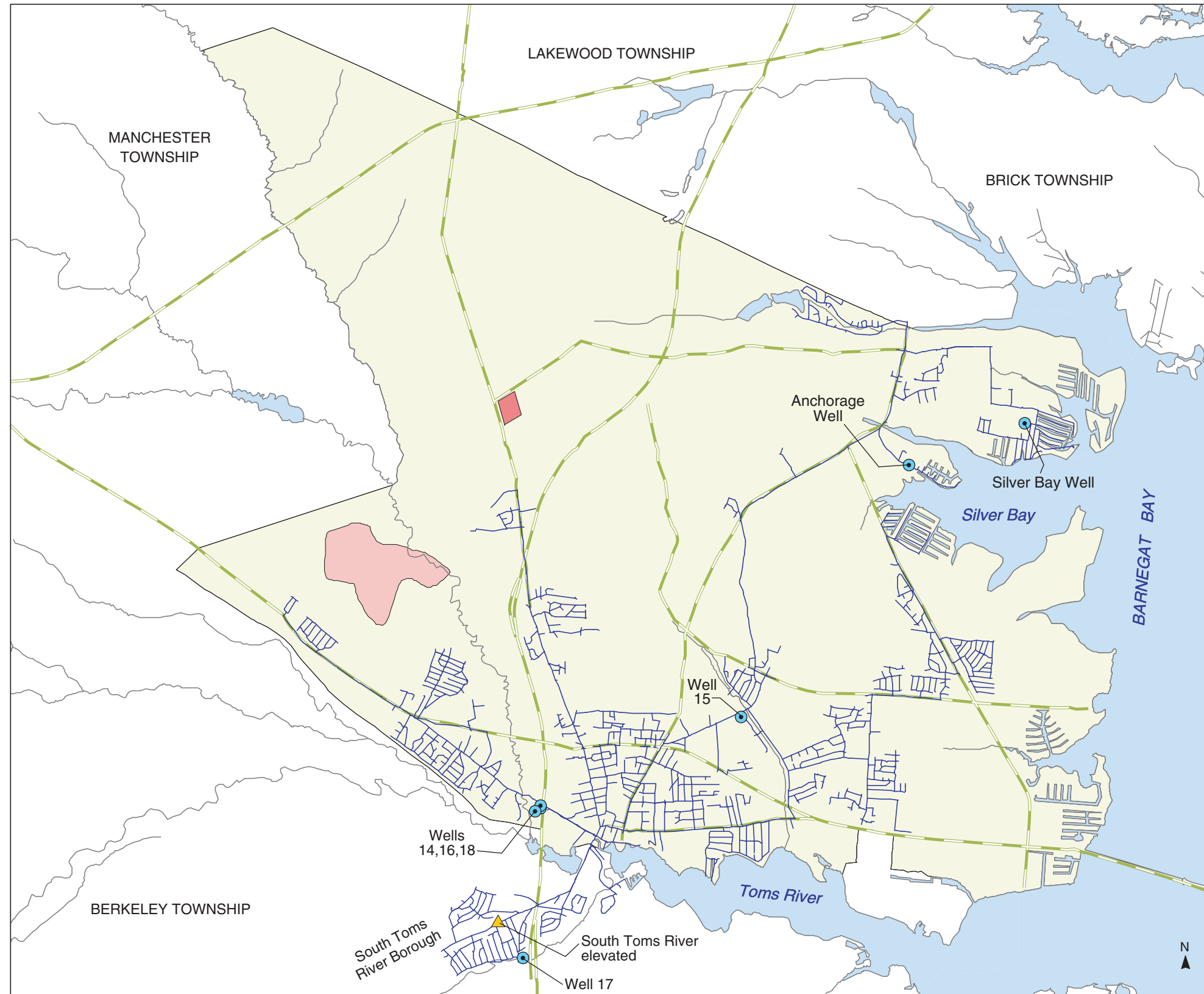
PLATE 7. WATER-DISTRIBUTION SYSTEM SERVING THE DOVER TOWNSHIP AREA, NEW JERSEY, 1966 By Morris L. Maslia, Jason B. Sautner, Mustafa M. Aral, Richard E. Gillig, Juan J. Reyes, and Robert C. Williams
