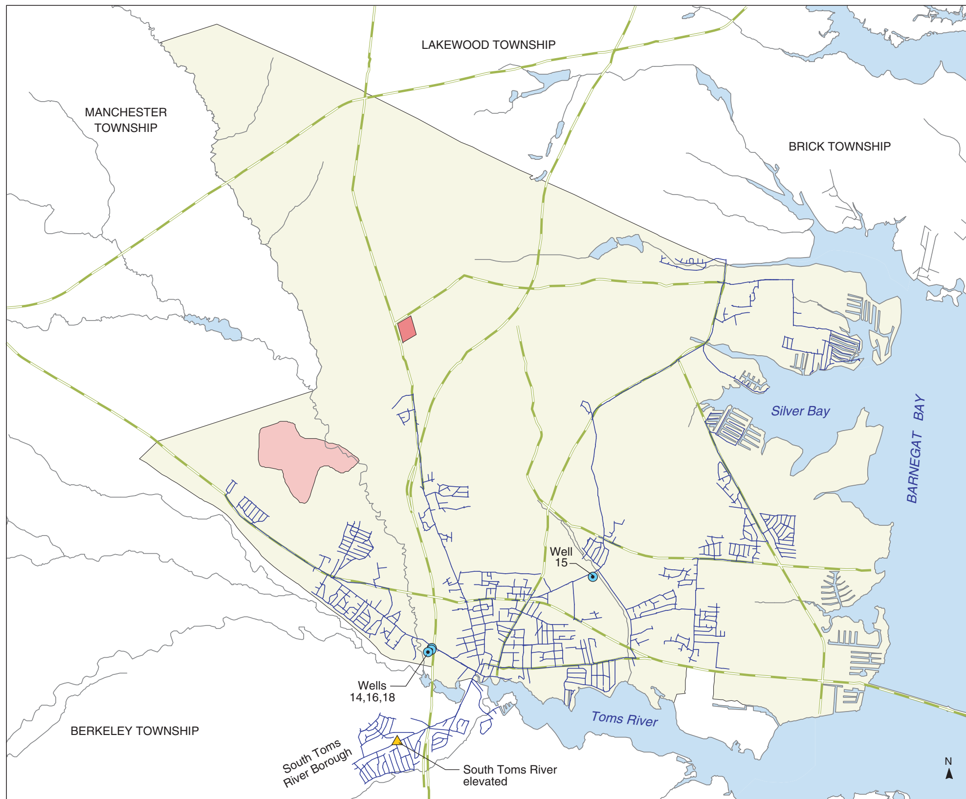
PLATE 6. WATER-DISTRIBUTION SYSTEM SERVING THE DOVER TOWNSHIP AREA, NEW JERSEY, 1965 By Morris L. Maslia, Jason B. Sautner, Mustafa M. Aral, Richard E. Gillig, Juan J. Reyes, and Robert C. Williams
