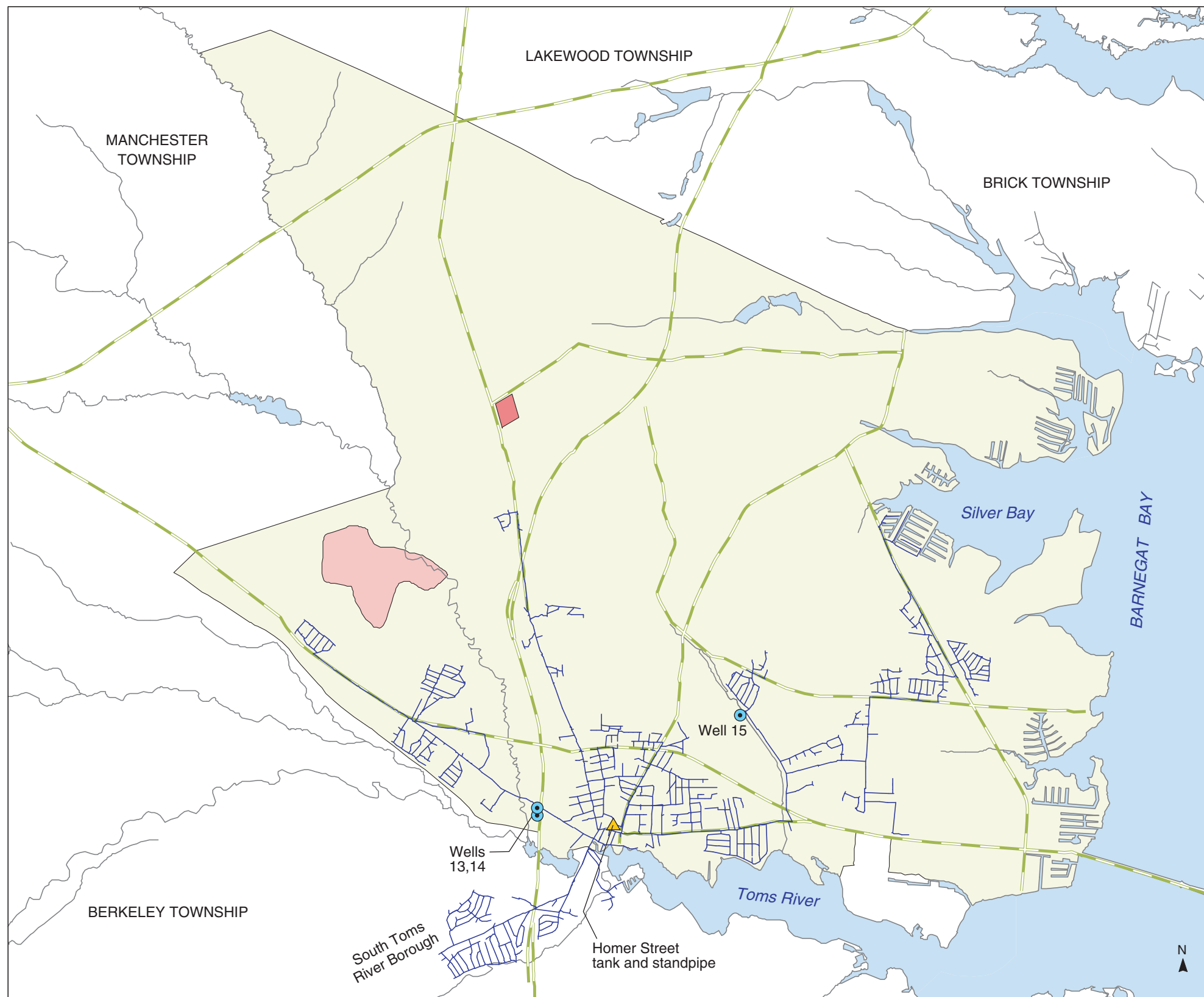
PLATE 3. WATER-DISTRIBUTION SYSTEM SERVING THE DOVER TOWNSHIP AREA, NEW JERSEY, 1962 By Morris L. Maslia, Jason B. Sautner, Mustafa M. Aral, Richard E. Gillig, Juan J. Reyes, and Robert C. Williams
