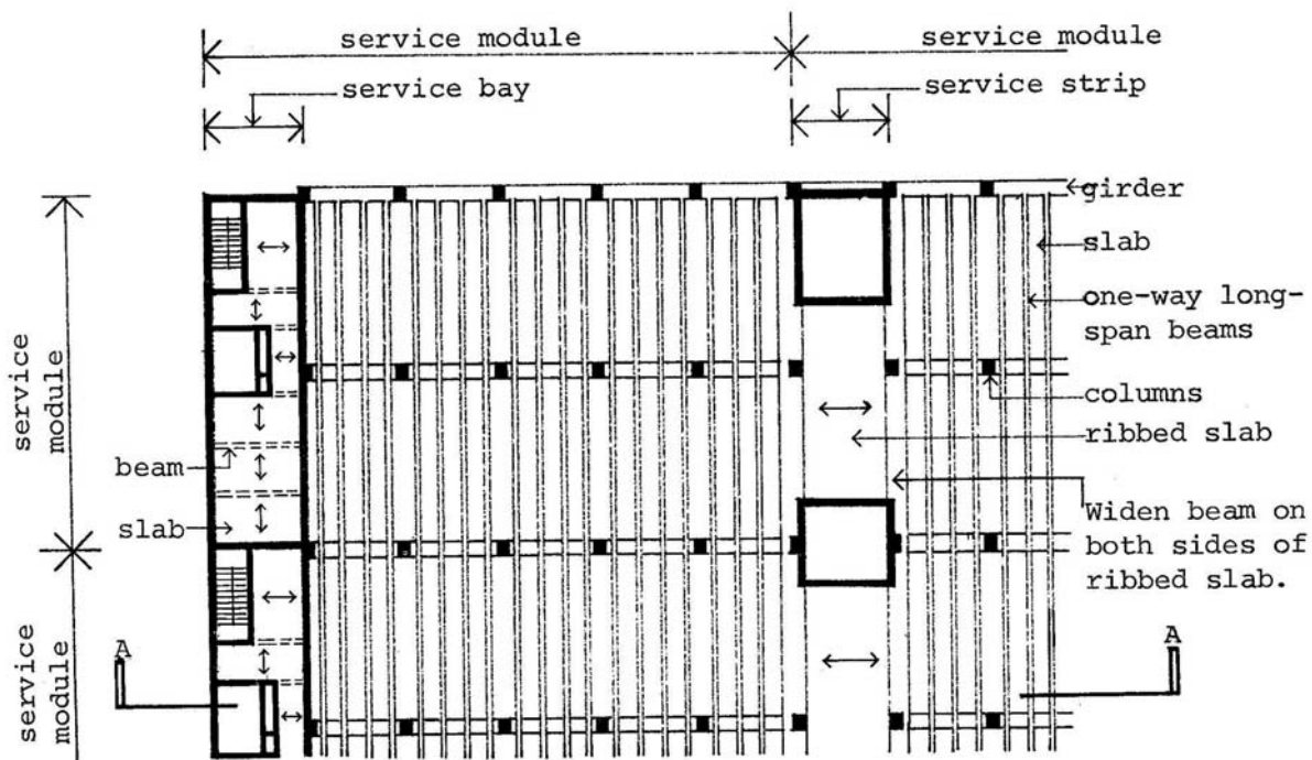
PLAN SHOWING PORTION OF A FLOOR INCORPORATING SERVICE STRIPS
