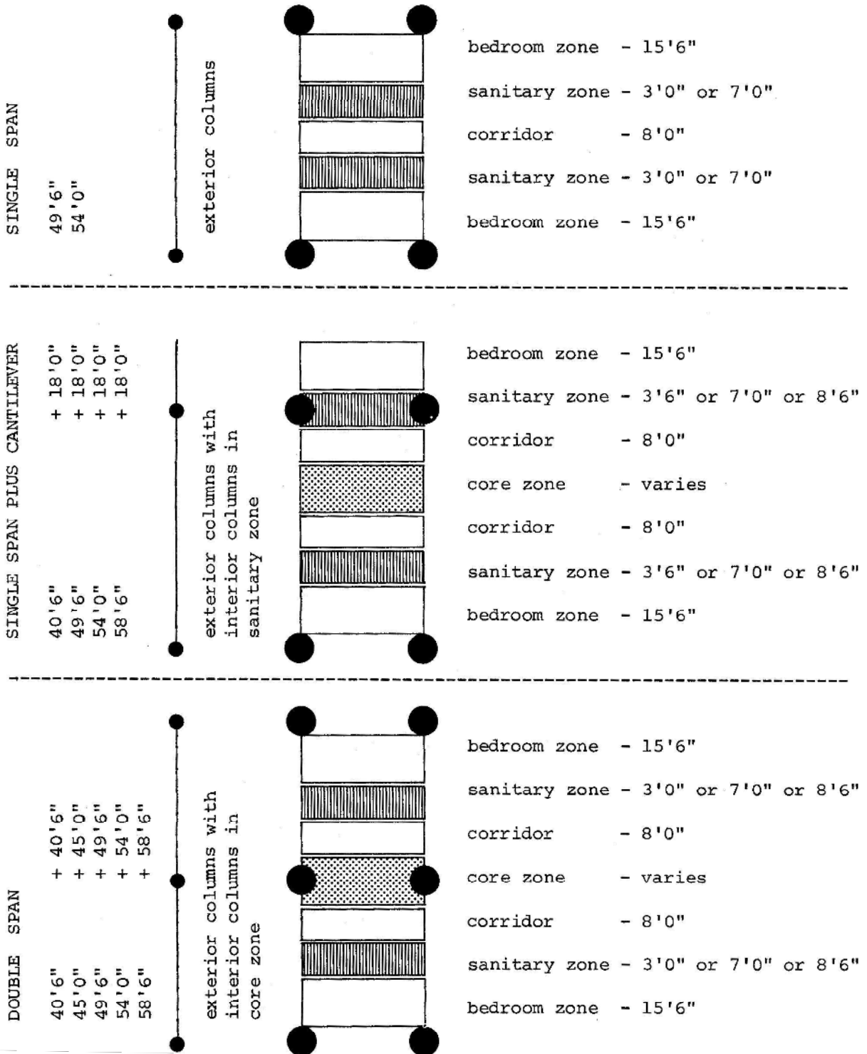
Figure 230-2. PLAN ZONES
