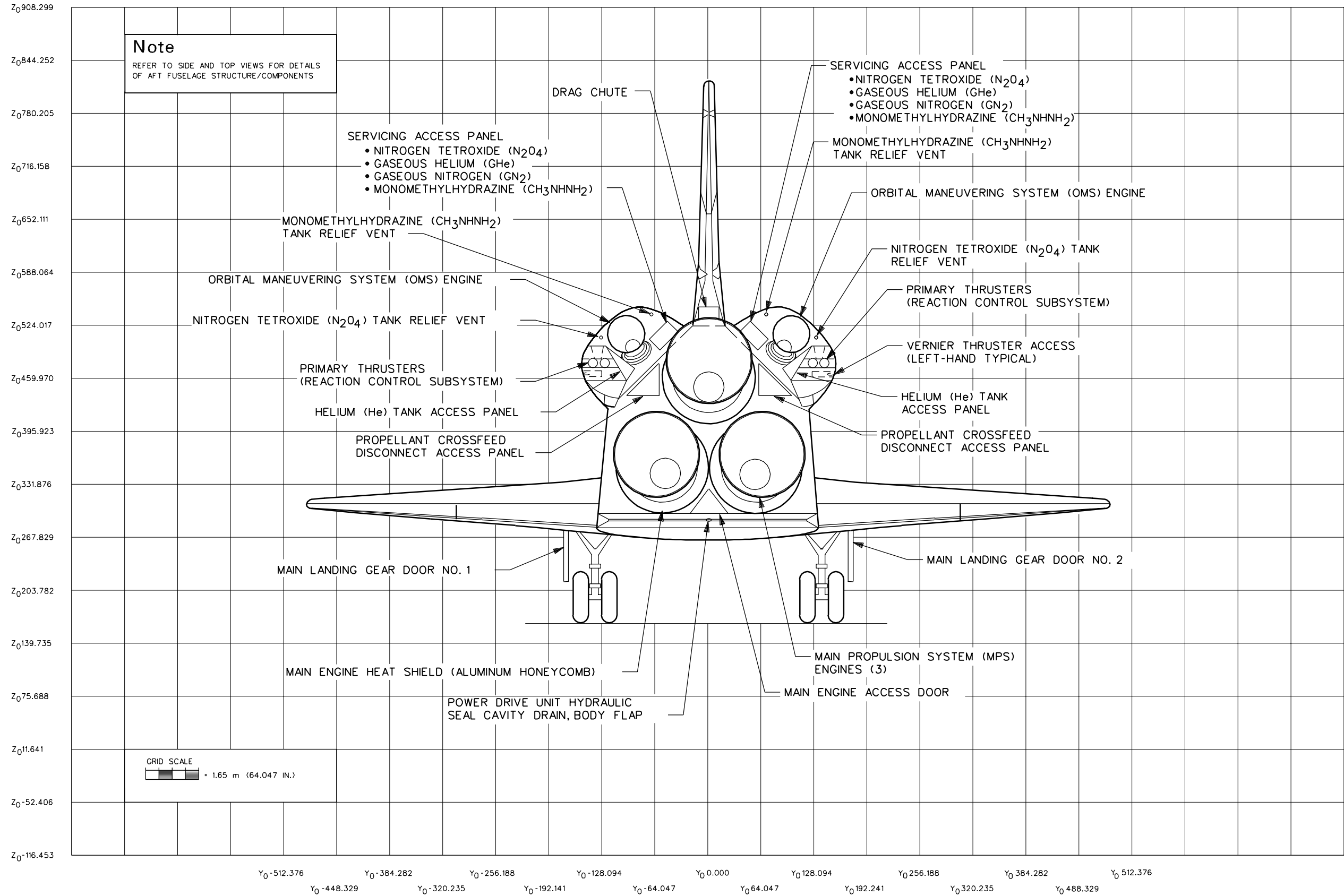
(a) Moldline penetrations/access panels.
