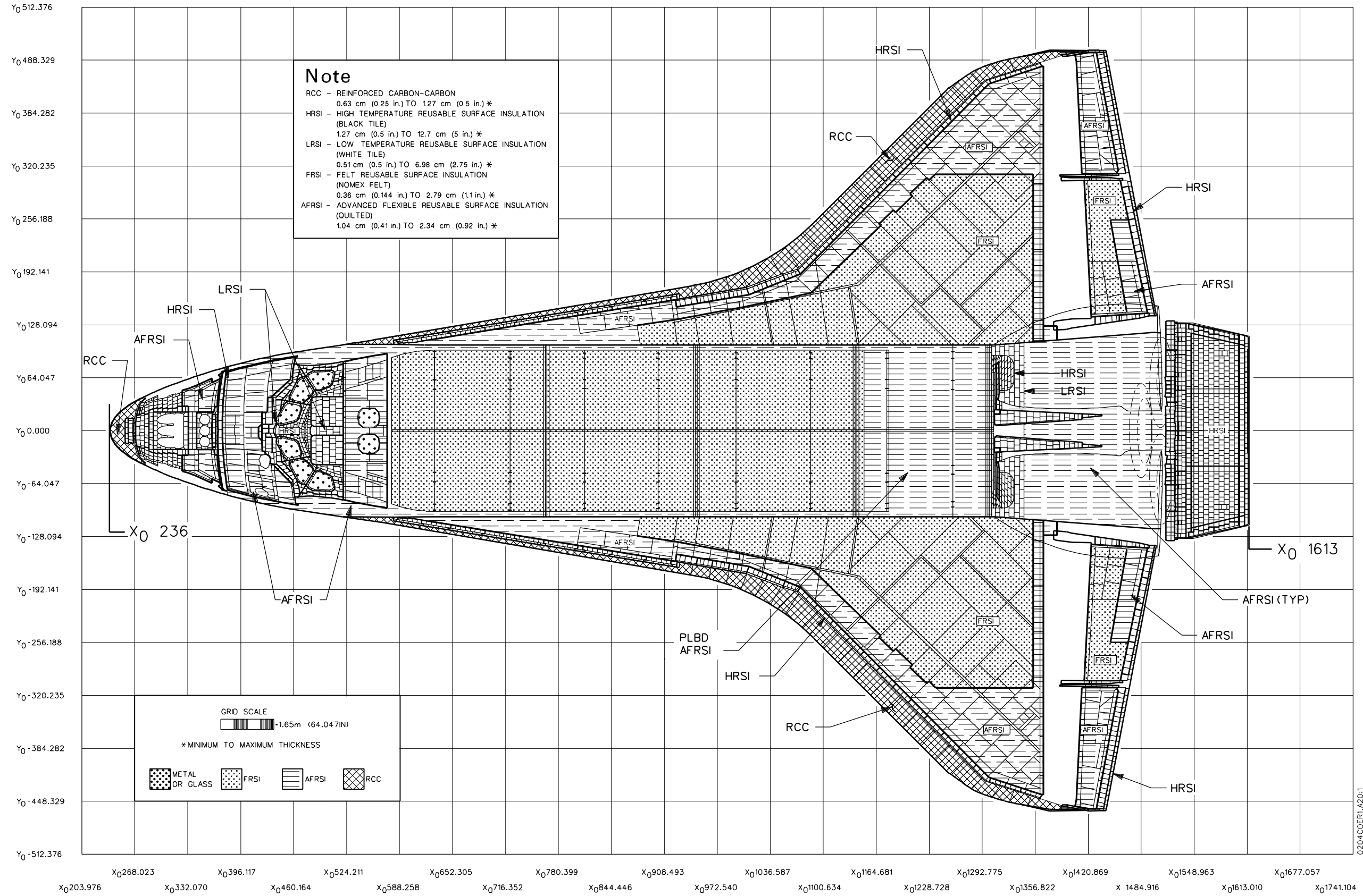
(c) Exterior finish/external insulation - OV103 (Discovery), OV104 (Atlantis) and OV105 (Endeavour). Figure 2-4.- Continued.
