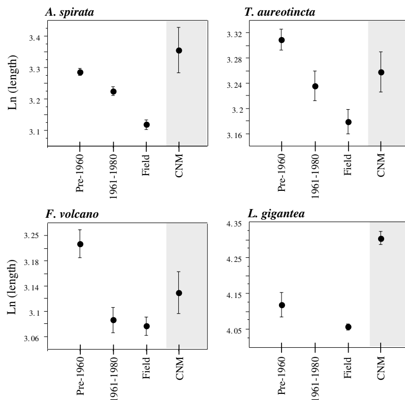
Figure 2 Mean sizes (log-transformed) of each species (with 95% confidence intervals) in individual temporal bins described in the text. The shaded area represents data from the only well-protected intertidal reserve in California (see text). As a result of small sample size, the second baseline was not calculated for Lottia gigantea . For Fissurella volcano , data are for San Diego County only. All pairwise comparisons of baselines, field samples and Cabrillo National Monument (CNM) reveal significant differences at 0.05 level or better (Kolmogorov–Smirnov tests with sequential Bonferroni corrections (Rice 1989), with the exception of Field–2nd Baseline ( P = 0.90 ) and Field–CNM ( P = 0.06 ) for F. volcano .
