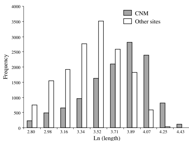
Figure 3 Size distributions of Lottia gigantea measured at fixed replicate quadrats over multiple years at Cabrillo National Monument (CNM) and less protected sites (see text). The distributions are significantly different ( P < 0.0001 Kolmogorov–Smirnov test).
