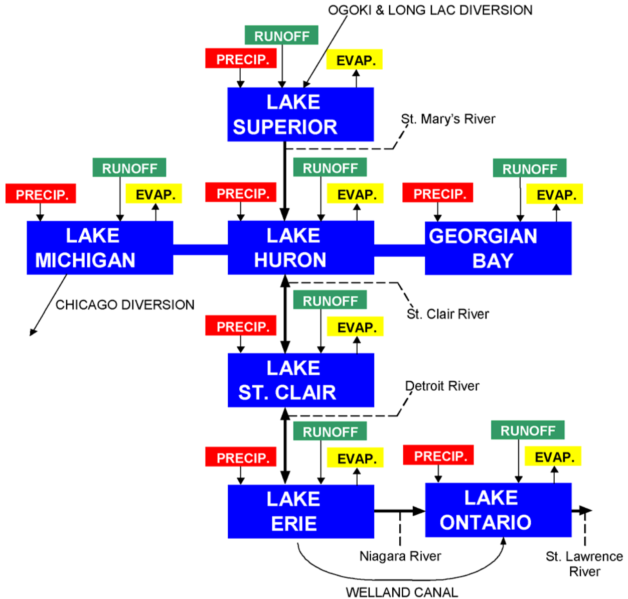
Figure 5. Arrangement schematic of Great Lakes, connecting channels, and all water flows.
