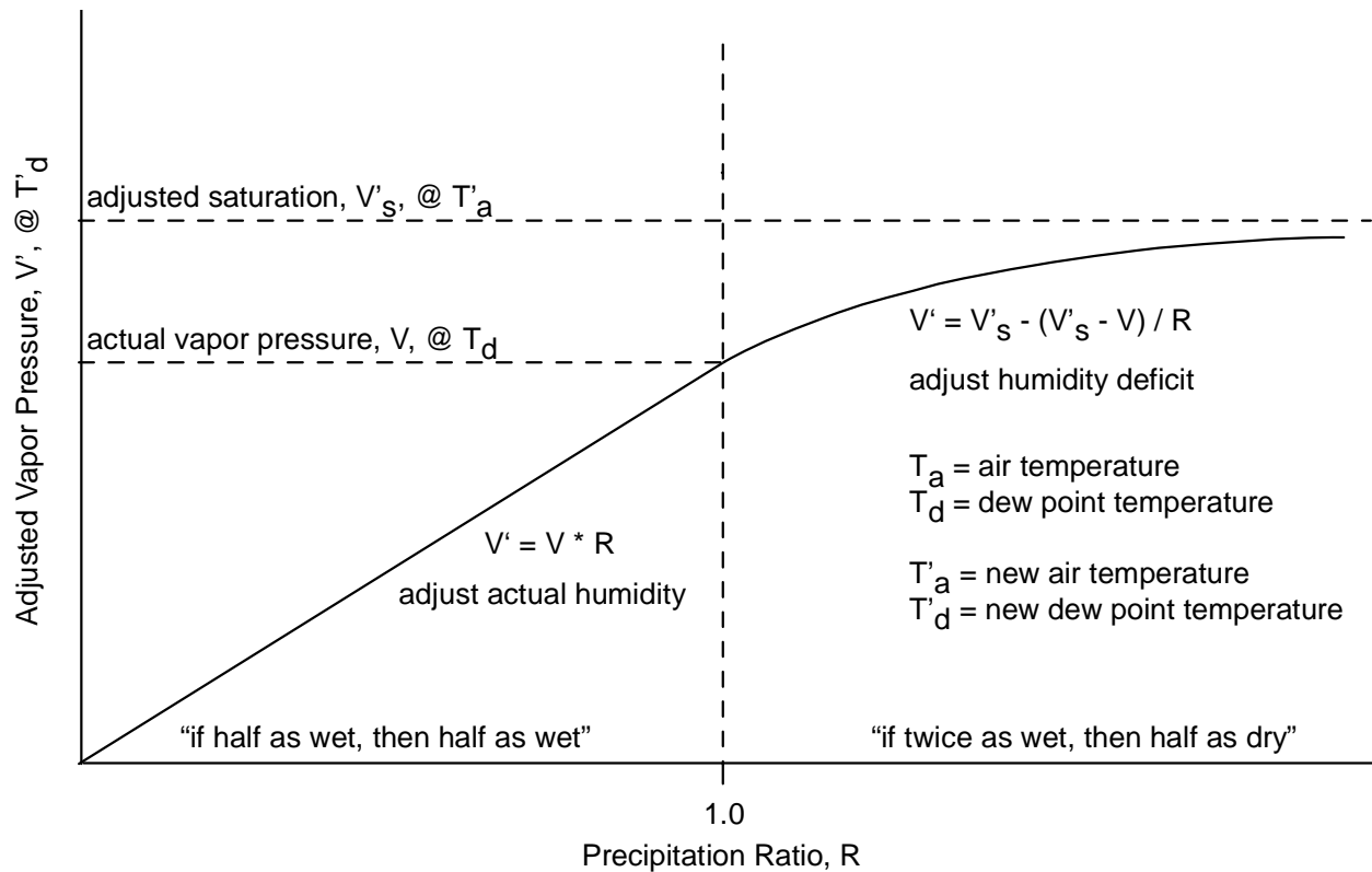
Figure 3. Humidity adjustments.
