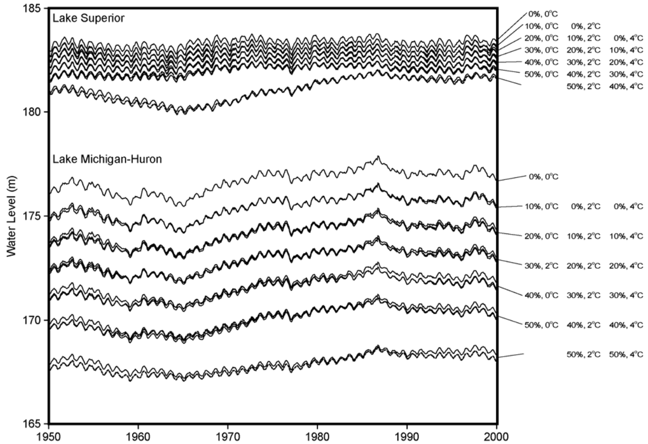
Figure 9. Steady-state upper Great Lakes water level scenarios for non-terminal lake climates.
