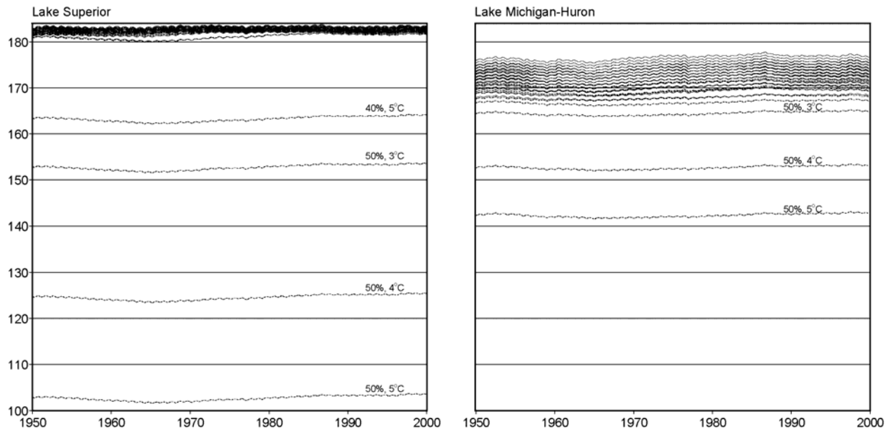
Figure 10. Steady-state upper Great Lakes water level scenarios for all climates considered.
