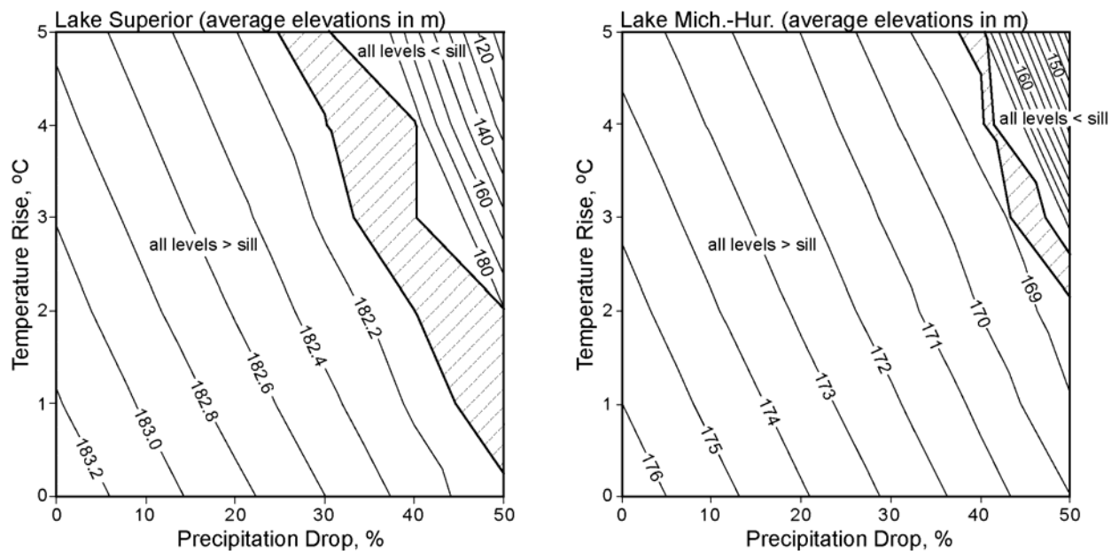
Figure 11. Steady-state upper Great Lakes average water levels as a function of temperature rise and precipitation drop relative to the present base climate.
