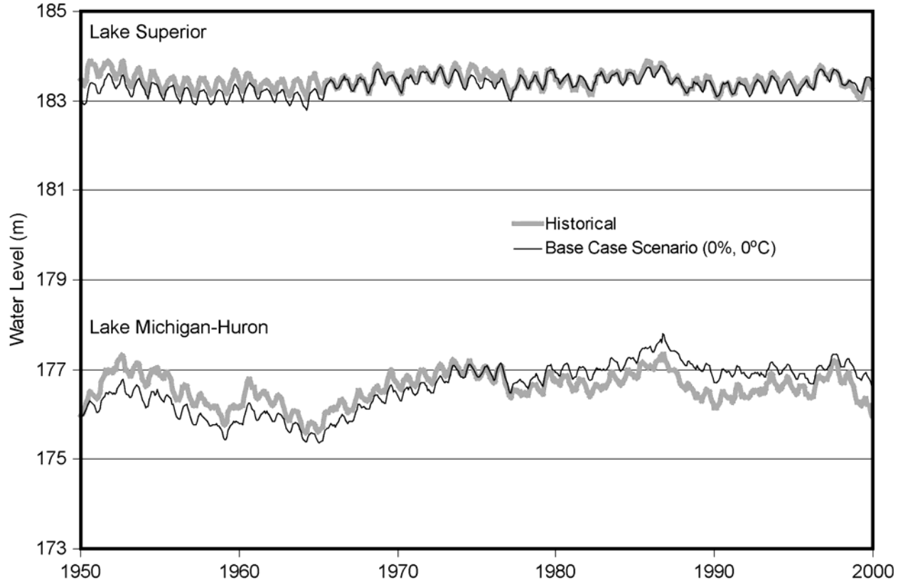
Figure 8. Matching the Lake Michigan-Huron historical water balance.
