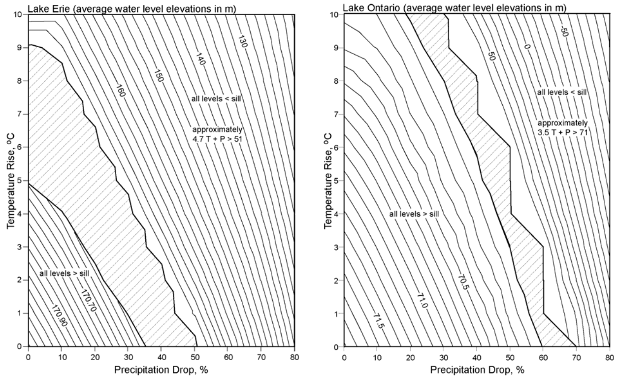
Figure 12. Steady state lower Great Lakes average water levels as a function of temperature rise and precipitation drop relative to the present base climate.
