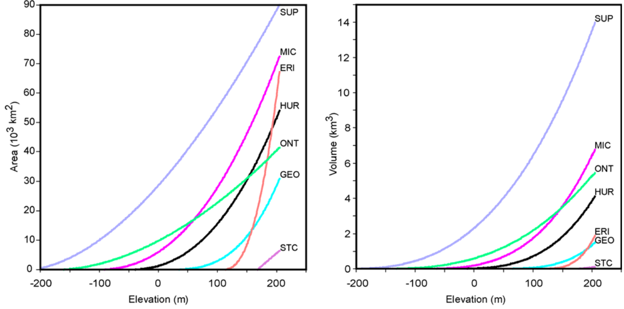
Figure 4. Great Lakes hypsometric relationships.
