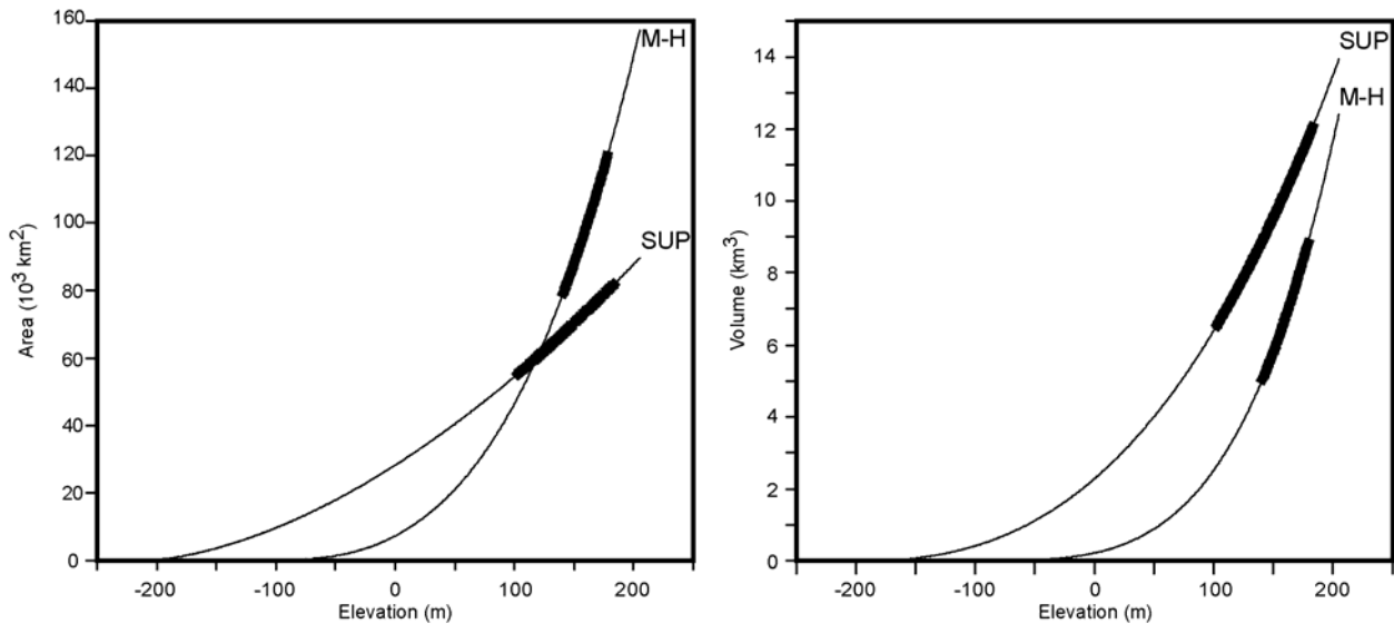
Figure 13. Steady state upper Great Lakes climate ranges for lake levels, areas, and volumes.
