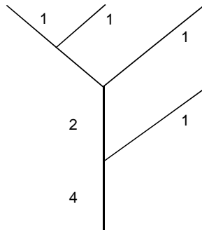
Figure 3. Example of Stream Order
