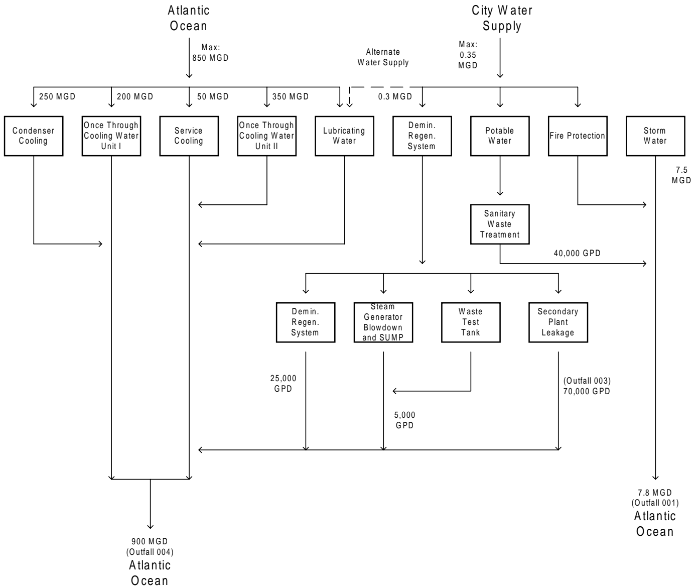
Example Flow Distribution/Water Balance Diagram
