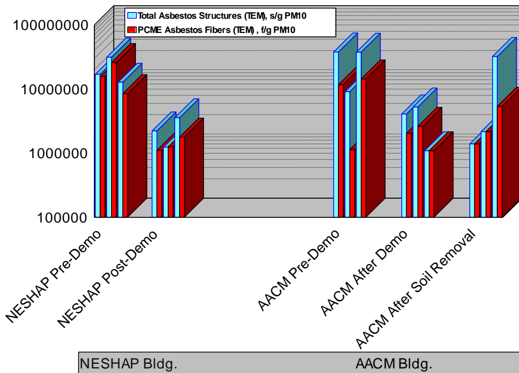
Figure 6-13. Soil elutriation air concentrations of asbestos (TEM).
