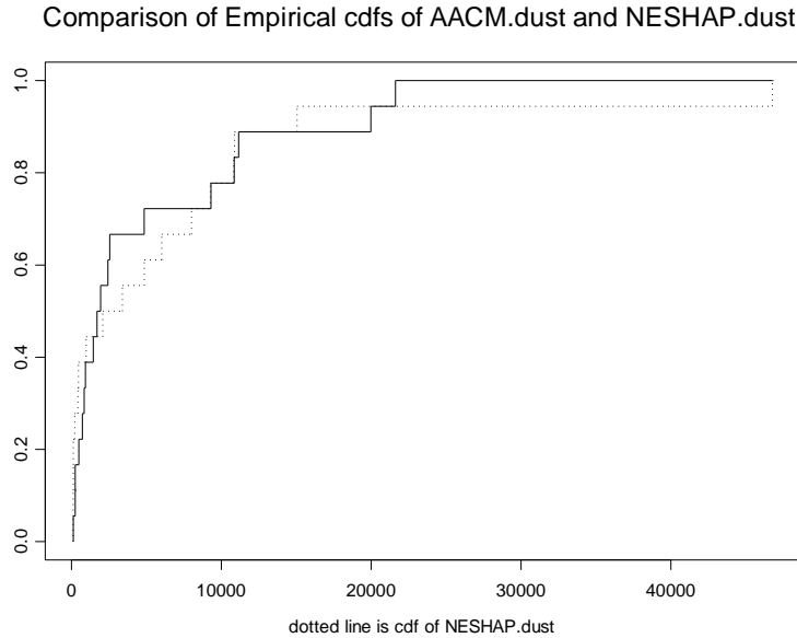
Figure 7-5. Empirical Cumulative Distributions for the Asbestos Loading in the Settled Dust ( s/cm^2 ) in the Inner Ring for the AACM and NESHAP Method.
