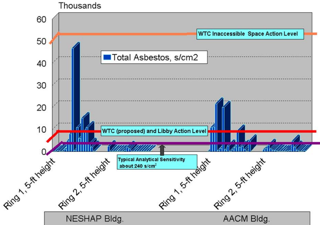
Figure 6-6. Asbestos (TEM) concentrations in settled dust resulting from the demolitions.
