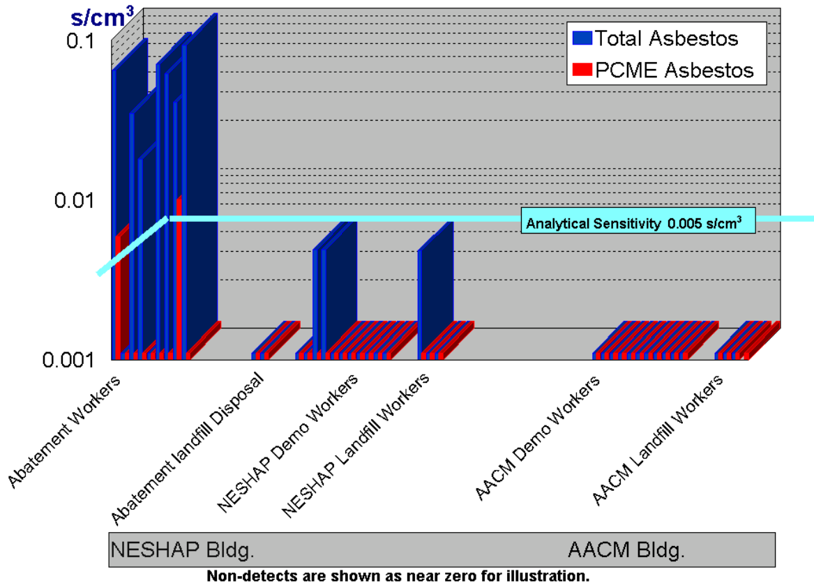
Figure 6-15. Worker breathing zone asbestos (TEM) data from the NESHAP and AACM demolition processes.
