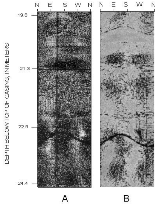
Figure 3. Amplitude images from acoustic televiewers in a 150-mm diameter borehole completed in schist with pegmatite: (A) Analog. (B) Downhole digital.
