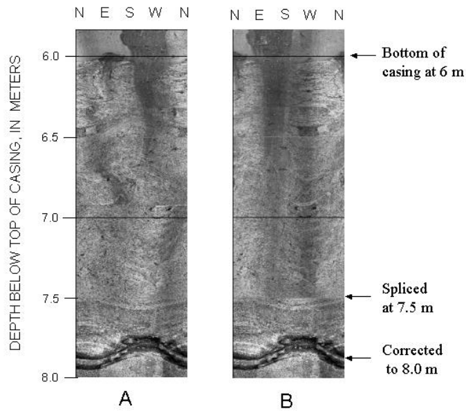
Figure 6. Optical-televiewer images in an interval in which the magnetometer is affected by steel casing: (A) Magnetometer turned on. (B) Magnetometer turned off and spliced into the oriented image.
