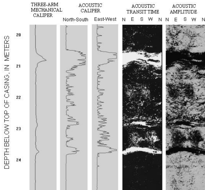
Figure 2. Three-arm mechanical and acoustic caliper logs and acoustic transit-time and amplitude televiewer images in a 150-mm diameter borehole completed in metabasalt.
