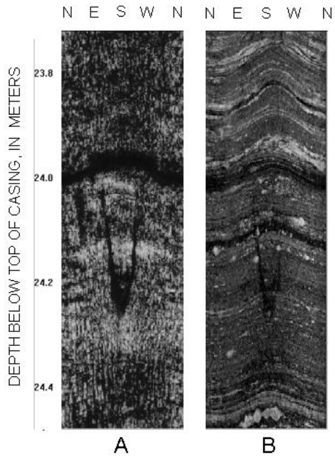
Figure 9. Televiwer images in a 150 mm diameter borehole completed in dark-colored gneiss: (A) Acoustic. (B) Optical.
