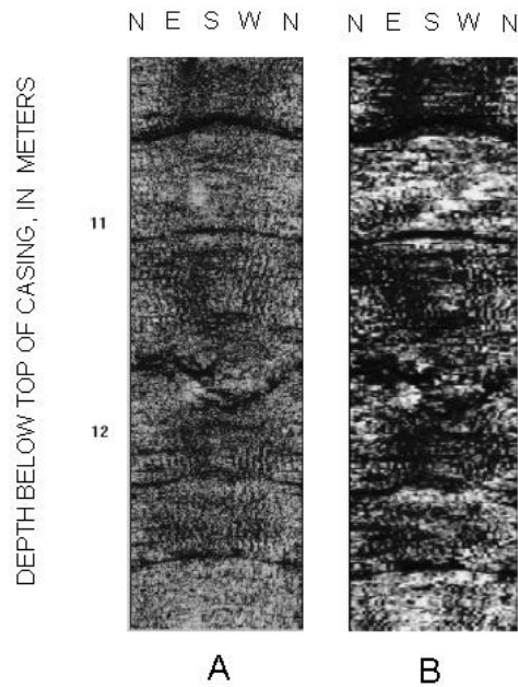
Figure 4. Amplitude images from acoustic televiewers in a 150-mm diameter borehole completed in gneiss: (A) Fixed high-frequency transducer. (B) Rotating low-frequency transducer.
