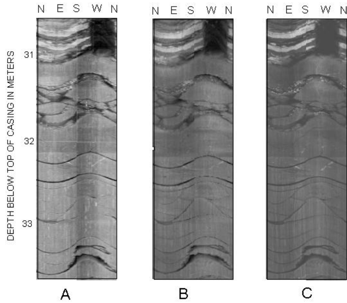
Figure 5. Optical-televiewer images of a 150-mm diameter borehole completed in sandstone: (A) Uphole-digital conical reflector. (B) Downhole-digital conical reflector. (C) Uphole-digital hyperbolic reflector.
