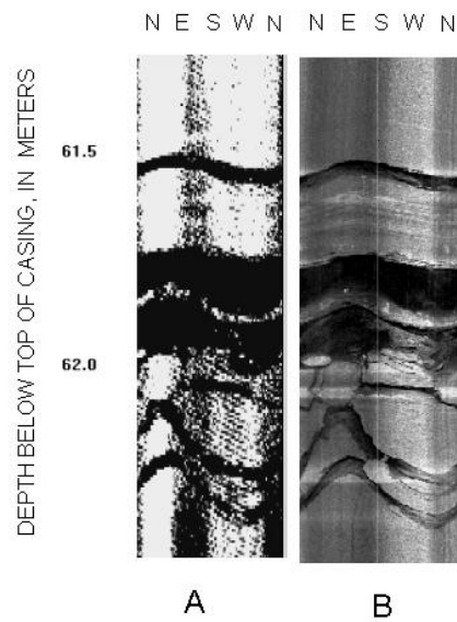
Figure 8. Televiewer images of a 75-mm diameter borehole completed in sandstone: (A) Acoustic. (B) Optical.
