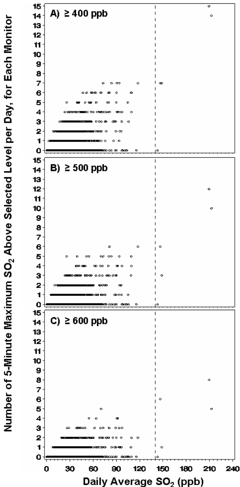
1 2 Figure 6-14. Comparison of the number of measured 5-minute maximum SO 2 3 concentrations above potential health effect benchmark levels at each 4 monitor per day and the associated daily average SO 2 concentration. 5 The 24-hour SO 2 NAAQS of 0.14 ppm is indicated by the dashed line.
