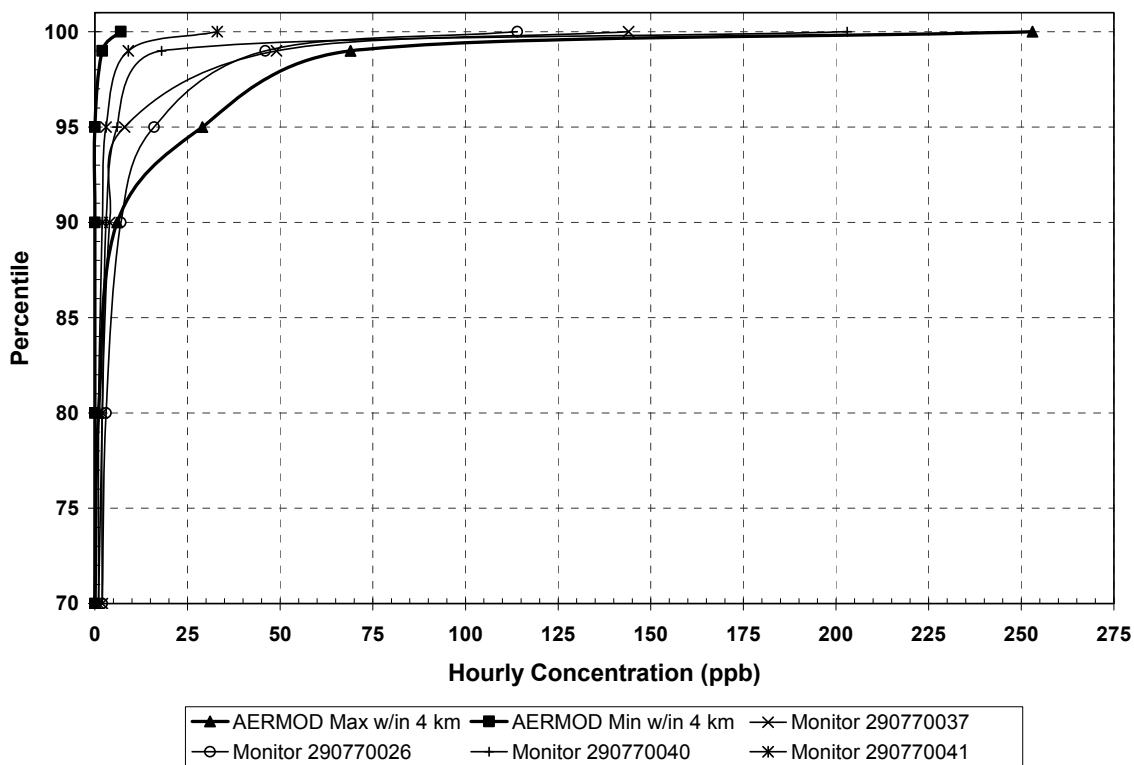
Figure 7-3. Distributions of 1-hour SO 2 concentrations in Greene County, Mo., estimated by AERMOD and measured at four ambient monitors.
