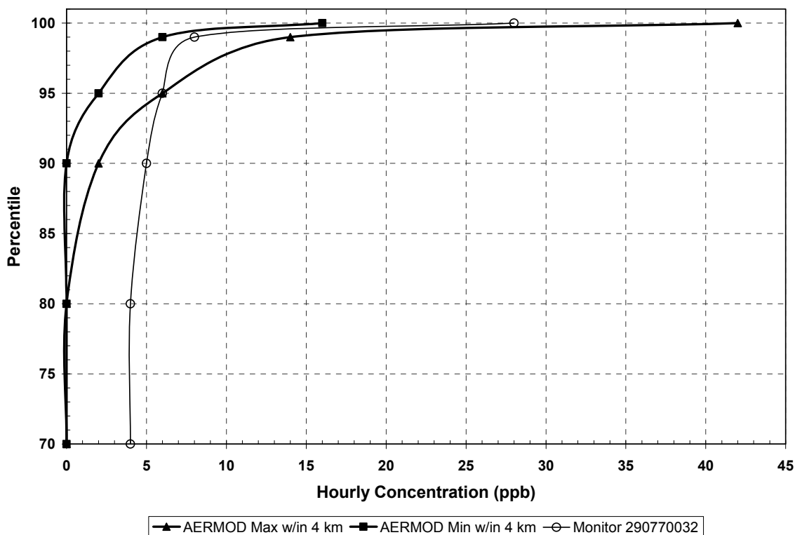
1 2 Figure 7-4. Distributions of 1-hour SO 2 concentrations in Greene County, Mo., 3 estimated by AERMOD and measured at one ambient monitor. 4
