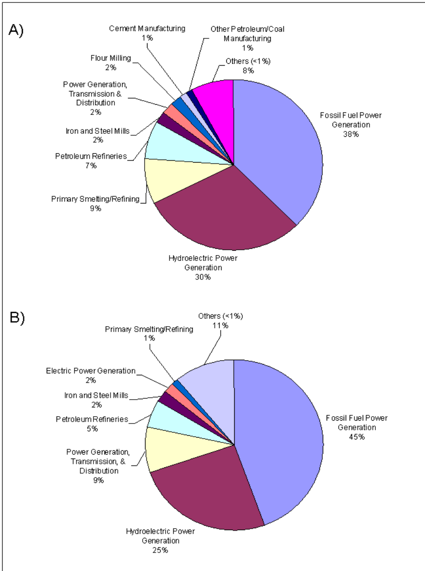
6 Figure 6-1. The percent of total SO 2 emissions by source types located within 20 7 km of ambient monitors. A) 5-minute maximum SO 2 monitors, B) 1-hour 8 SO 2 monitors. 9 10
