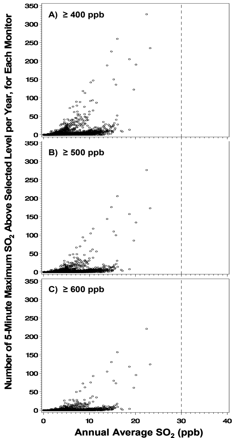
1 2 Figure 6-20. Comparison of the number of modeled 5-minute maximum SO 2 3 concentrations above potential health effect benchmark levels at each 4 monitor per year and the associated annual average SO 2 concentration, 5 Years 1997 through 2006, all 1-hour monitors. A) number of 5-minute 6 maximums ≥400 ppb/year, B) number of 5-minute maximums ≥500 7 ppb/year, C) number of 5-minute maximums ≥600 ppb/year. The level of 8 the annual average SO 2 NAAQS of 0.03 ppm is indicated by the dashed 9 line.
