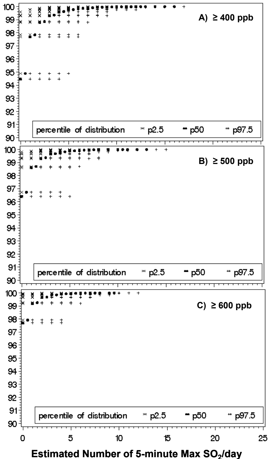
1 2 Figure 6-36. 95% prediction intervals for estimated number of 5-minute maximum 3 SO 2 concentrations per day above potential health effect benchmark 4 levels at each monitor, Years 2002 through 2006 for 20 selected counties, 5 air quality data adjusted to just meeting the current standards (either one 6 exceedance of 0.14 ppm daily average or no exceedance of 0.03 ppm 7 annual average).
