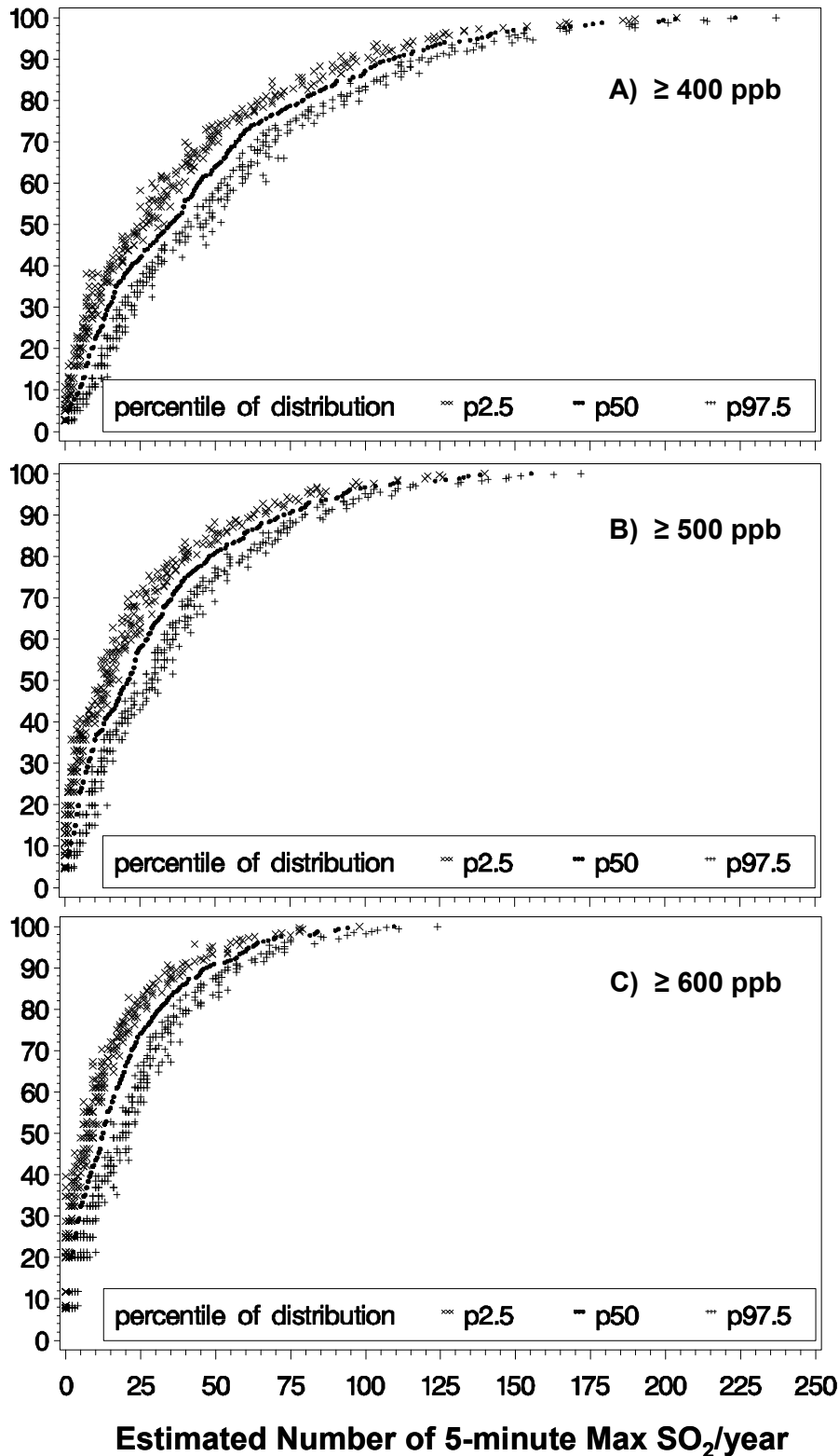
1 2 Figure 6-35. 95% prediction intervals for estimated number of 5-minute maximum 3 SO 2 concentrations in a year above potential health effect benchmark 4 levels at each monitor, Years 2002 through 2006 for 20 selected counties, 5 air quality data adjusted to just meeting the current standards (either one 6 exceedance of 0.14 ppm daily average or no exceedance of 0.03 ppm 7 annual average).
