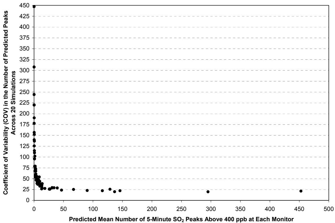
1 2 Figure 6-6. Variability in the predicted number of 5-minute maximum 3 concentrations above 400 ppb at monitors that measured 5-minute 4 maximum concentrations.
