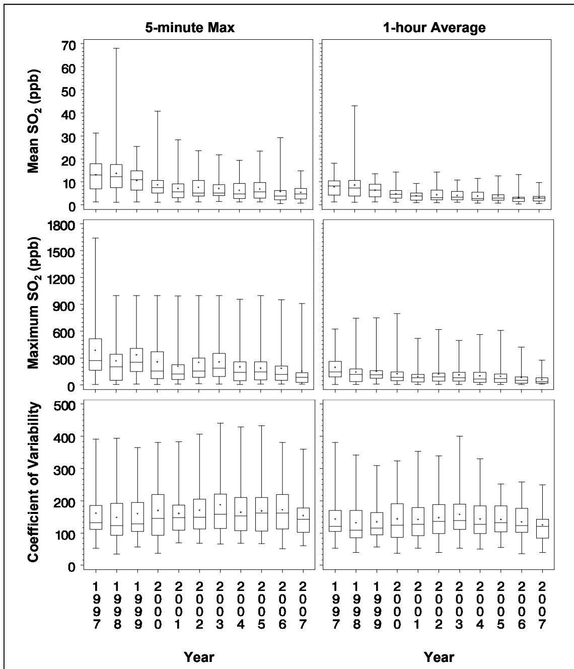
1 2 Figure 6-9. Distribution of the mean SO 2 concentrations, the maximum SO 2 3 concentrations and the coefficient of variability for each monitor that 4 measured both the 5-minute maximum and 1-hour concentrations, Years 5 1997 through 2007.
