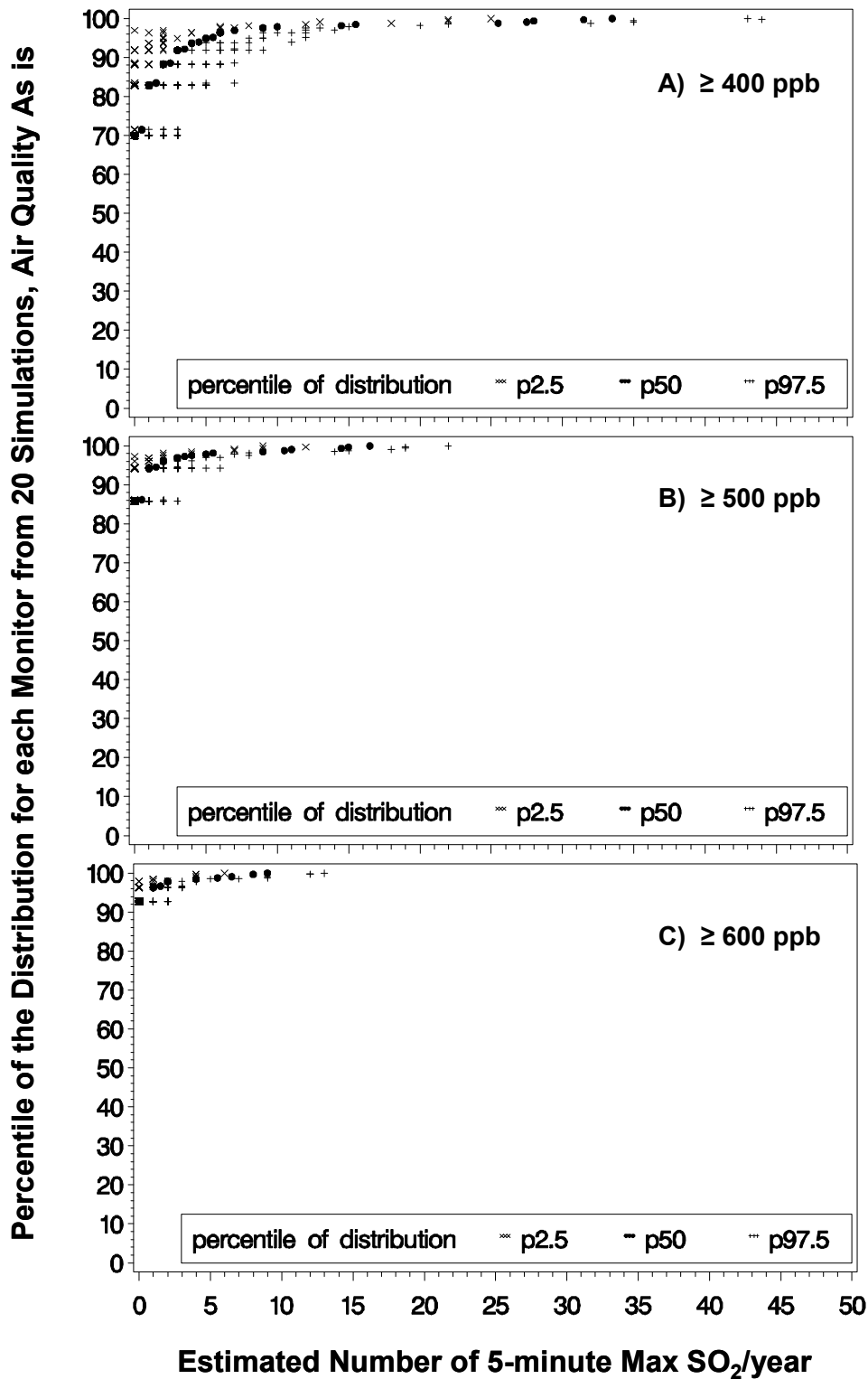
1 2 Figure 6-34. 95% prediction intervals for estimated number of 5-minute maximum 3 SO 2 concentrations in a year above potential health effect benchmark 4 levels at each monitor, Years 2002 through 2006 for 20 selected counties, 5 air quality data as is.
