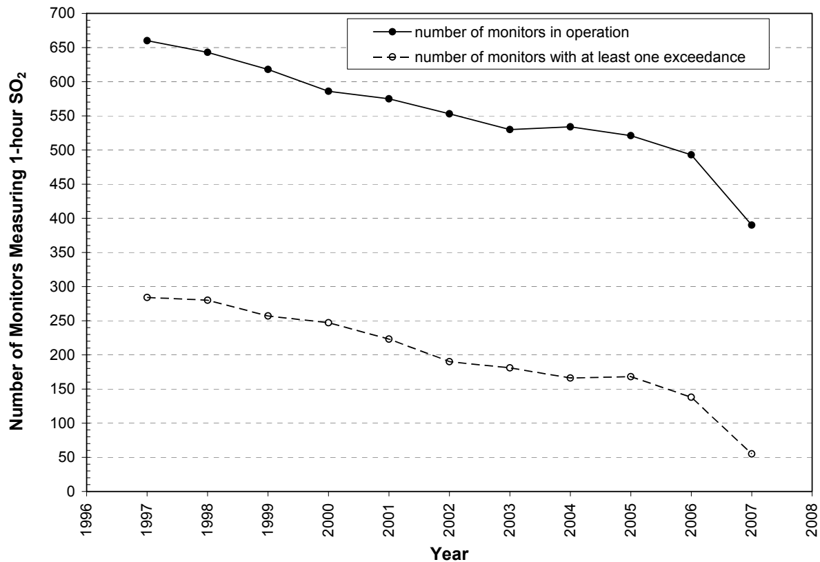
4 Figure 6-17. Number of ambient monitors measuring 1-hour average SO 2 5 concentration concentrations and number of monitors with at least one 6 benchmark exceedance by year, Years 1997 through 2007.
