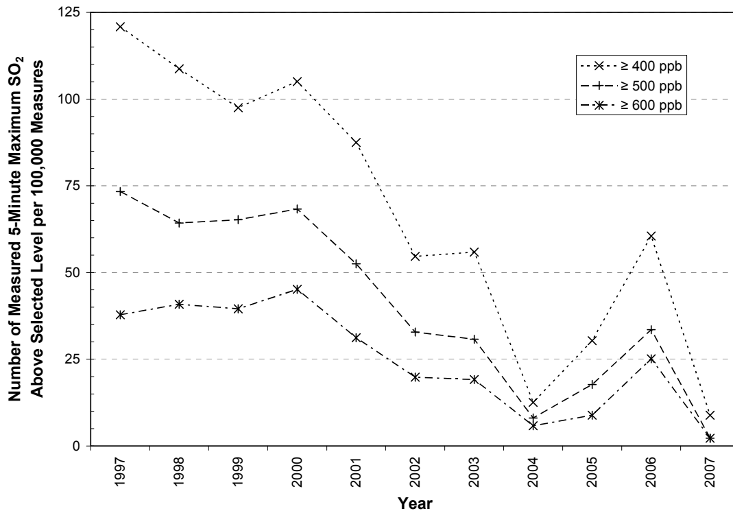
1 2 Figure 6-12. Frequency of measured 5-minute maximum SO 2 concentrations 3 above potential health effect benchmark levels in each year, normalized 4 to 100,000 measurements, Years 1997 through 2007. 5
