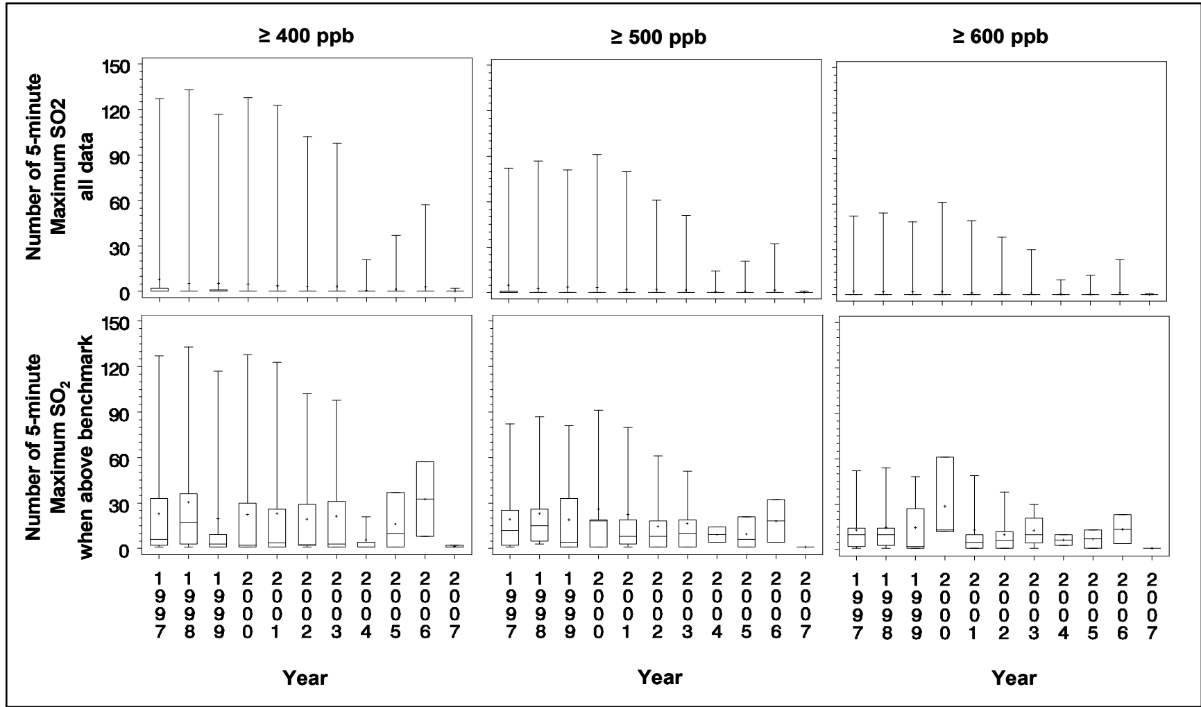
Figure 6-10. Distribution of the number of measured 5-minute maximum SO 2 concentrations above potential health effect benchmark levels at each monitor, Years 1997 through 2007. The top row represents the distribution for all monitors (including those with no exceedances), the bottom row represents the distribution for those monitors with at least one measured exceedance.
