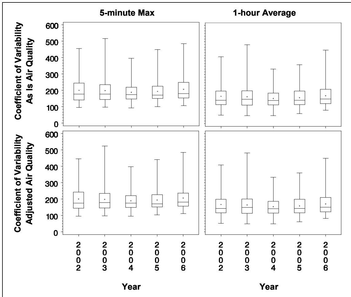
1 2 3 Figure 26. Coefficient of variability (COV, %) for modeled 5-minute maximum and 4 measured 1-hour SO 2 concentrations, Years 2002 through 2006 at 20 5 selected counties, with air quality as is and air quality adjusted to just 6 meeting the current standards (either one exceedance of 0.14 ppm daily 7 average or no exceedance of 0.03 ppm annual average). 8
