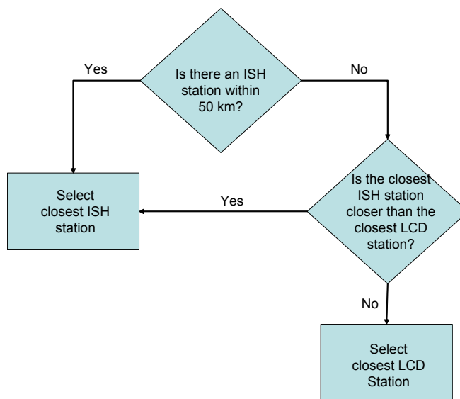
1 2 Figure 7-2. Decision tree for selection of meteorological stations. 3
