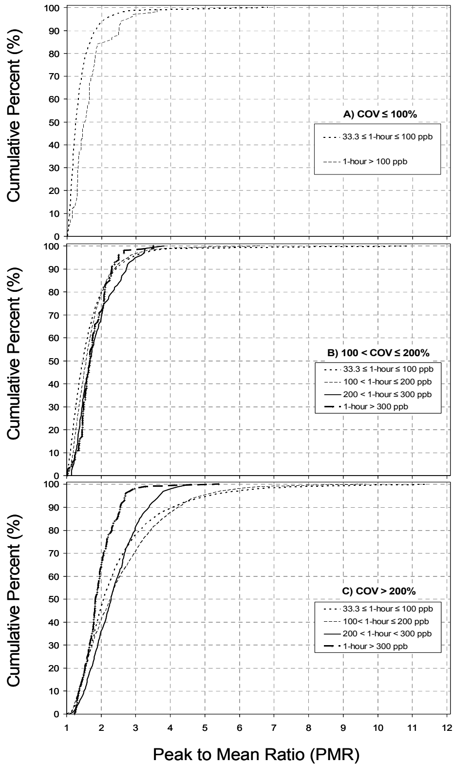
1 2 Figure 6-4. Peak to mean ratio (PMR) distributions for three variability categories 3 and 1-hour concentration groups. A) COV ≤ 100%, B) 100 < COV ≤ 200%, 4 and C) COV > 200%.
