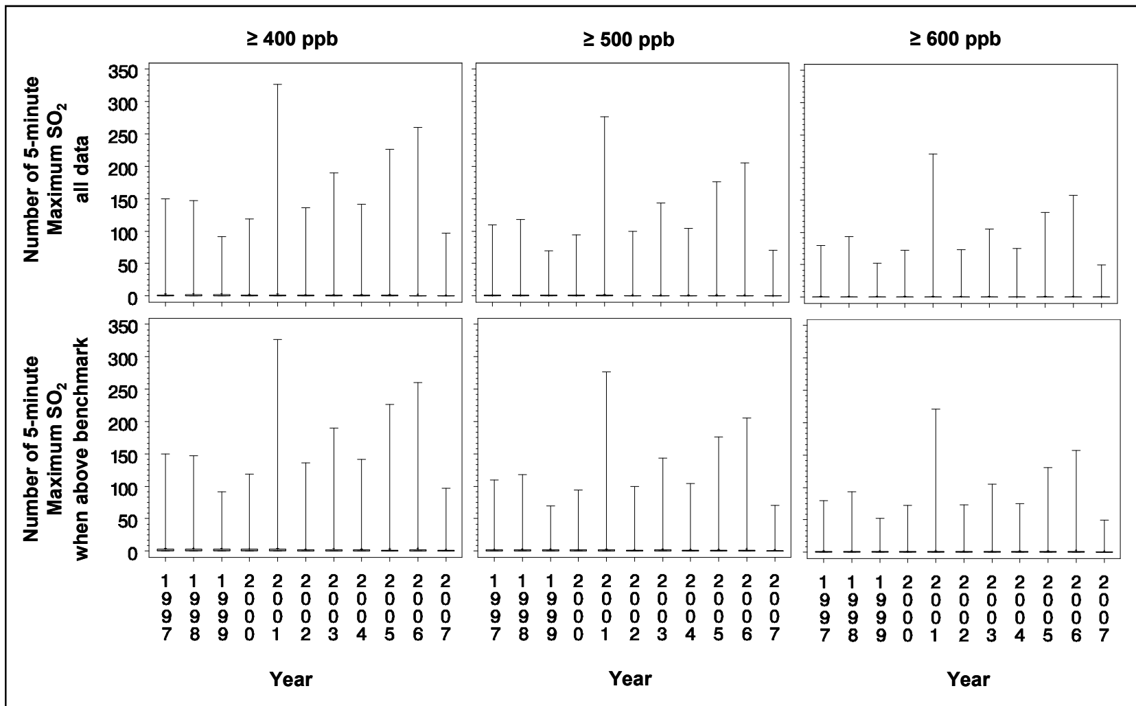
Figure 6-16. Distribution of the modeled 5-minute maximum SO 2 concentrations above potential health effect benchmark levels at each monitor by year, Years 1997 through 2007. The top row represents the distribution for all monitors (including those with no exceedances), the bottom row represents the distribution for those monitors with at least one estimated exceedance.
