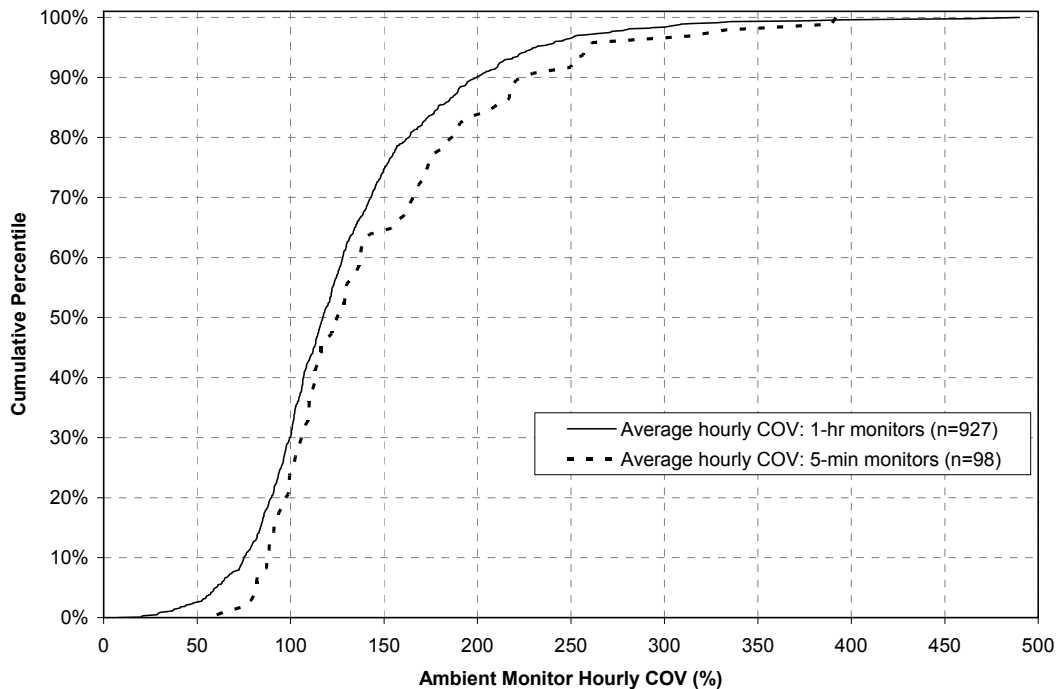
1 2 Figure 6-3. Cumulative density functions (CDFs) for hourly COV at 1-hour and 5- 3 minute SO 2 monitors. 4
