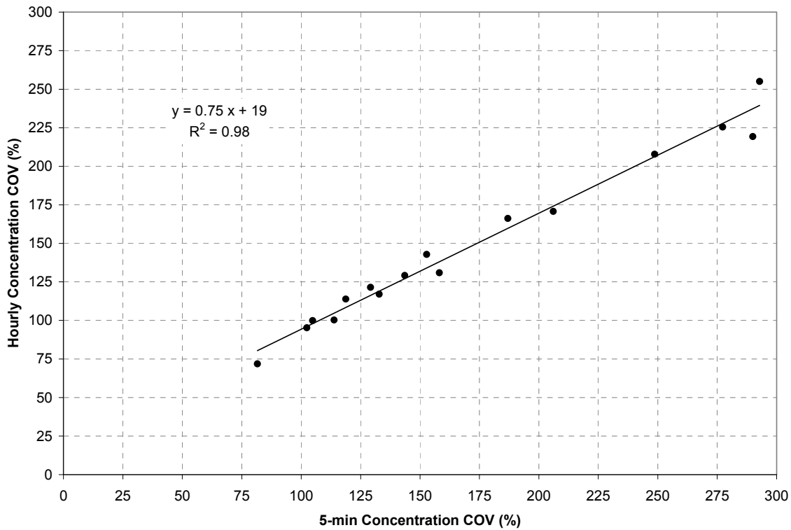
7 8 Figure 6-2. Comparison of hourly COV and 5-minute COV at 16 continuous-5 9 monitors, over multiple years of monitoring. 10
