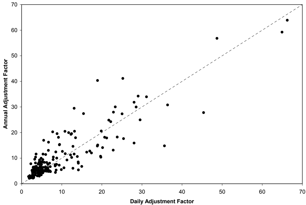
1 2 Figure 6-8. Comparison of annual and daily adjustment factors derived from 3 counties containing at least three 1-hour ambient SO 2 monitors with 4 valid data, years 2002 through 2006. 5
