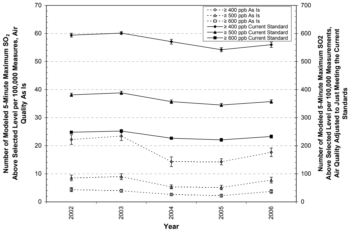
7 8 9 Figure 6-27. Frequency of modeled 5-minute maximum SO 2 concentrations above 10 potential health effect benchmark levels in each year, normalized to 11 100,000 measurements, Years 2002 through 2006 at twenty selected 12 counties, with air quality as is and air quality adjusted to just meeting the 13 current standards (either one exceedance of 0.14 ppm daily average or 14 no exceedance of 0.03 ppm annual average). Bars indicate standard 15 deviation of the mean from the twenty model simulations.
