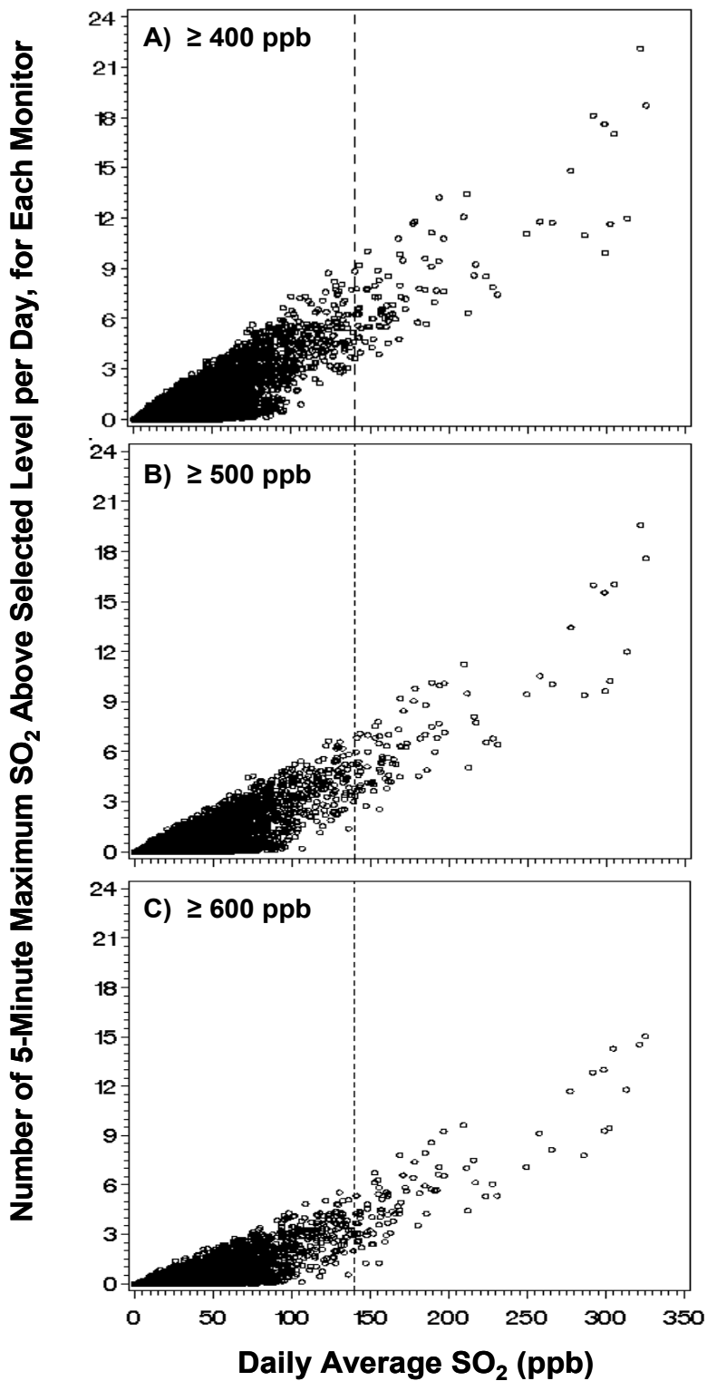
1 2 Figure 6-22. Comparison of the number of modeled 5-minute maximum SO 2 3 concentrations above potential health effect benchmark levels at each 4 monitor per day and the associated daily average SO 2 concentration, 5 Years 1997 through 2007, all 1-hour SO 2 monitors. The level of the 24- 6 hour SO 2 NAAQS of 0.14 ppm is indicated by the dashed line.
