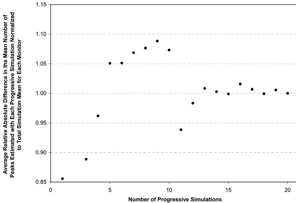
4 5 Figure 6-5. Comparison of the mean relative absolute difference in number of 6 predicted and measured peaks above 400 ppb, across progressive 7 model simulations using the monitors that contained measurements for 8 5-minute maximum SO 2 concentrations.
