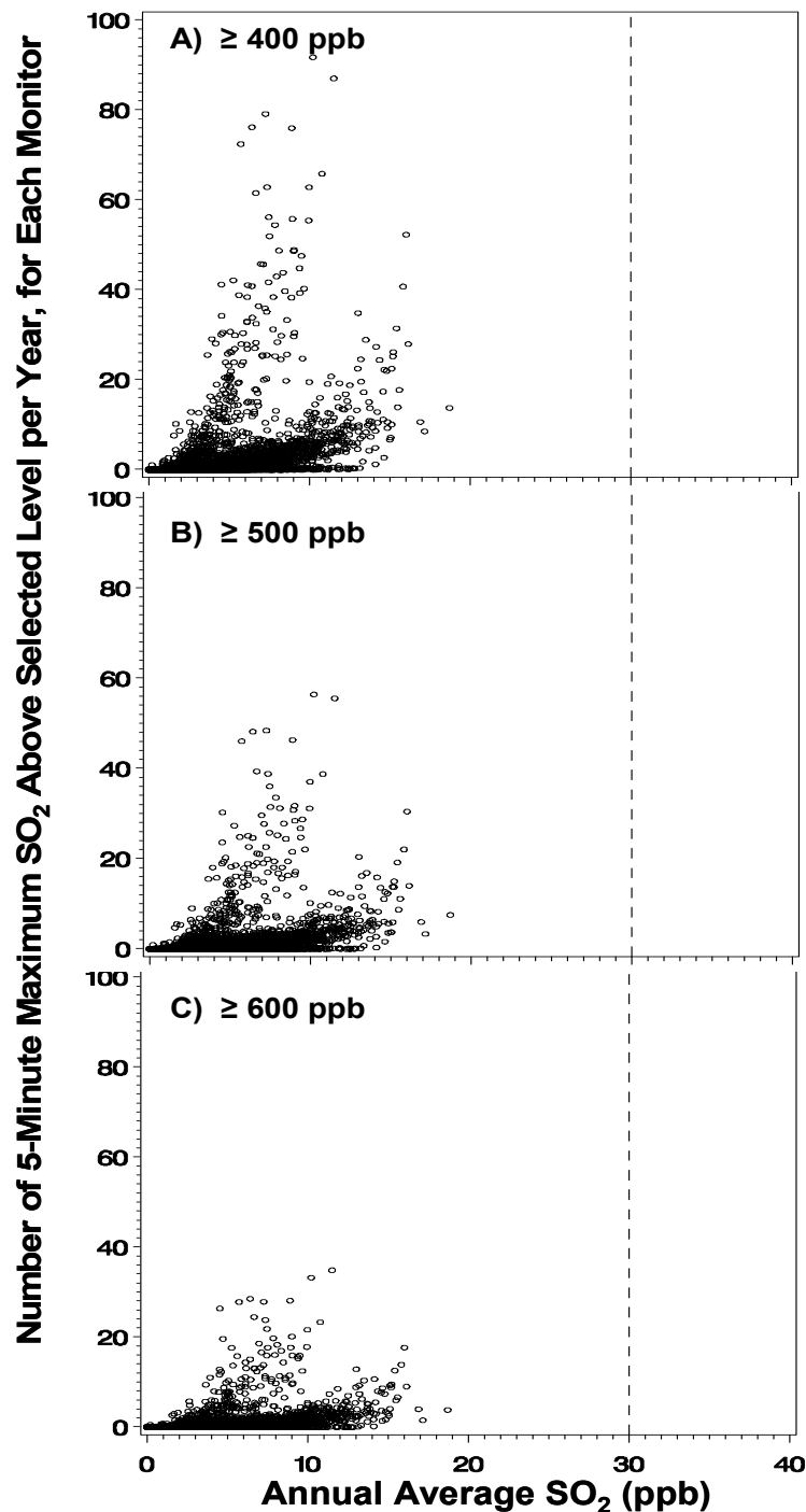
1 2 Figure 6-21. Comparison of the number of modeled 5-minute maximum SO 2 3 concentrations above potential health effect benchmark levels at each 4 monitor per year and the associated annual average SO 2 concentration, 5 Years 1997 through 2006, without Hawaii and Caribou Counties (2001 6 only). A) number of 5-minute maximums ≥400 ppb/year, B) number of 5- 7 minute maximums ≥500 ppb/year, C) number of 5-minute maximums 8 ≥600 ppb/year. The level of the annual average SO 2 NAAQS of 0.03 ppm 9 is indicated by the dashed line.
