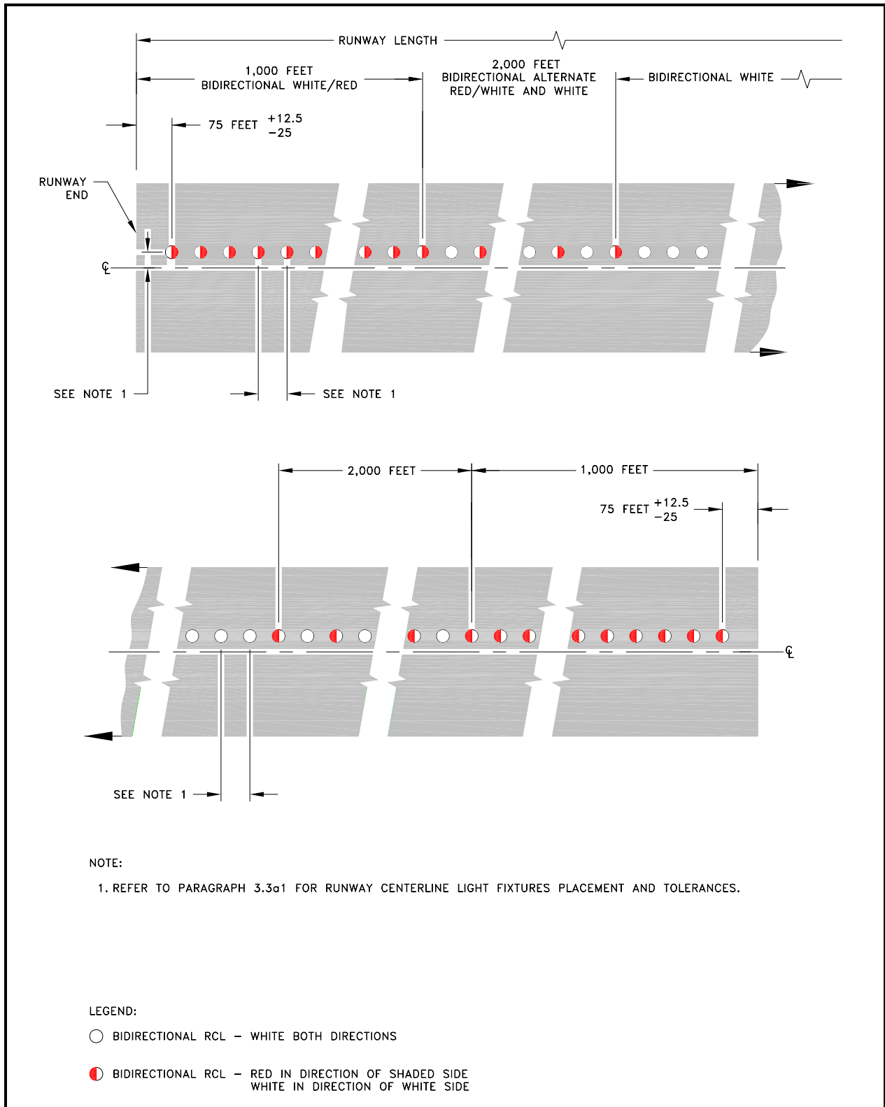
Figure 33. Runway Centerline Lighting Layout.
