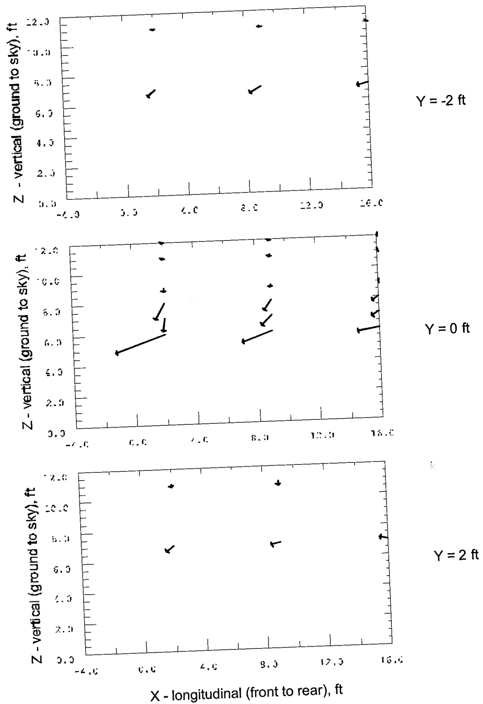
Figure 4.27. Vehicle wake flow vectors, cross-section view at y = -2 ft ( -0.61 m), y = 0 ft ( 0 m), y = 2 ft ( 0.61 m), respectively, from centerline, speed = 30 mph ( 13.4 m/s), looking from side, vehicle width = 6.2 ft ( 1.9 m), height = 6.9 ft ( 2.1 m), scale for vectors on plots: 1 unit = 2 m/s.
