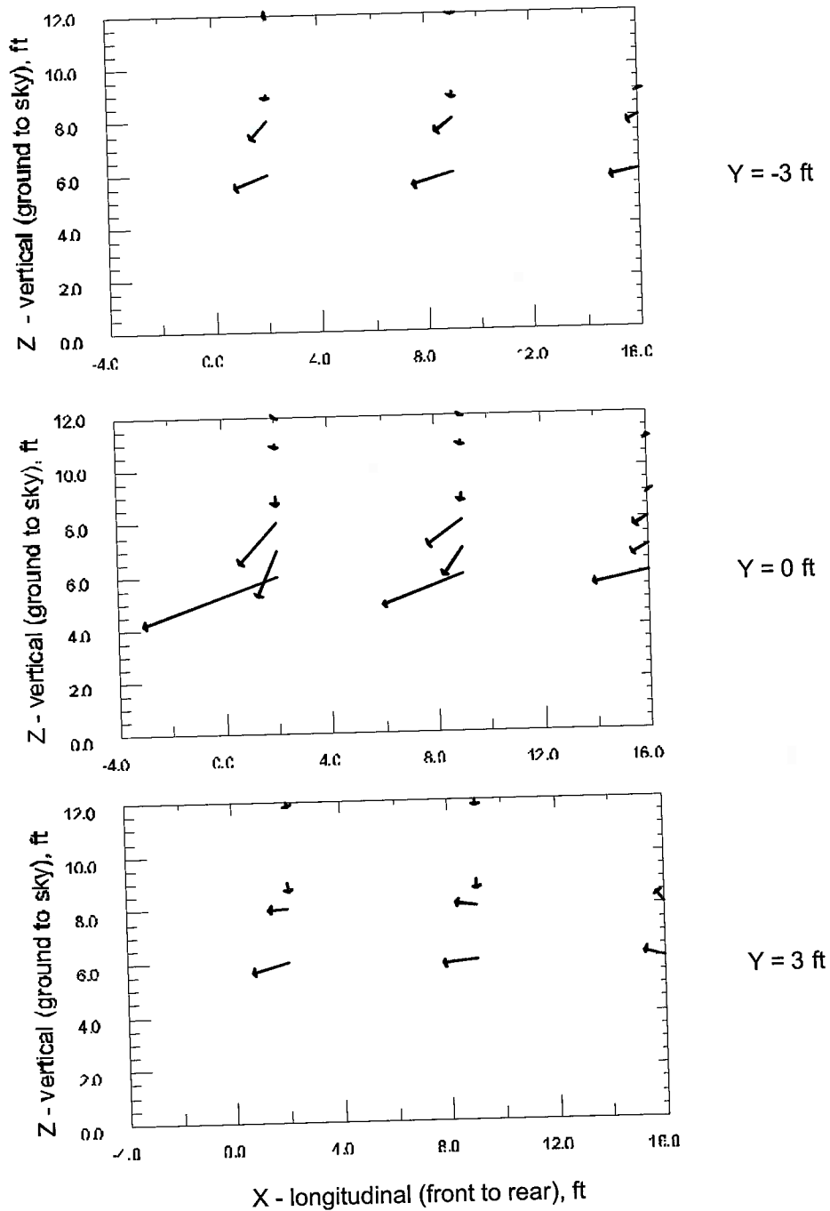
Figure 4.30. Vehicle wake flow vectors, cross-section view at y = -3 ft (-0.91 m), y = 0 ft (0 m), y = 3 ft (0.91 m), respectively, from centerline, speed = 50 mph (22.4 m/s), looking from side, vehicle width = 6.2 ft (1.9 m), height = 6.9 ft (2.1 m), scale for vectors on plots: 1 unit = 2 m/s.
