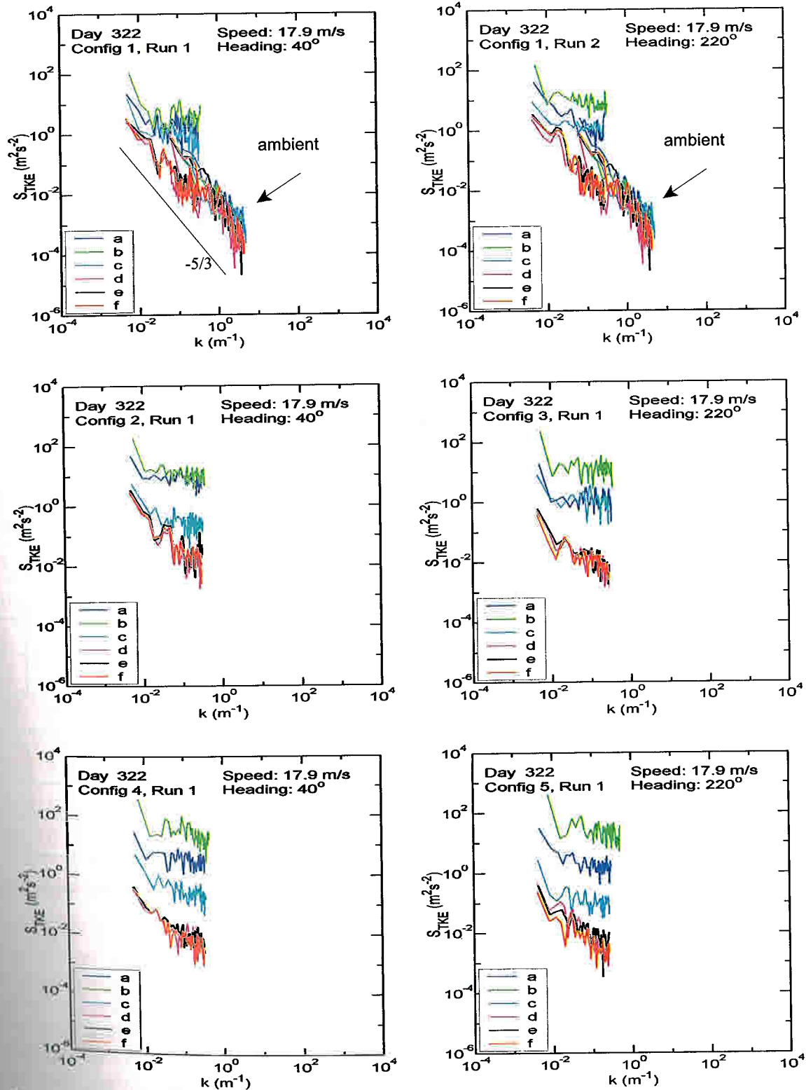
Figure 4.2 Power spectral density of TKE for Day 322, Configurations 1-5. The inertial subrange slope is shown on Configuration 1, Run 1. Ambient data are with Configuration 1.
