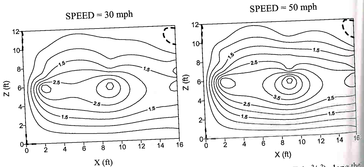
Figure 4.15 Contours in vertical-along-axis plane of constant values of TKE ( \text{m}^2/\text{s}^2 ) along the wake centerline, for vehicle speeds of 30(13.4 \text{ m/s}) and 50 \text{ mph}(22.3 \text{ m/s}) .
