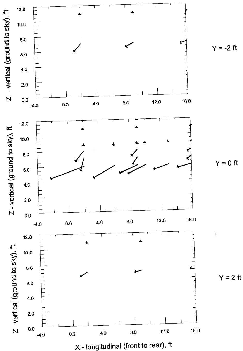
Figure 4.29. Vehicle wake flow vectors, cross-section view at y = -2 ft ( -0.61 m), y = 0 ft ( 0 m), y = 2 ft ( 0.61 m), respectively, from centerline, speed = 40 mph ( 17.9 m/s), looking from side, vehicle width = 6.2 ft ( 1.9 m), height = 6.9 ft ( 2.1 m), scale for vectors on plots: 1 unit = 2 m/s.
