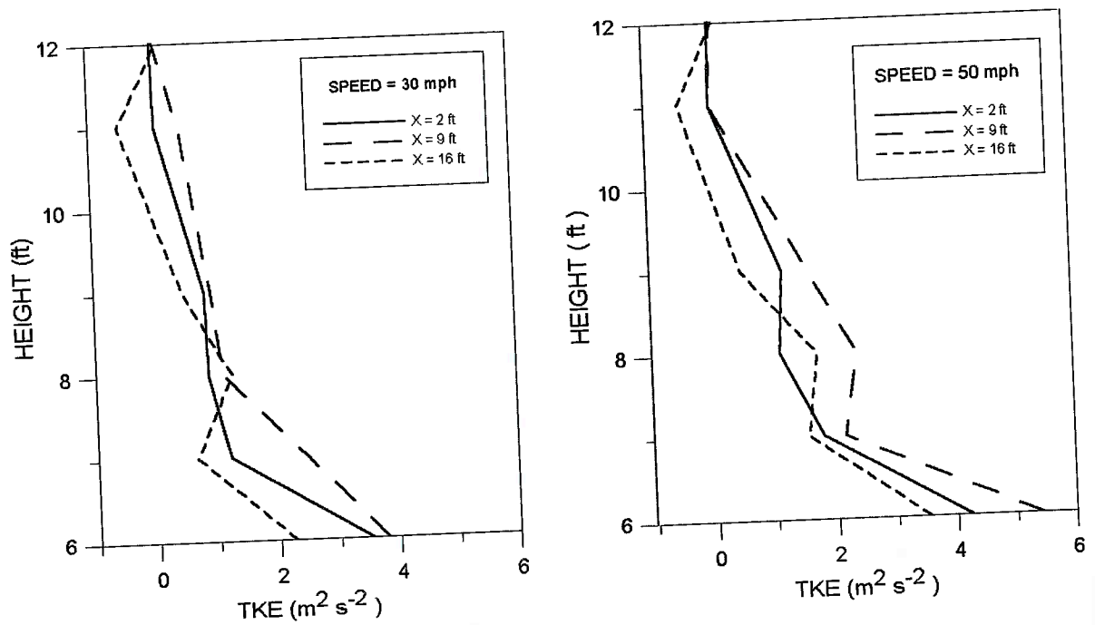
Figure 4.14 Vertical profiles of turbulent kinetic energy (TKE) in near-wake of vehicle ( x = 2, 9, and 16 ft from rear of vehicle for road speeds of 30 and 50 mph.
