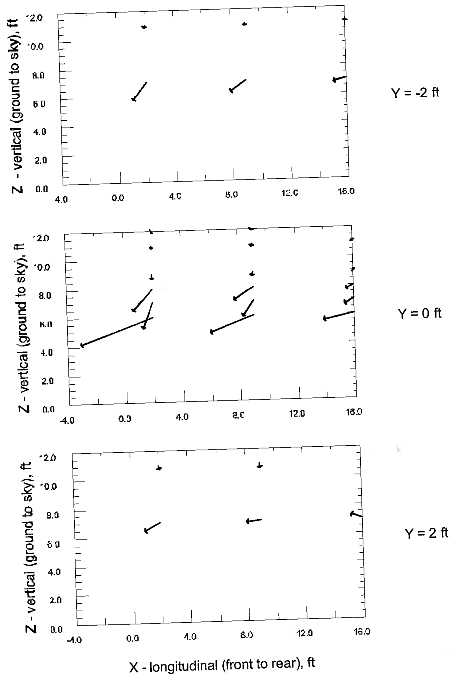
Figure 4.31. Vehicle wake flow vectors, cross-section view at y = -2 ft ( -0.61 m), y = 0 ft ( 0 m), y = 2 ft ( 0.61 m), respectively, from centerline, speed = 50 mph ( 22.4 m/s), looking from side, vehicle width = 6.2 ft ( 1.9 m), height = 6.9 ft ( 2.1 m), scale for vectors on plots: 1 unit = 2 m/s.
