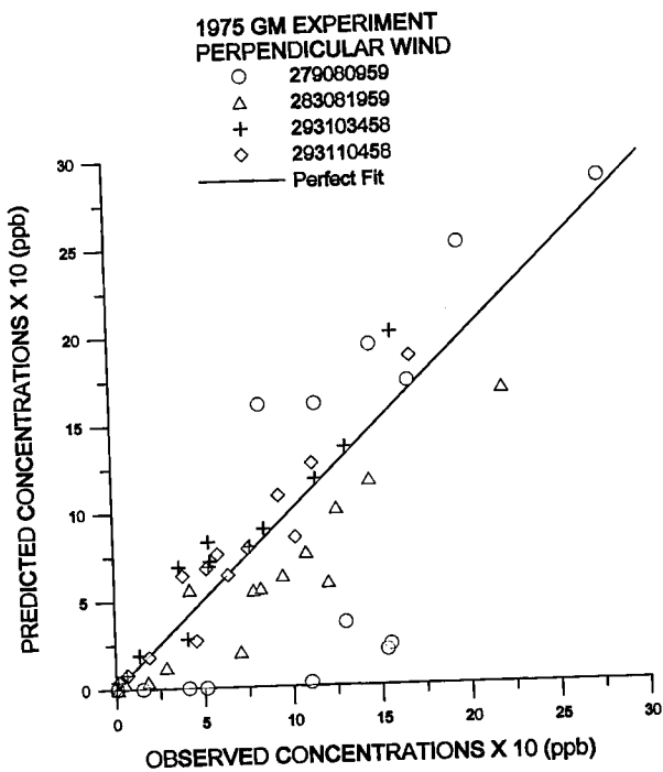
Figure 5.4 Comparison of predicted and observed concentrations for perpendicular winds.
