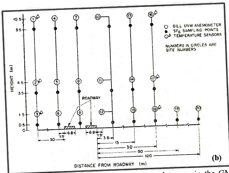
Figure 5.2 (a) Layout plan of instrumented towers in the GM experiment in relation to the traffic lanes; (b) Elevation view of meteorological towers and instrument locations.
