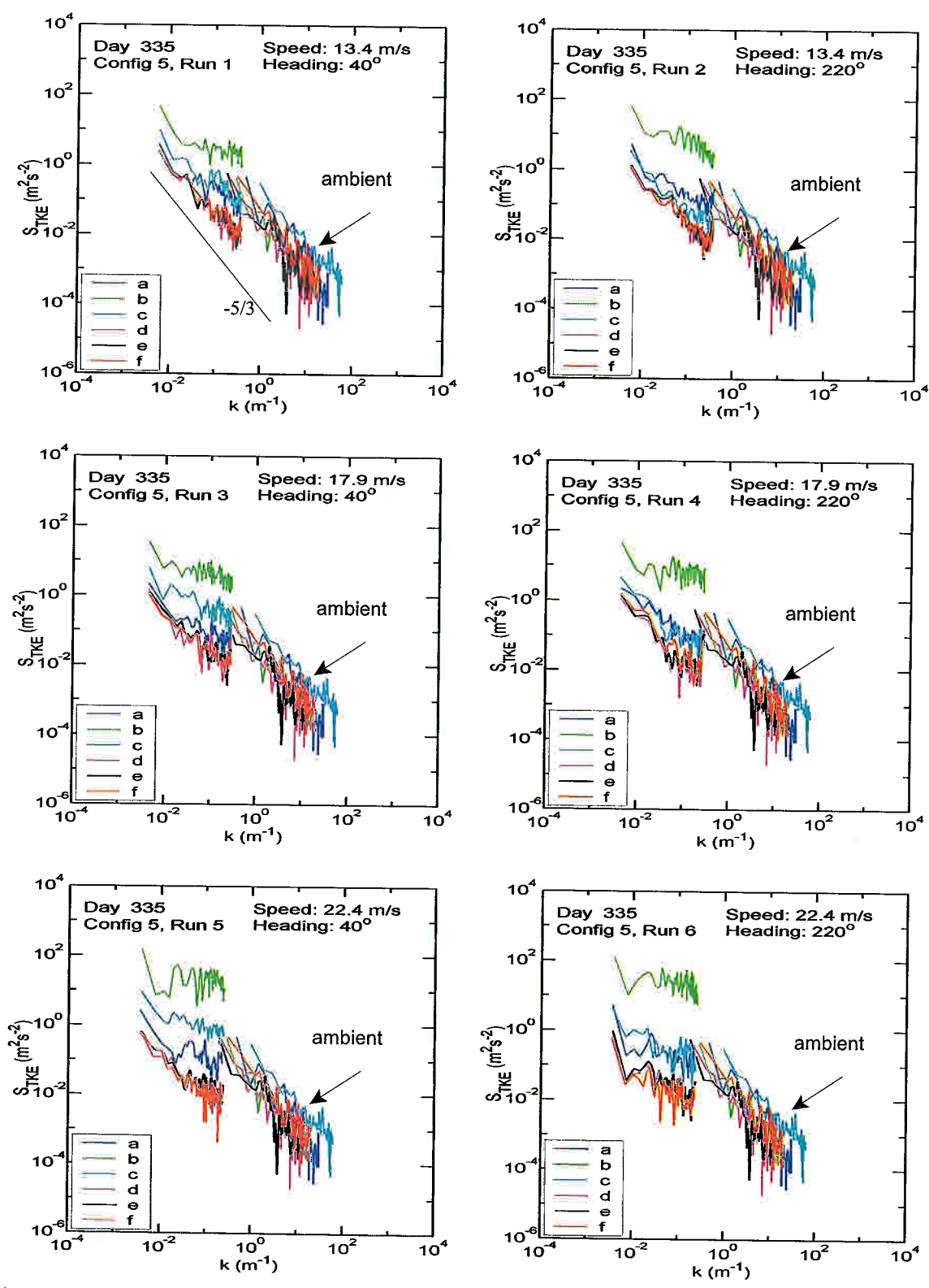
Figure 4.7 Power spectral density of TKE for Day 335, Configuration 5. The inertial subrange slope is shown on Run 1. Ambient data are with each run.
