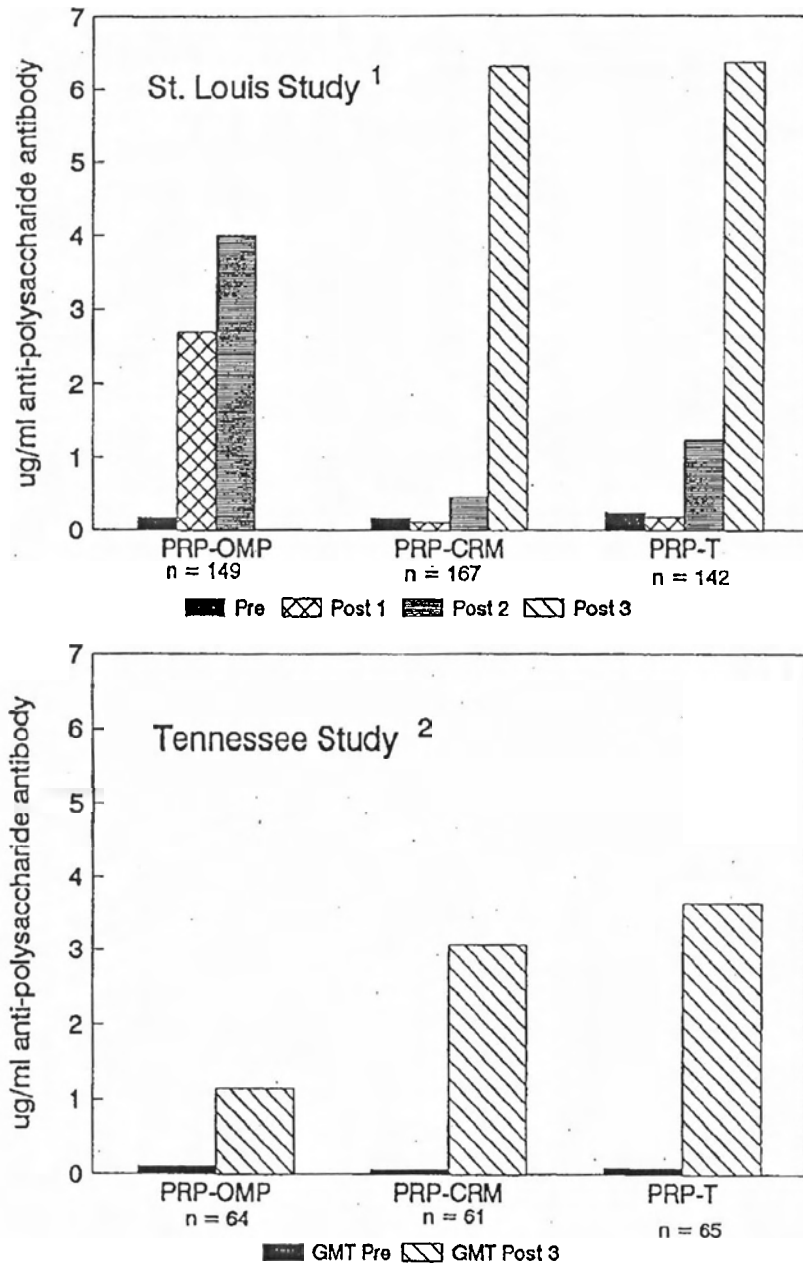
Figure 1. Comparative antibody responses to three different Haemophilus b conjugate vaccines
