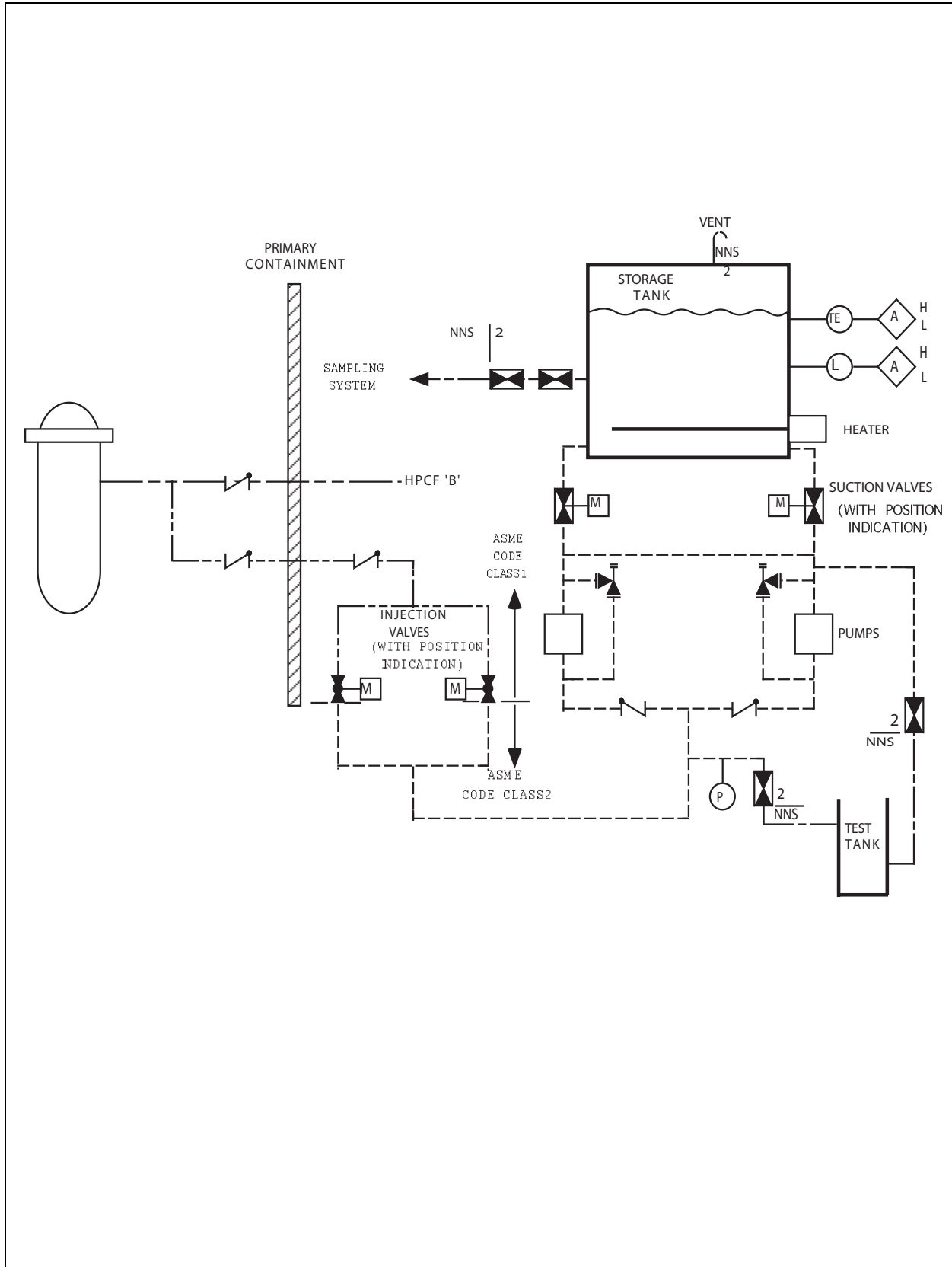
Figure 17.3-7 Standby Liquid Control System (Standby Mode)
