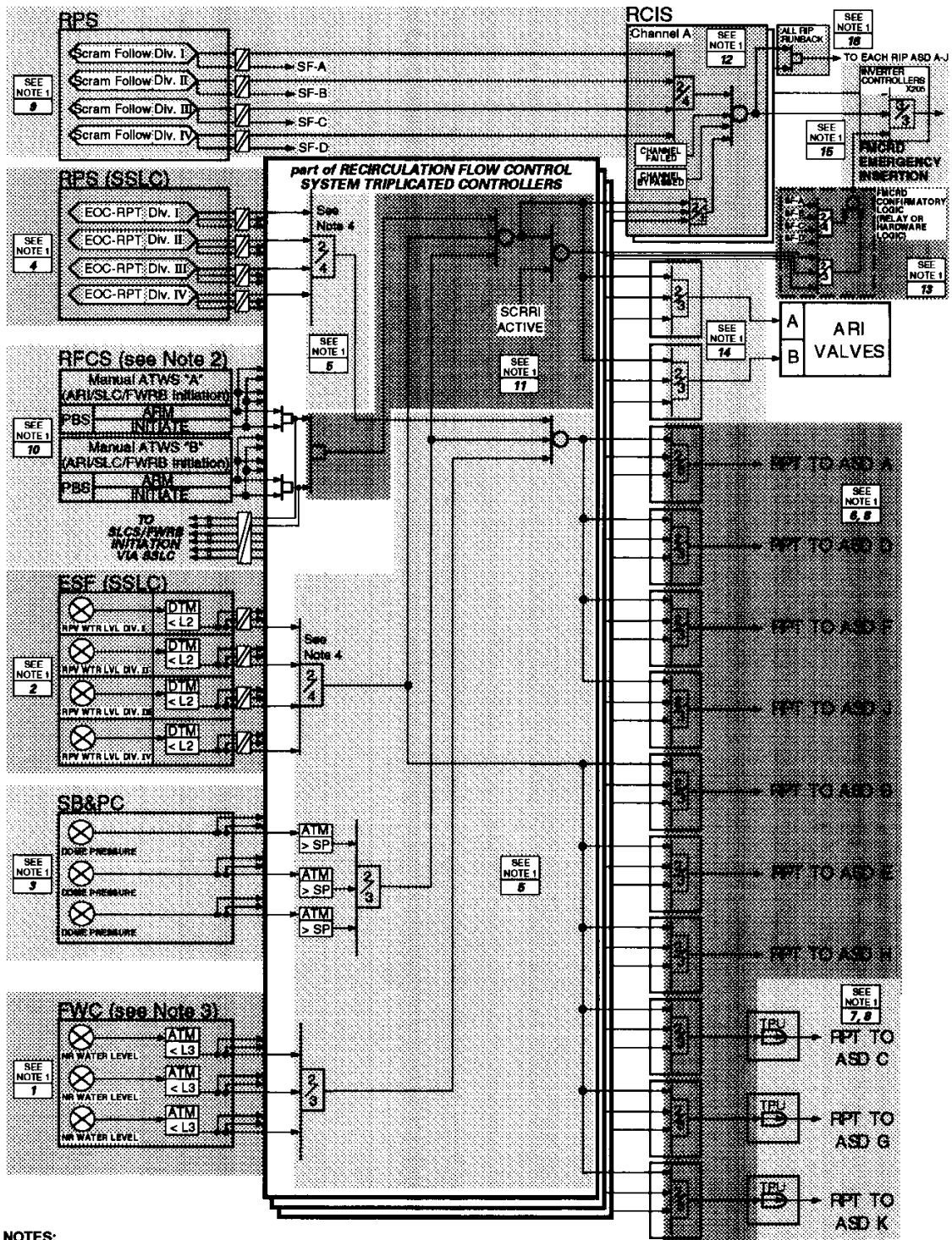
FIGURE B 3.3.4.1-1 ATWS and EOC-RPT INSTRUMENTATION CHANNELS
