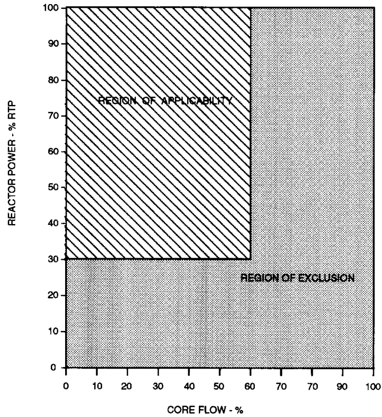
FIGURE 3.3.1.1-1: Oscillation Power Range Function Conditions of Operability
