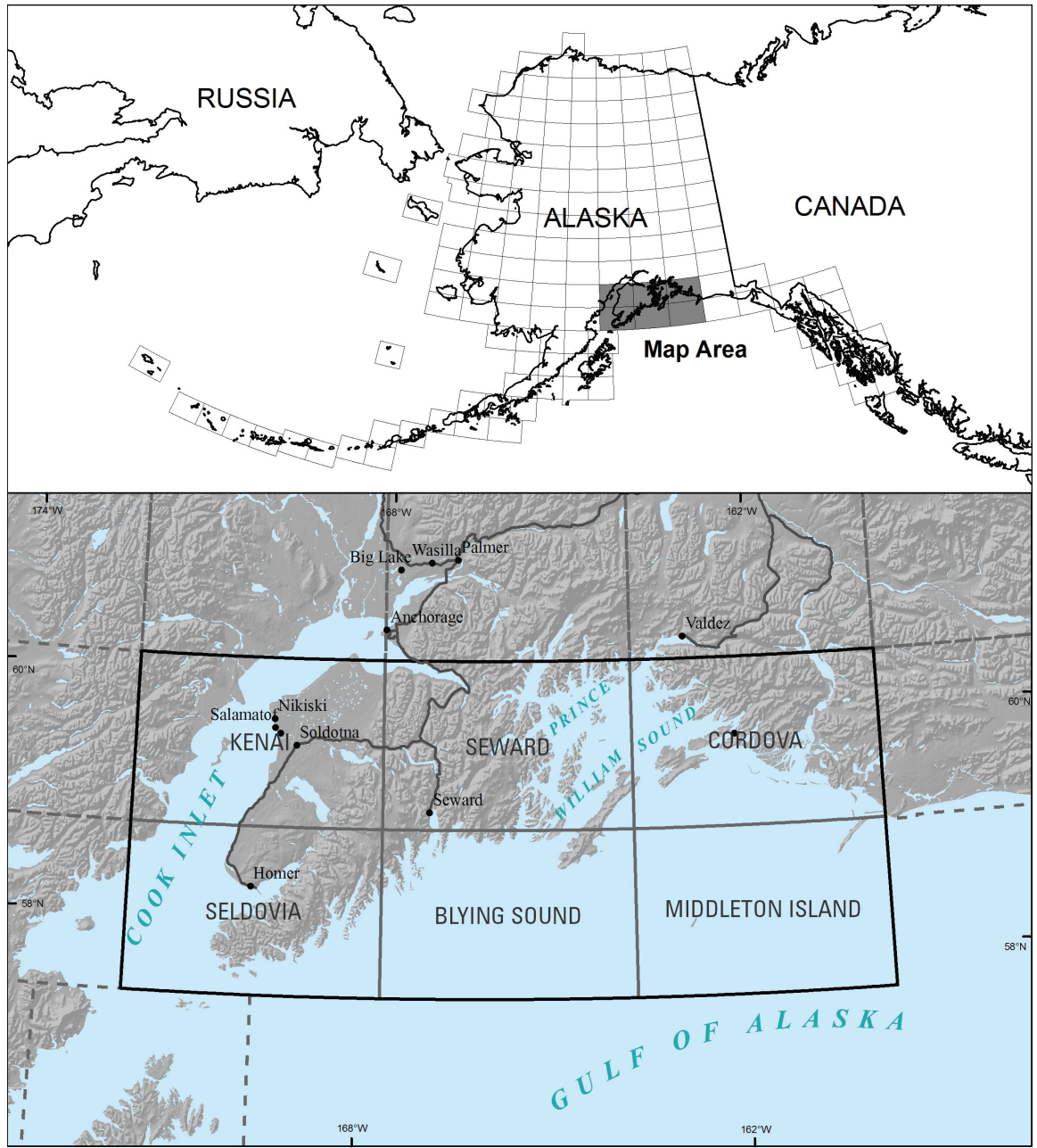
Figure 1. Location of the reconnaissance geologic map of the Prince William Sound region showing the geographic setting and included 1:250,000 quadrangles.
