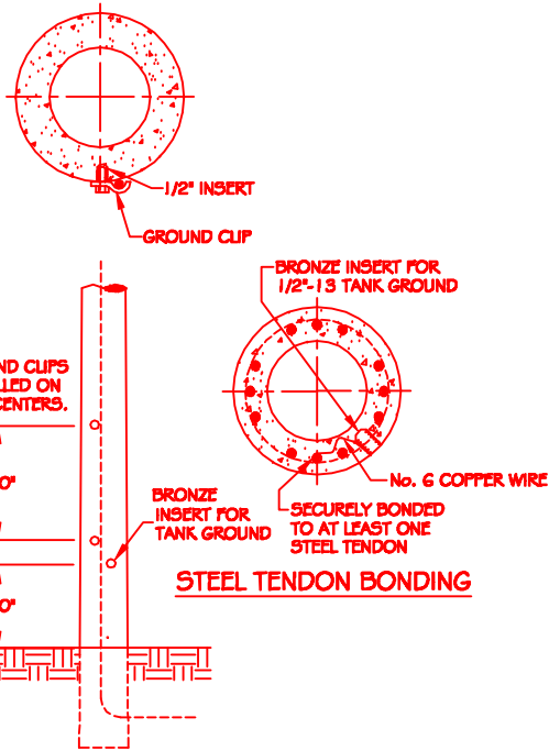
TYPICAL EXTERNAL GROUNDING
