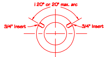
STEPBOLT DETAILS
