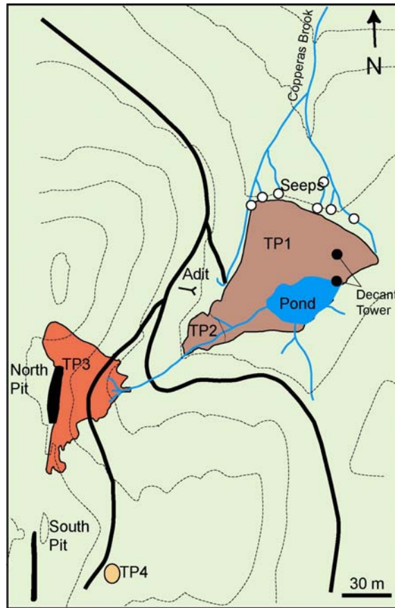
Figure 2. Elizabeth mine site map showing locations of historic mine waste pile TP3 and flotation tailings piles TP1 and TP2. Surface runoff from TP3 flows downhill through a breach in TP2 to a pond on TP1. Pond water flows down through a decant system that discharges at the northeastern corner of TP1, where it joins seeps and surface runoff to form the main channel of Copperas Brook.
