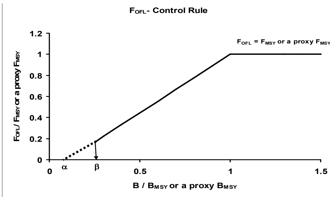
Figure 2-2 Proposed control rule for overfishing for Tiers 1 through 4 under Alternatives 2 and 3. Directed fishing mortality is 0 below \beta .
