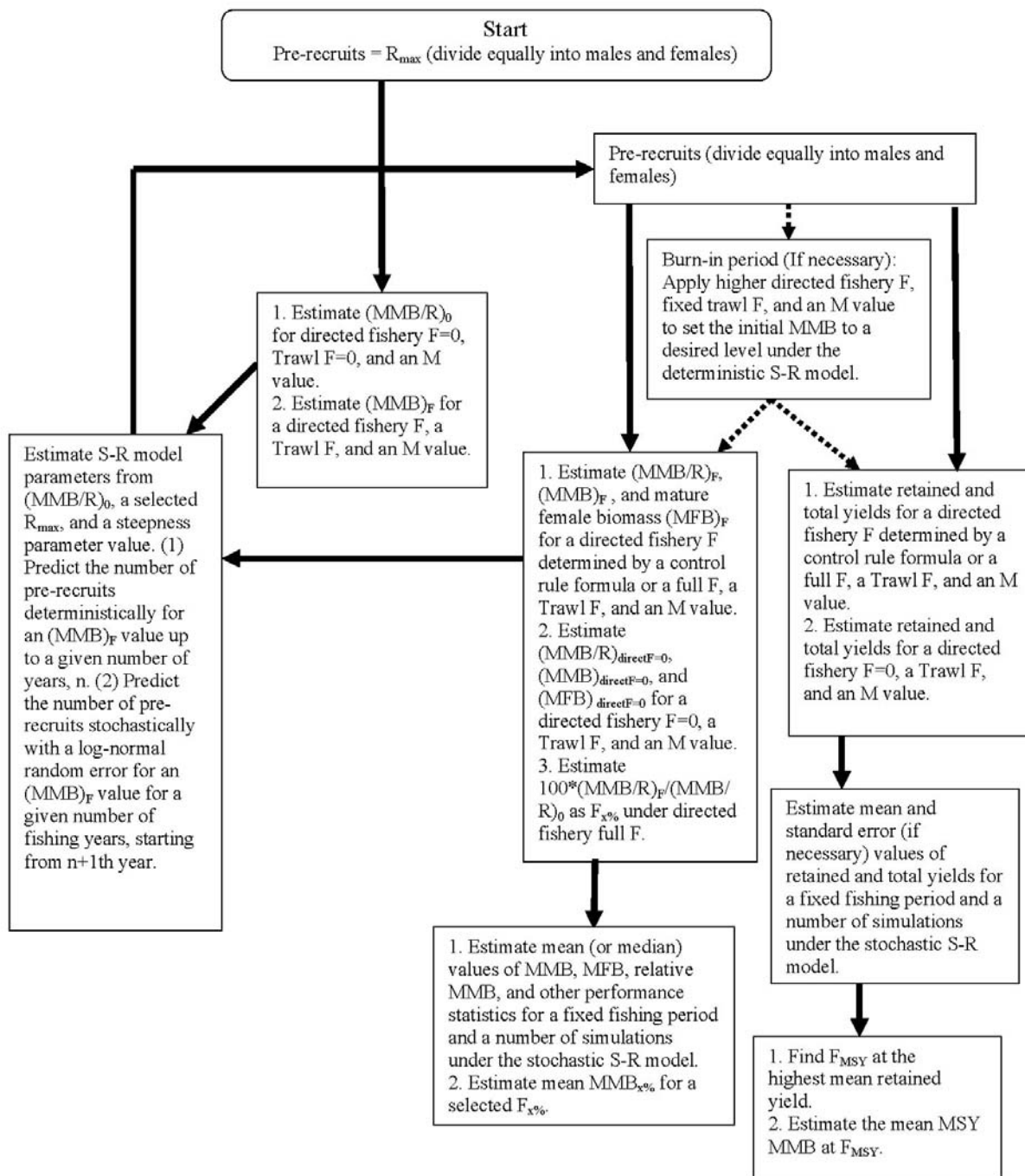
Figure 3-1 Schematic of model simulation.
