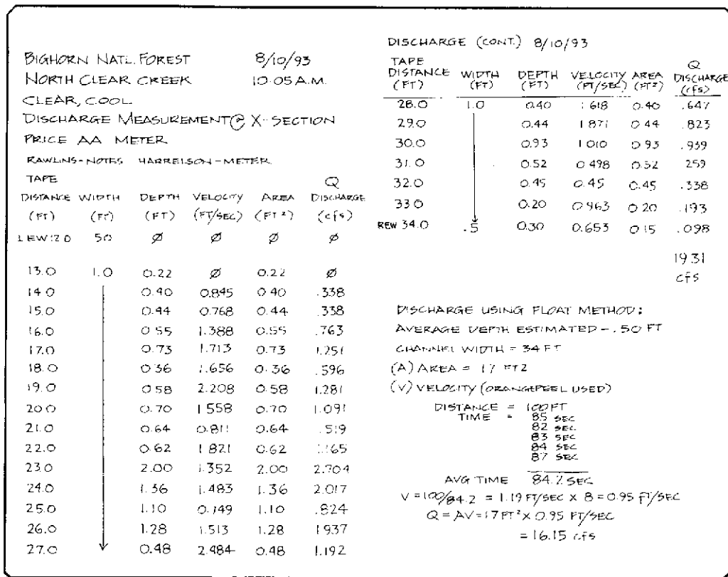
Figure 58. Field notes of discharge measurement.
