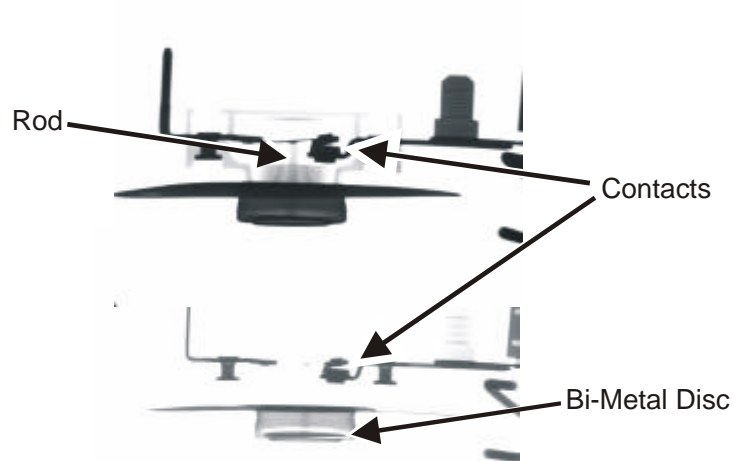
Figure 106. X-ray Images of High-Limit Thermostat 2 (HLT2)
