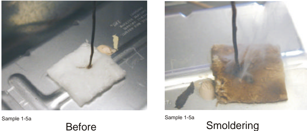
Figure 55. Sample Smoldering at Location A
