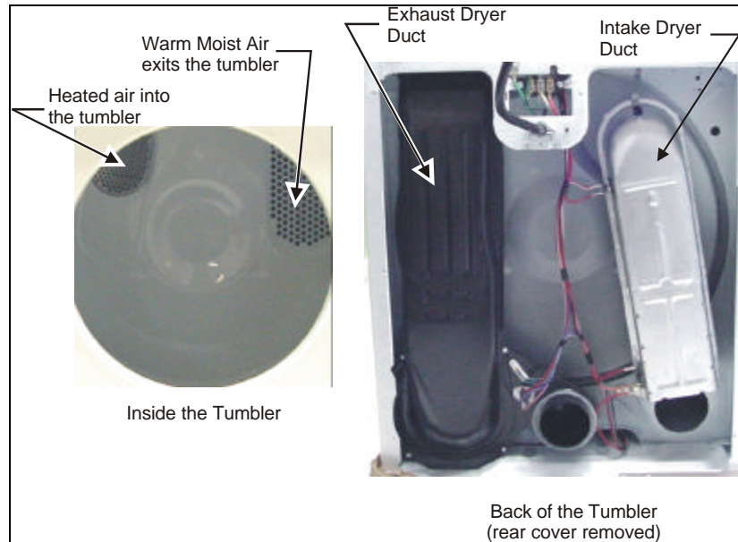
Figure 8. Dryer Design A Intake and Exhaust
