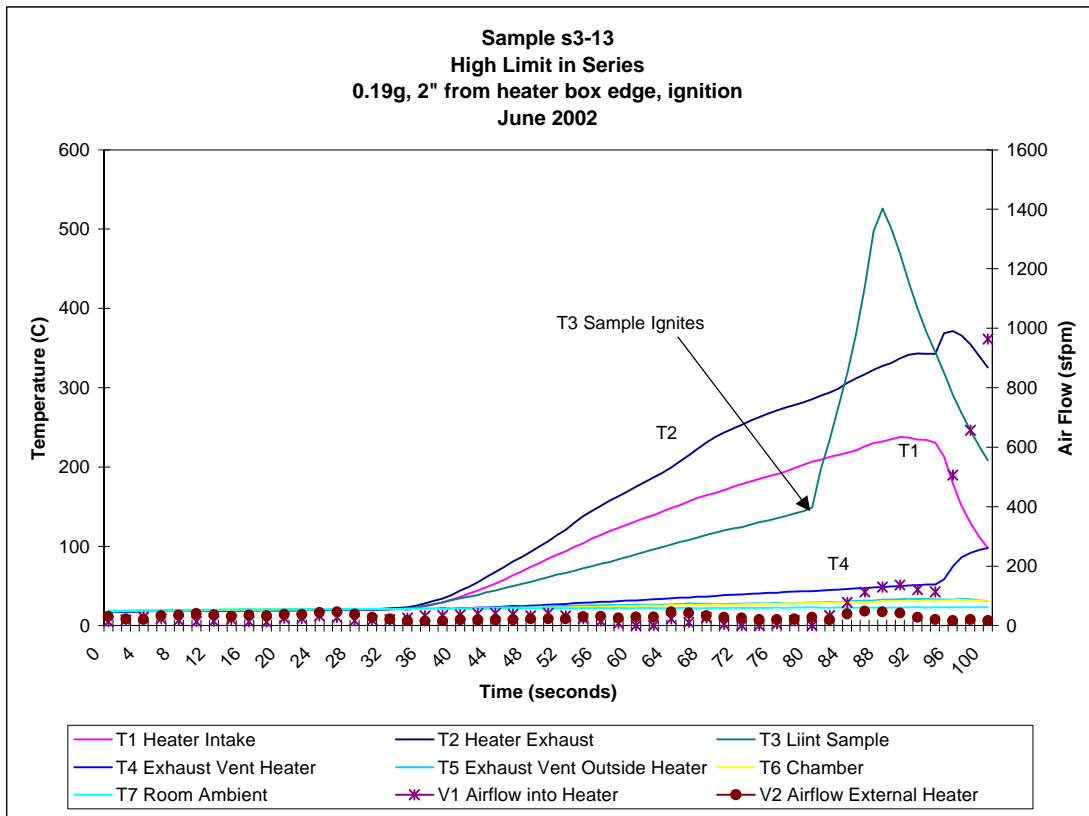
Figure 99. Sample s3-13 Test with the High Limit Thermostat in Series
