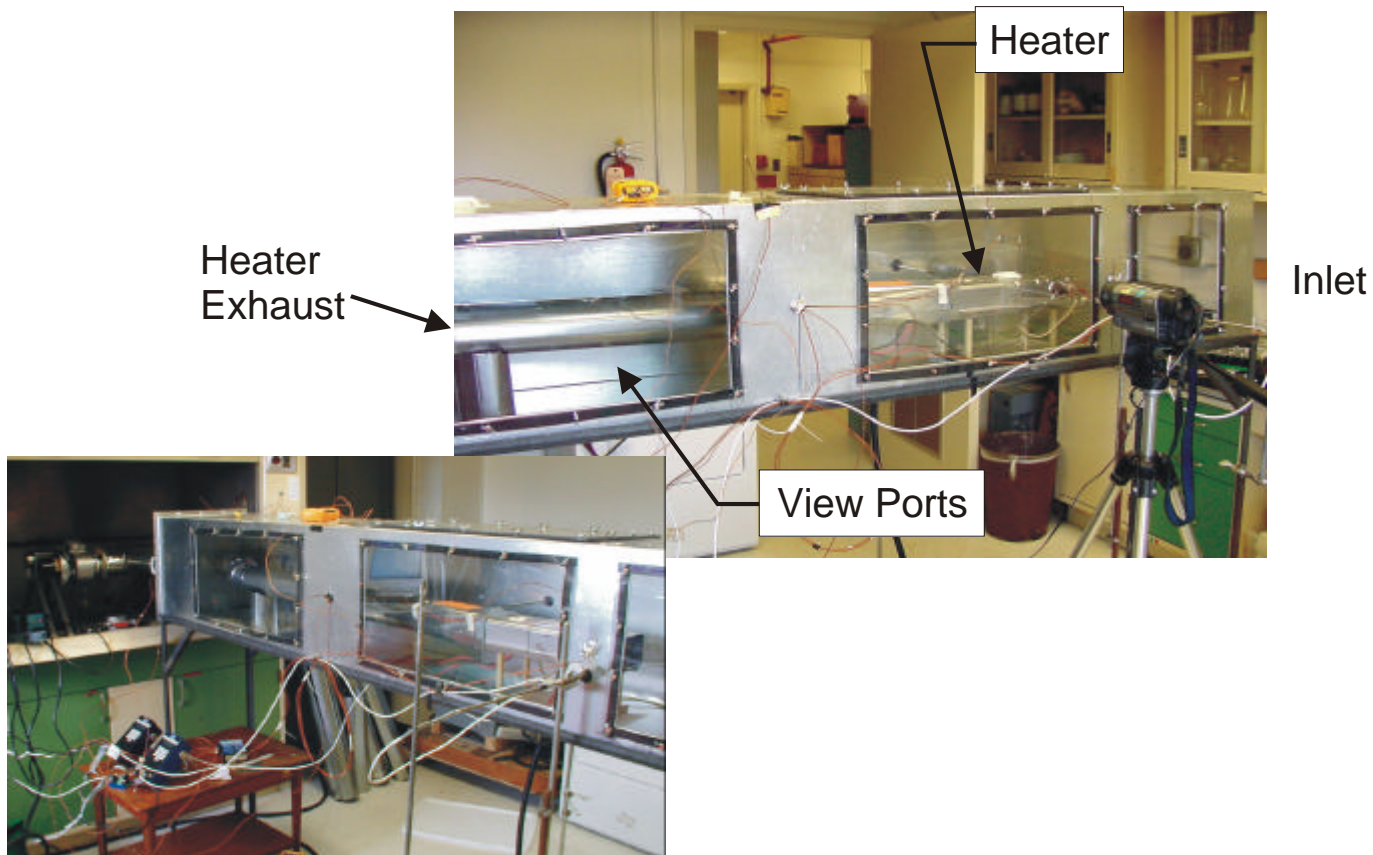
Figure 51. Test Setup for Lint Ignition
