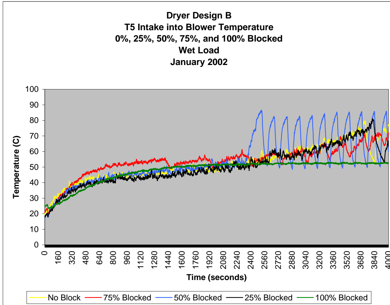
Figure 22. Dryer Design B – T5 Intake into the Blower Comparison
