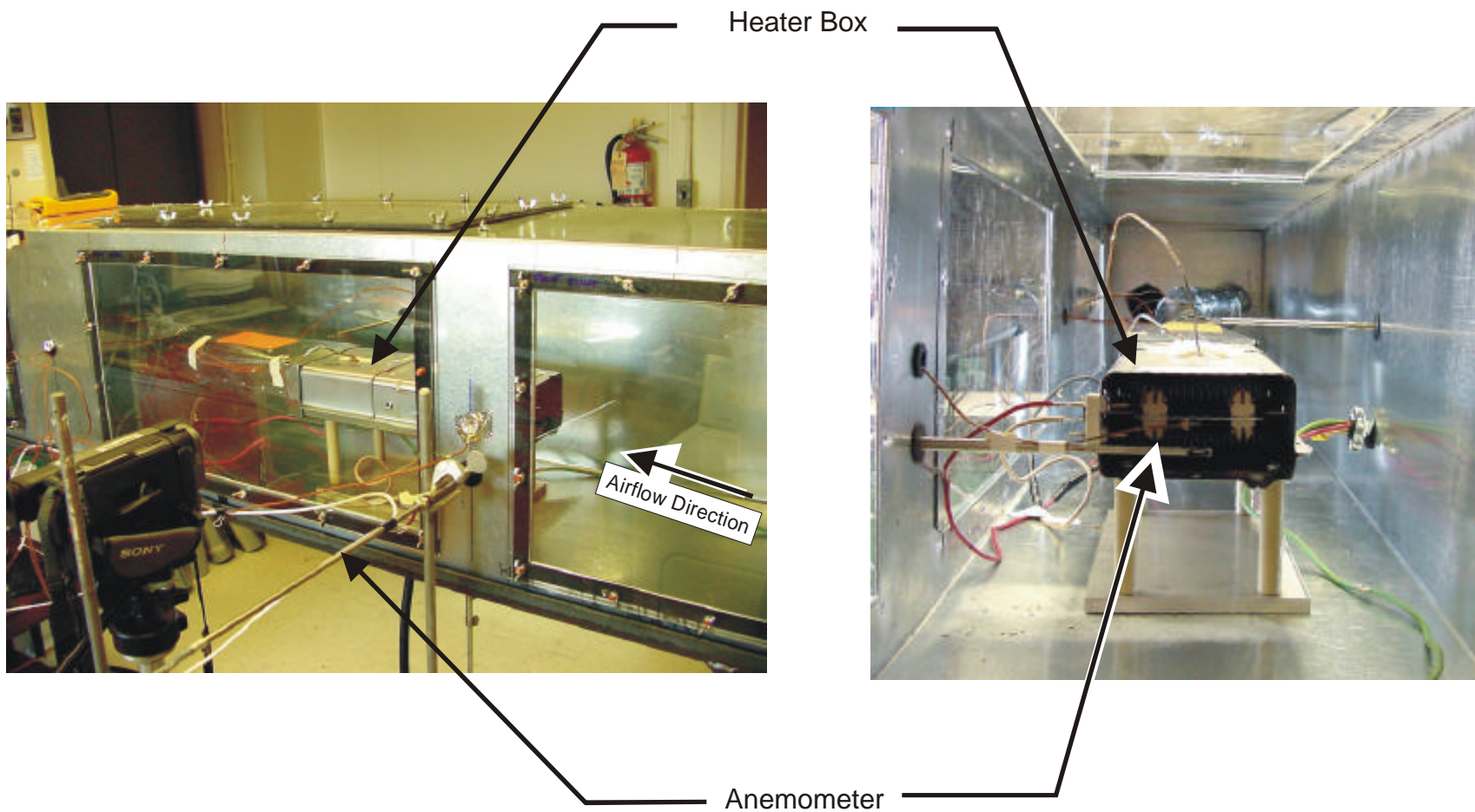
Figure 52. Test Setup for Lint Ignition
