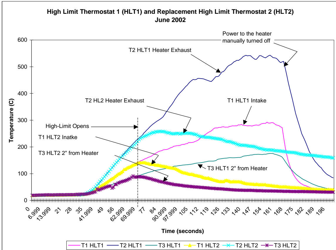
Figure 100. Failed Thermostat compared to a Replacement Thermostat
