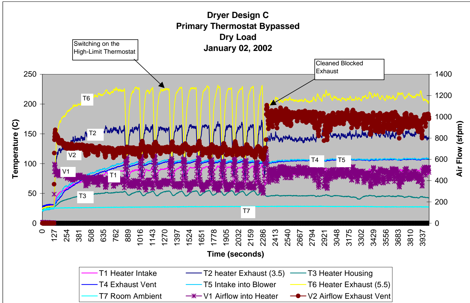
Figure 35. Dryer Design C – Primary Thermostat Bypassed
