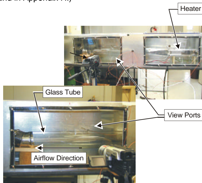
Figure 67. Setup with Glass Tube
