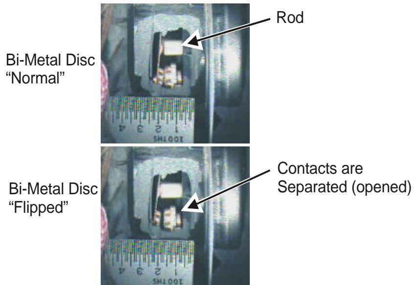
Figure 109. New High Limit Thermostat
