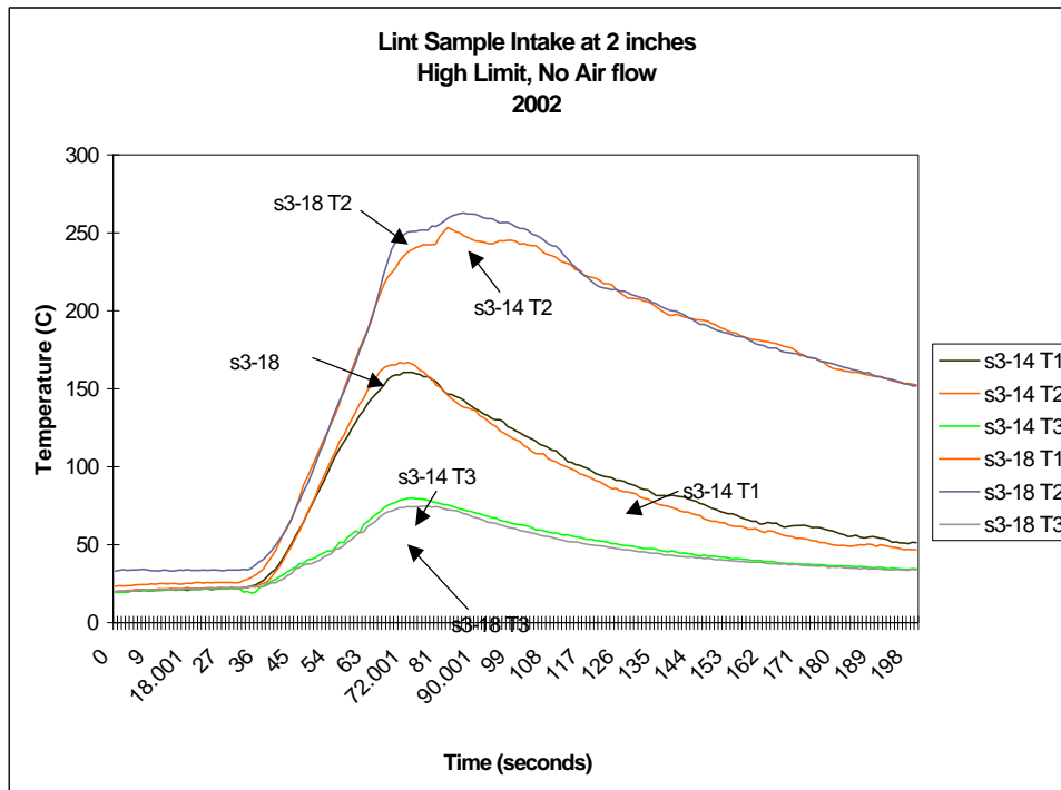
Figure 95. Lint Samples s3-14 and s3-18 Tested 2 Inches from the Heater Edge
