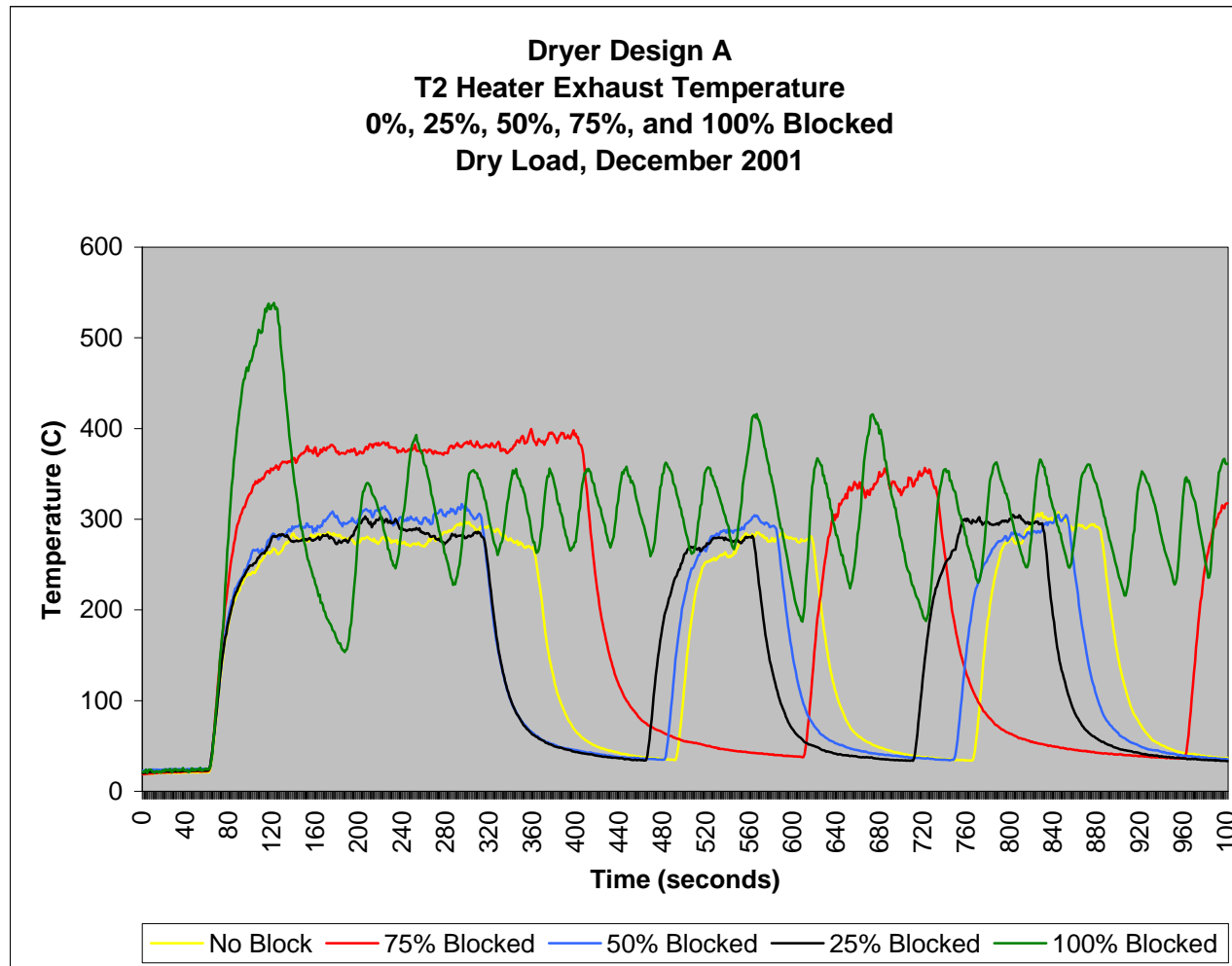
Figure 12. Dryer Design A – T2 Heater Exhaust Comparison
