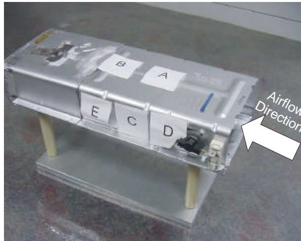
Figure 53. Location of Lint Samples on the Housing
