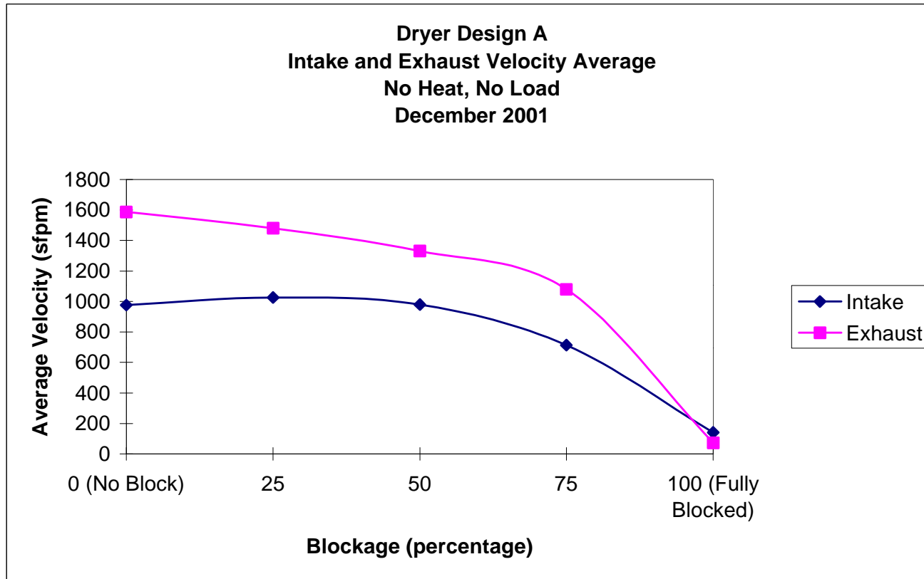
Figure 16. Dryer Design A – Average Airflow Velocities (No Heat and No Load)
