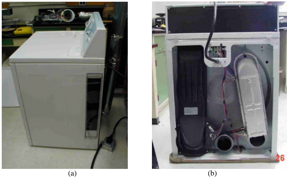
Figure 46. Dryer Design A Used in Task 3 Testing
