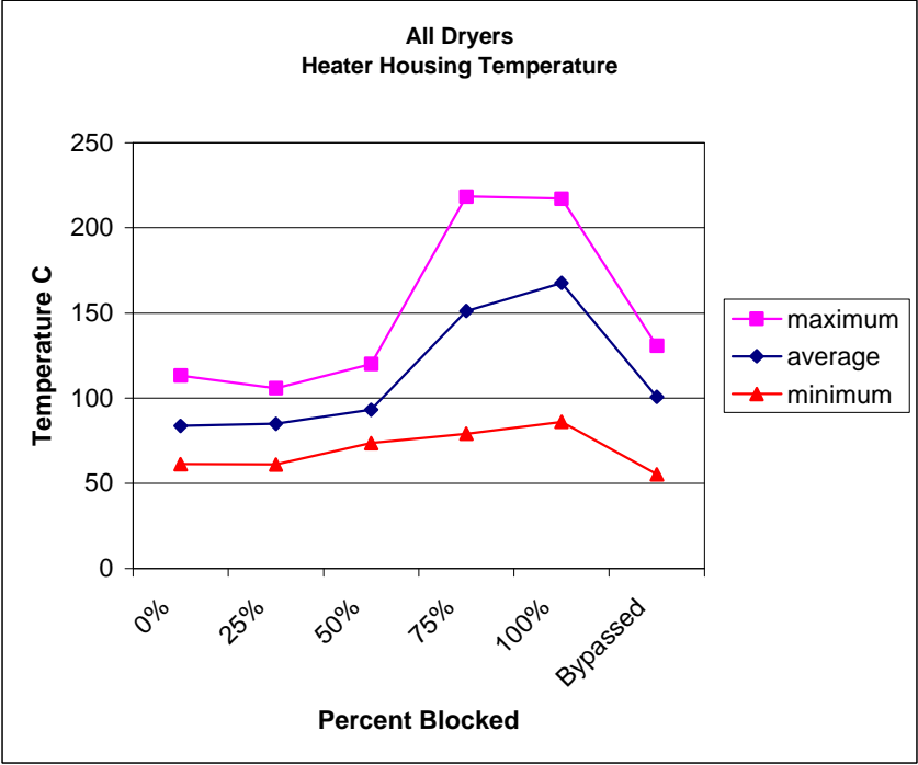
Figure 78. Heater Housing Temperature
