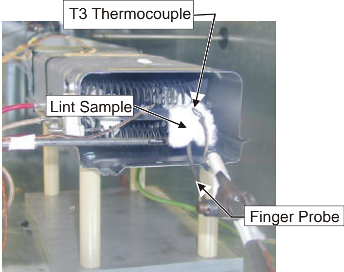
Figure 63. Lint Sample at Heater Intake
