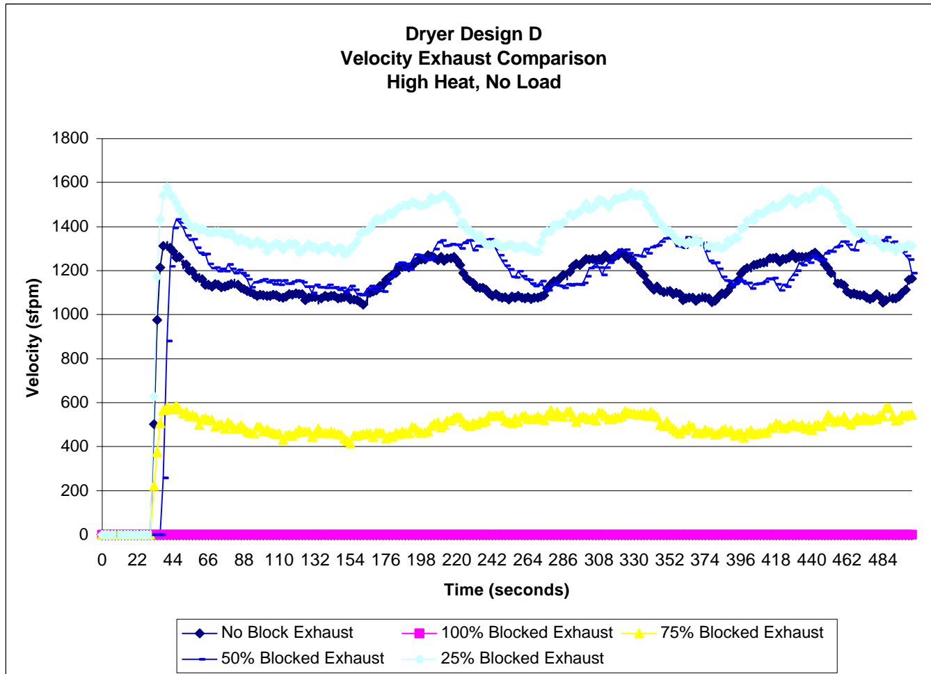
Figure 43. Dryer Design D – Exhaust Vent Air Velocity
