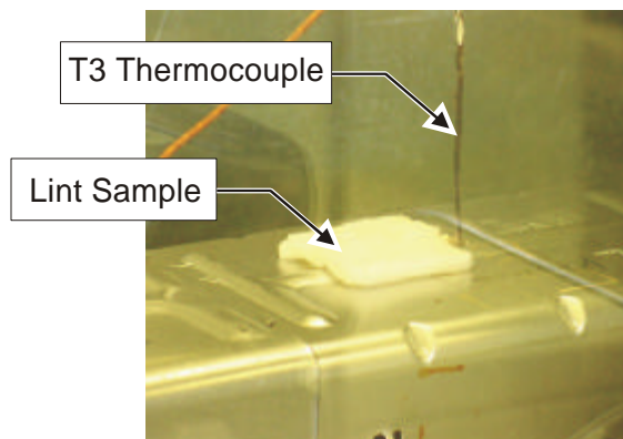
Figure 54. Lint Sample on Heater Housing at Location A
