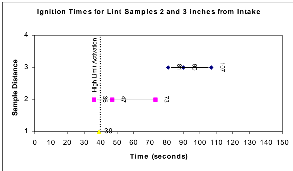
Figure 96. High Limit Activation Time Comparison at Sample 2 and 3 inches
