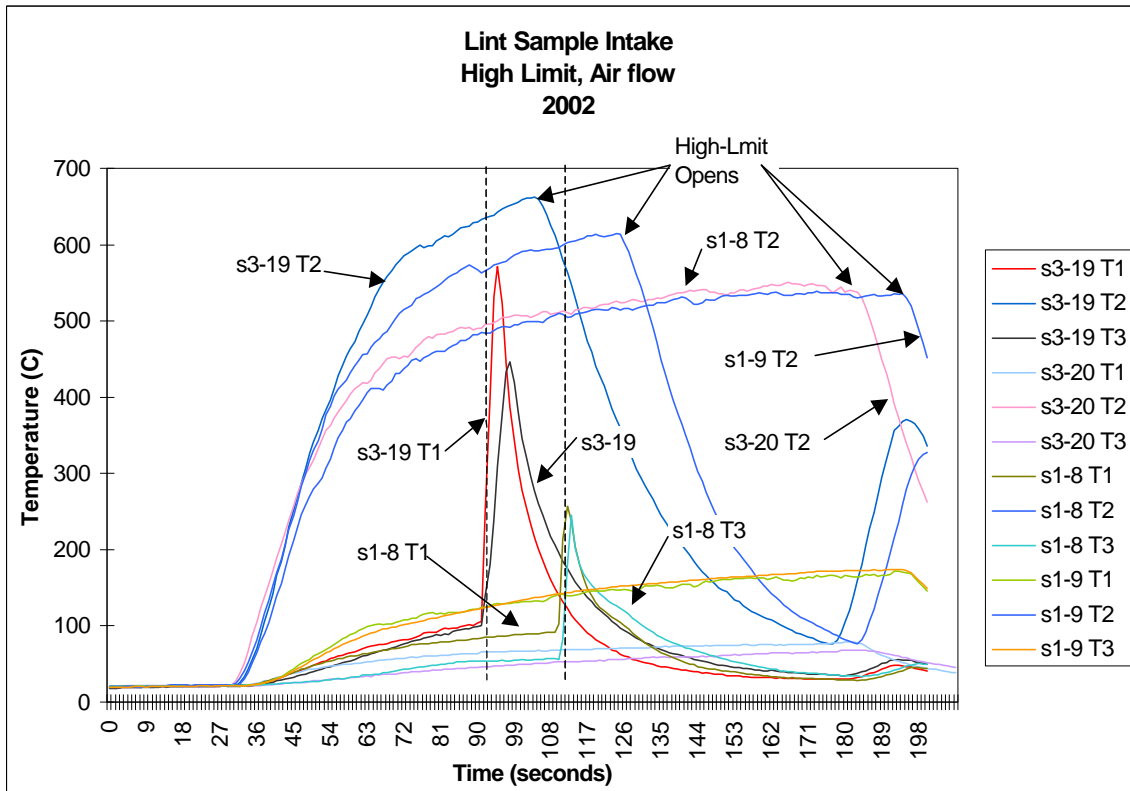
Figure 97. Lint Samples Tested 1 Inch from the Heater Edge with Airflow
