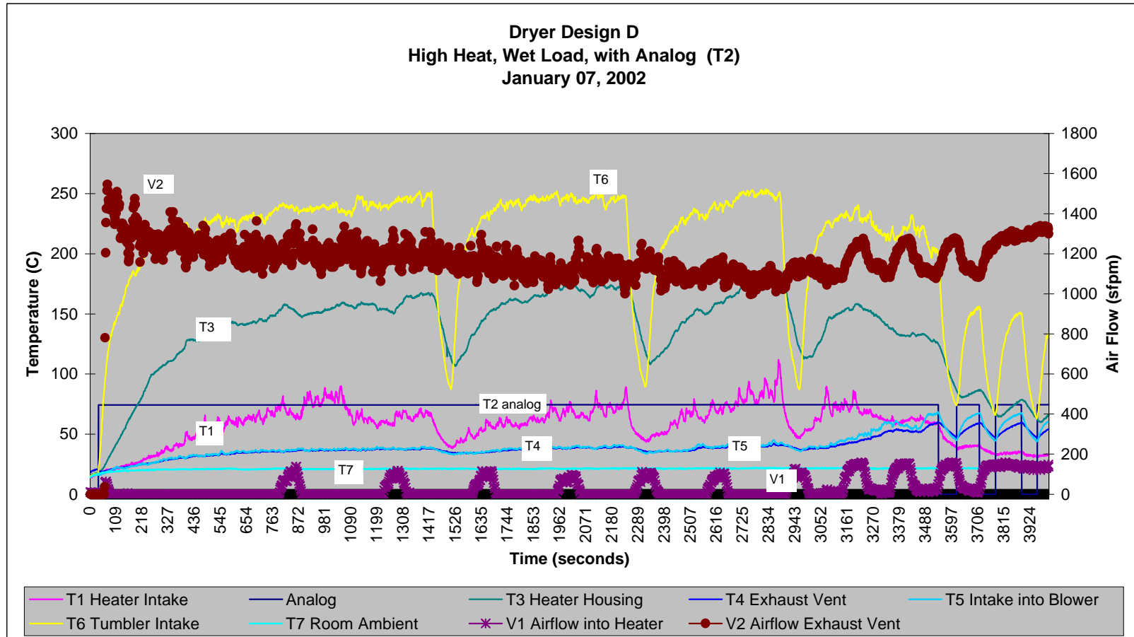
Figure 39. Thermocouple, Airflow and Relay (T2 Analog) Measurements
