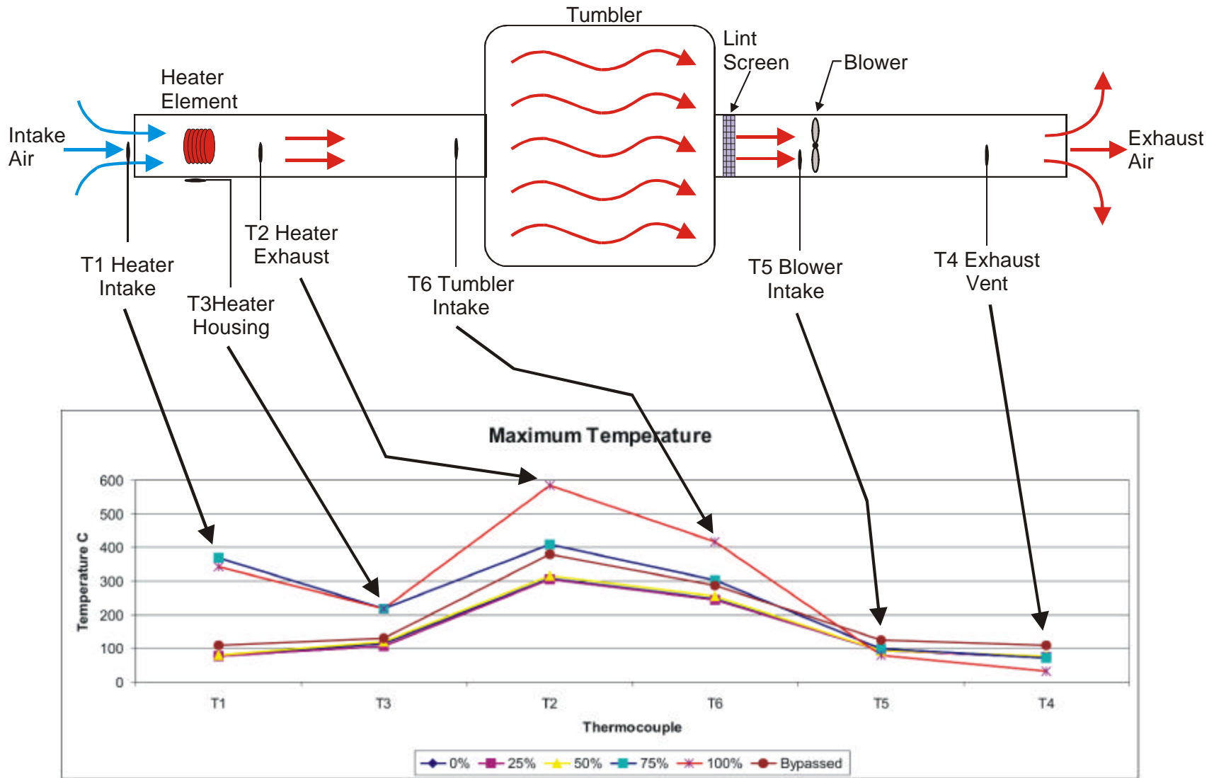
Figure 82. Maximum Temperatures for All Dryers at Each Location and Condition
