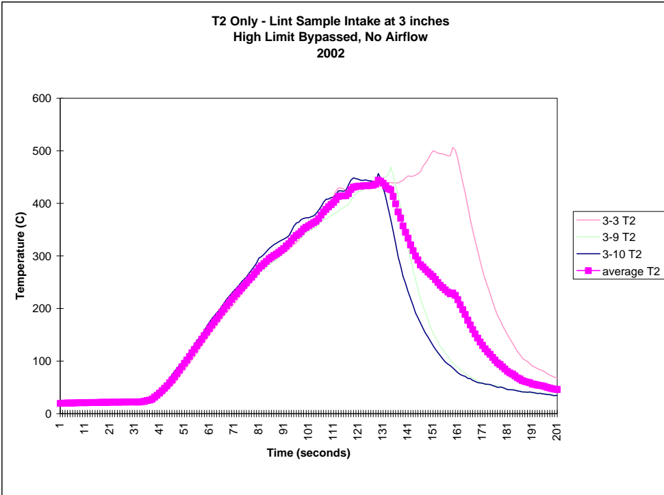
Figure 90. T2 Only - 3 Inches from the Heater Housing Edge
