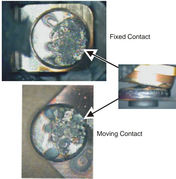
Figure 103. Contact Pads for High-Limit Thermostat 1 (HLT1)
