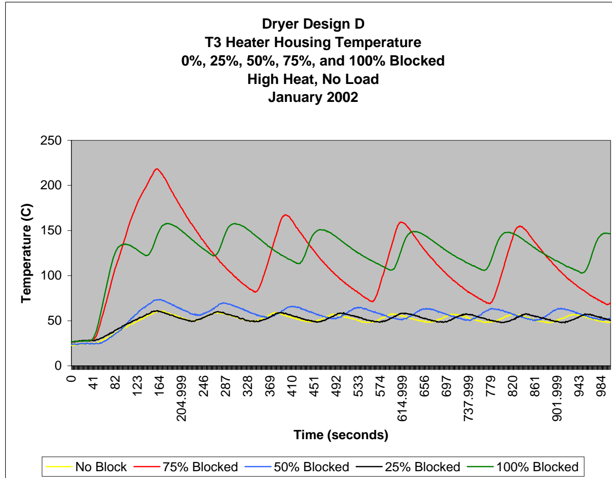
Figure 41. Dryer Design D – T3 Heater Housing Temperature Comparison
