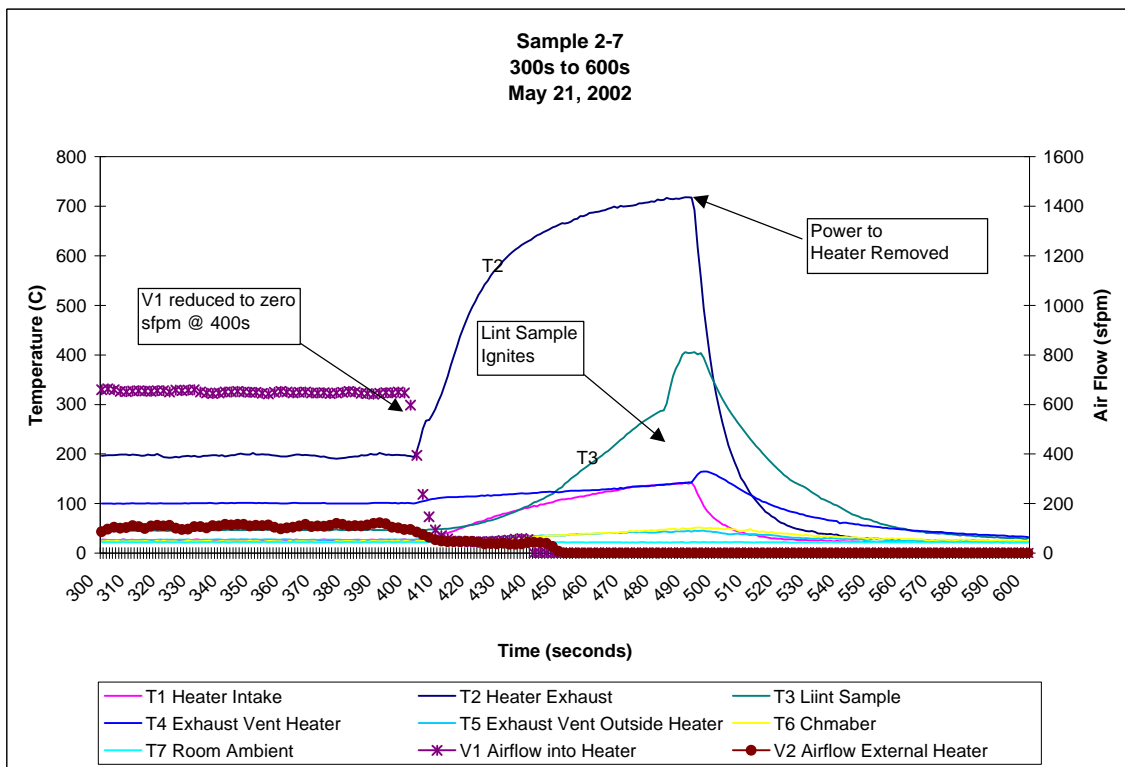
Figure 59. Sample s2-7 Thermocouple Traces
