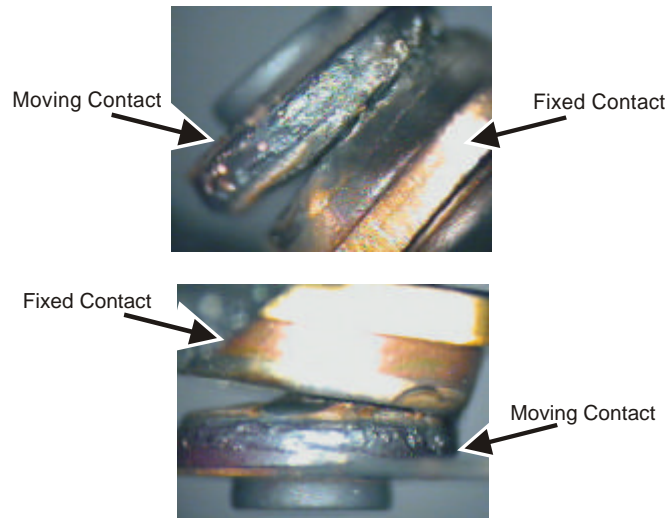
Figure 102. Contacts for High-Limit Thermostat 1 (HLT1)
