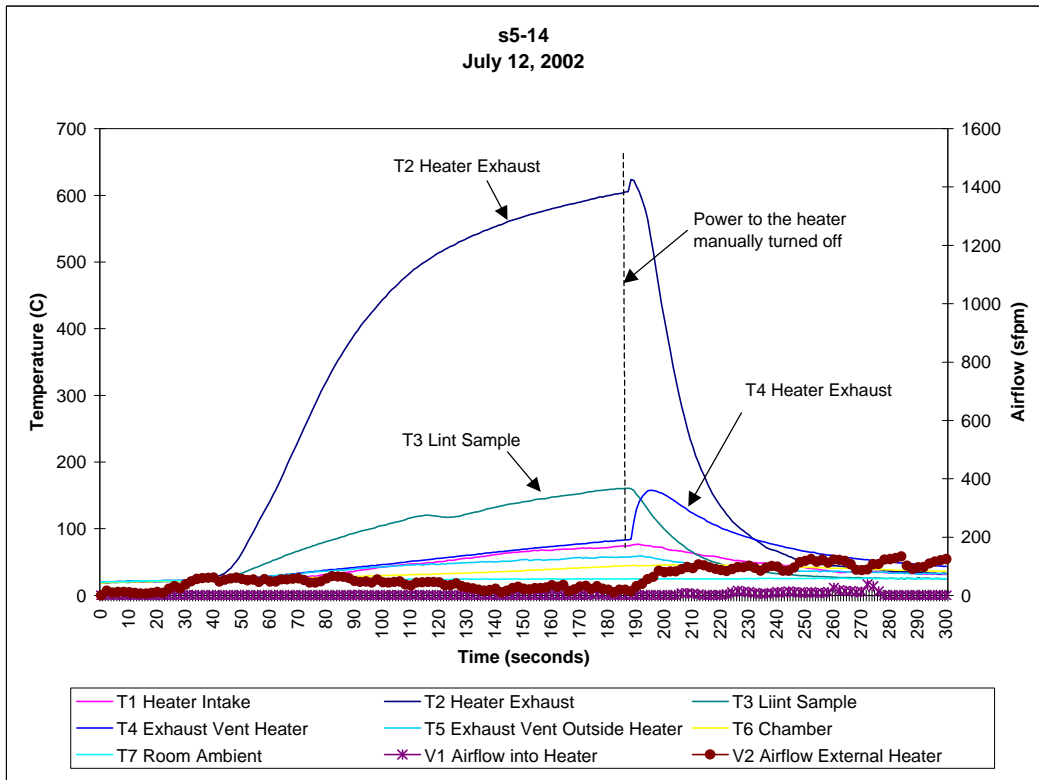
Figure 104. Sample s5-14 with High Limit Thermostat in Series
