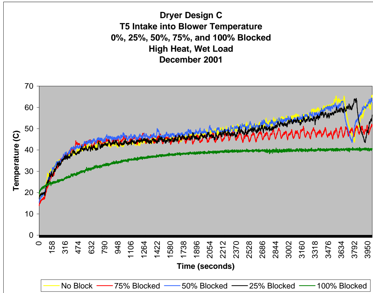
Figure 31. Dryer Design C – T5 Intake into the Blower Comparison
