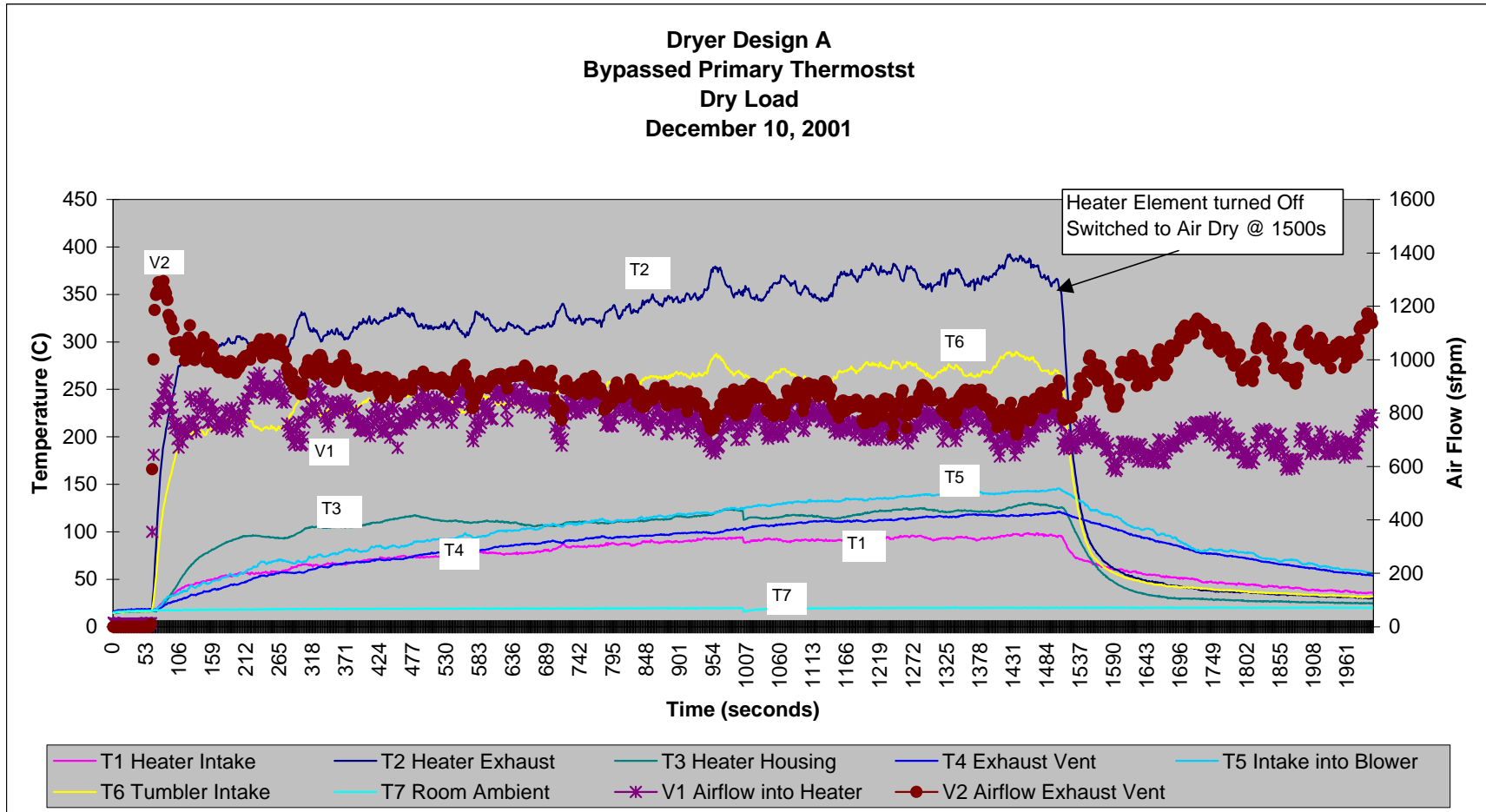
Figure 17. Dryer Design A – Primary Thermostat Bypassed
