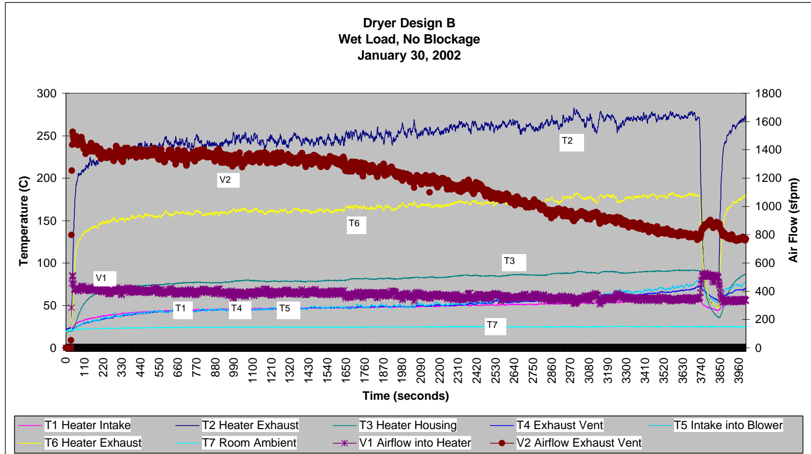
Figure 19. Dryer Design B – Thermocouple and Airflow Measurements (Wet Load)
