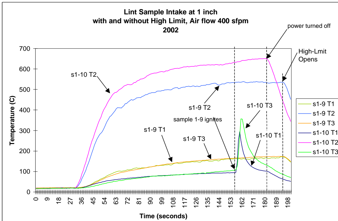
Figure 98. Samples Tested at 1 Inch, With and Without High-Limit Thermostat
