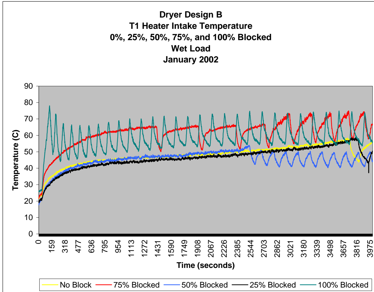
Figure 20. Dryer Design B – T1 Heater Intake Comparison
