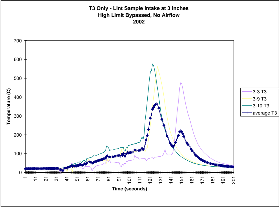
Figure 91. T3 Only - 3 Inches from the Heater Housing Edge
