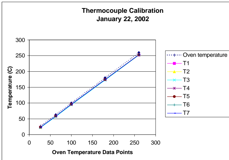
Figure 6. Thermocouple Response After Task 2 Testing
