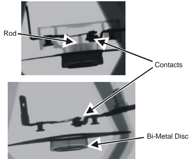
Figure 101. X-ray Images of High-Limit Thermostat 1 (HLT1)
