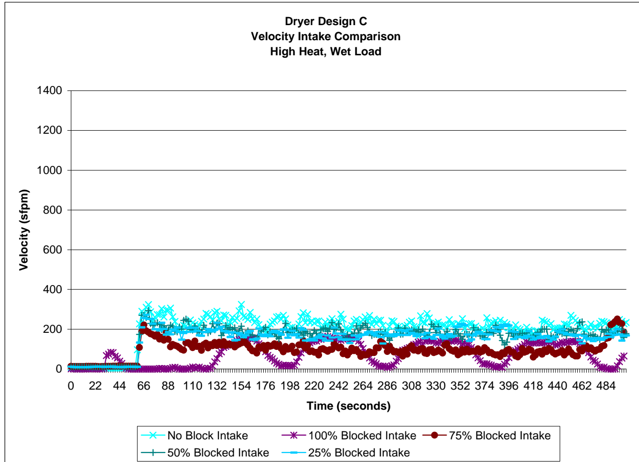
Figure 32. Dryer Design C – Intake Air Velocity
