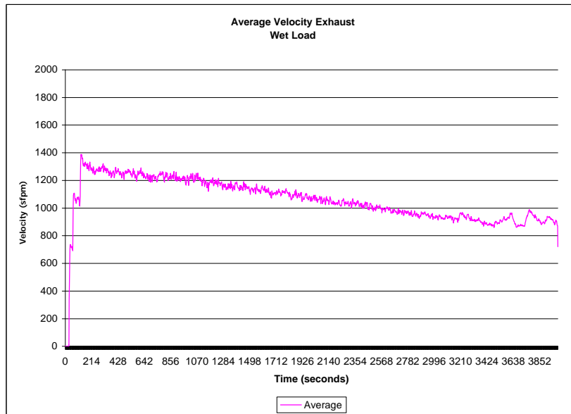
Figure 84. Calculated Average Exhaust Air Velocity
