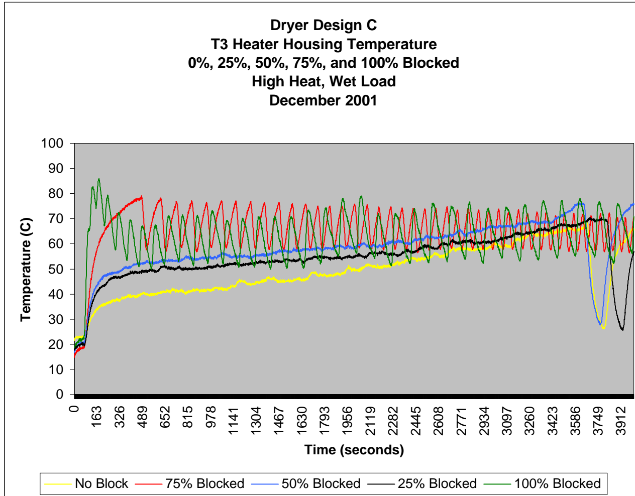
Figure 30. Dryer Design C – T3 Heater Housing Comparison
