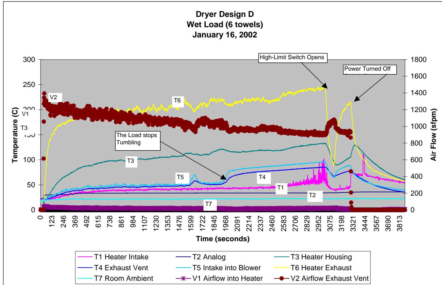
Figure 45. Dryer Design D – Primary Thermostat Bypassed
