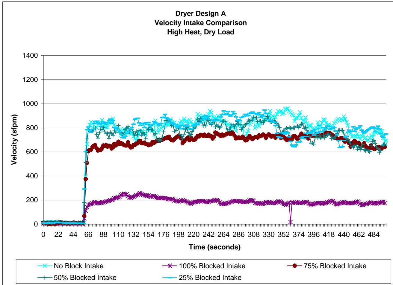
Figure 13. Dryer Design A – Intake Air Velocity
