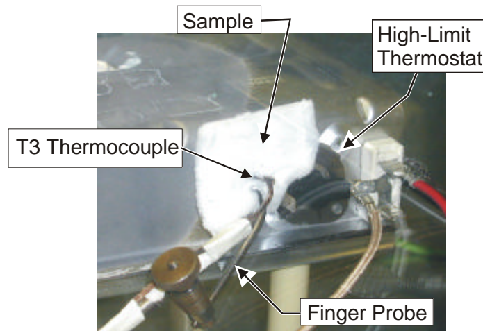
Figure 60. Sample s2-2 Tested at Location D
