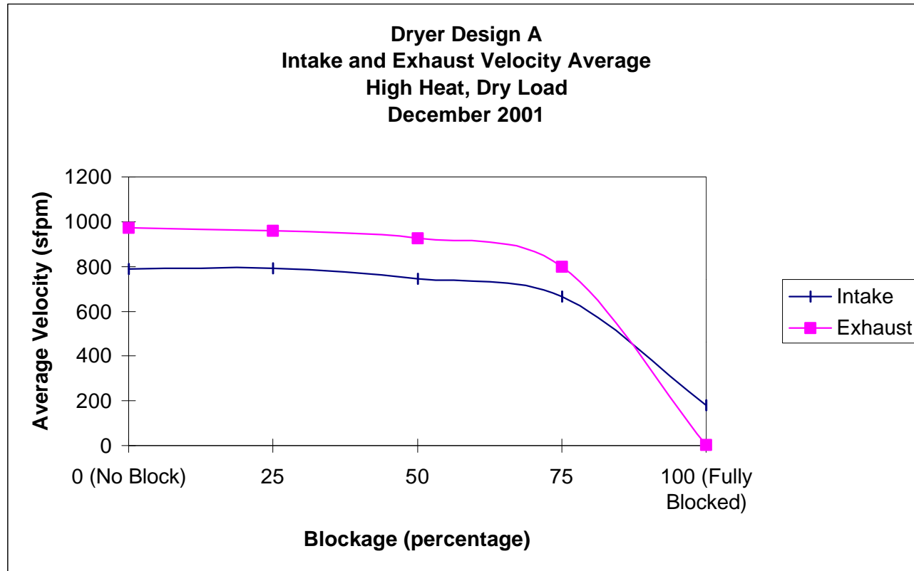
Figure 15. Dryer Design A – Average Airflow Velocities (High Heat and Dry Load)
