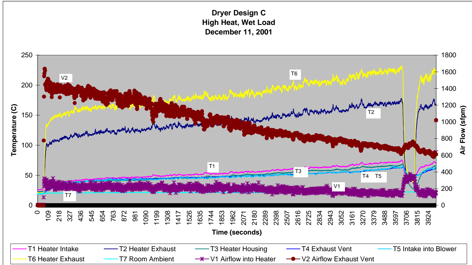
Figure 28. Dryer Design C – Thermocouple and Airflow Measurements (Wet Load)
