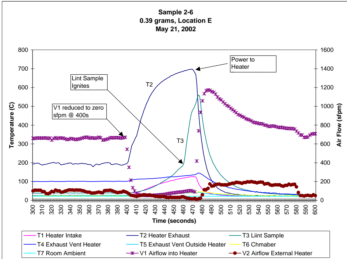
Figure 62. Thermocouple Traces for Sample s2-6 at Location E
