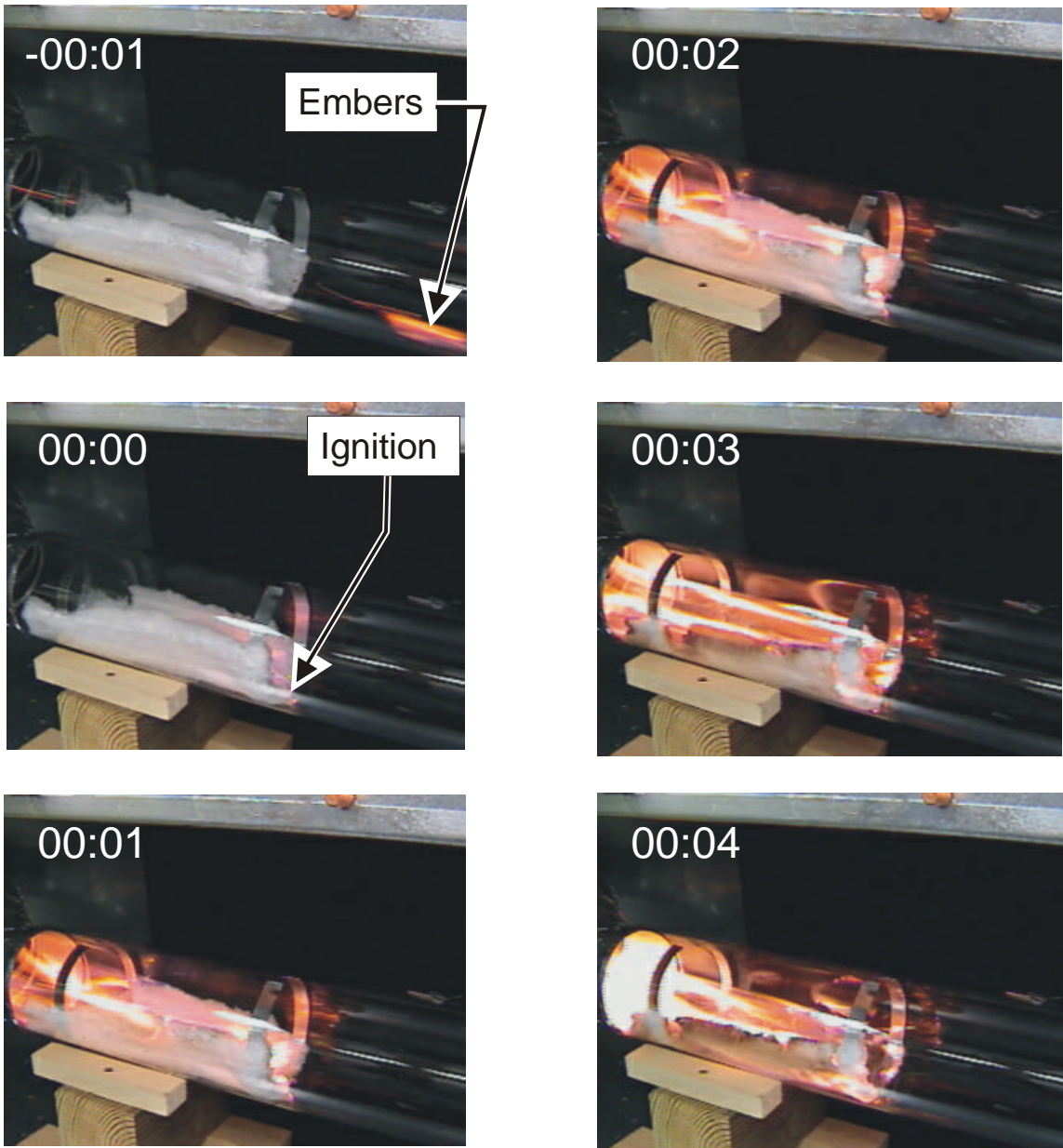
Figure 69. Target Sample Igniting During Test 1
