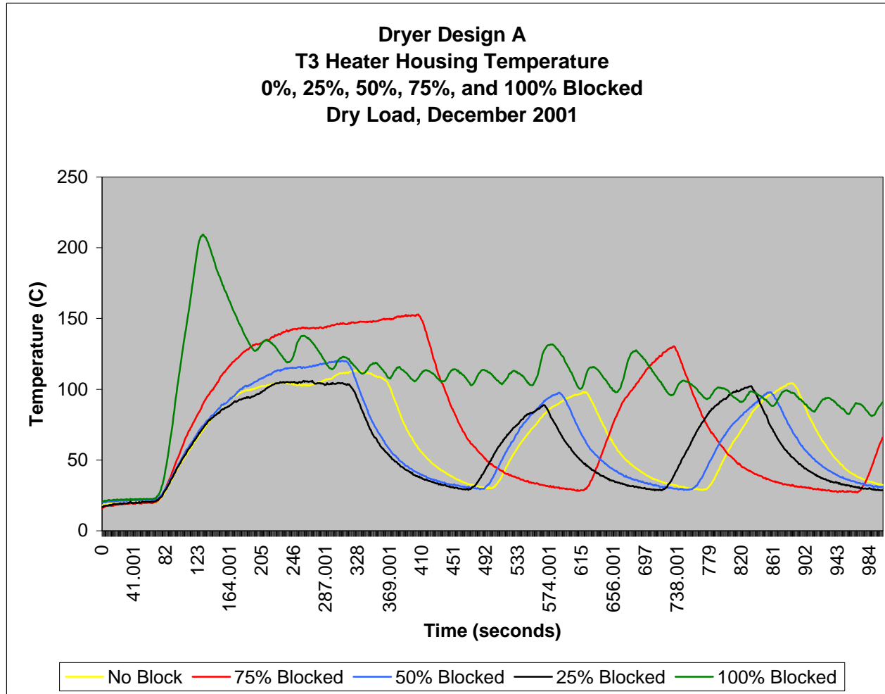
Figure 11. Dryer Design A – T3 Heater Housing Comparison
