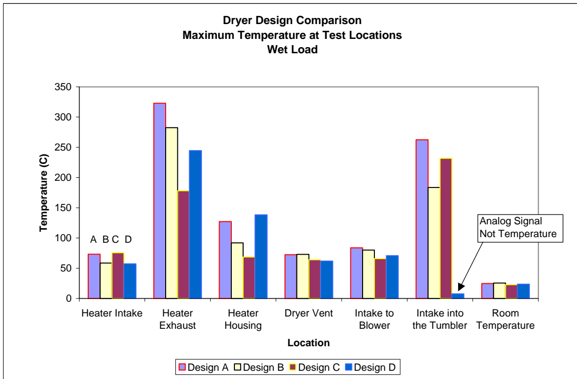
Figure 75. Maximum Temperatures Measured at Location
