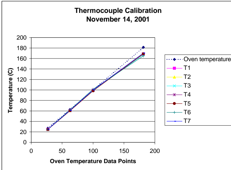
Figure 5. Thermocouple Response Before Task 2 Testing
