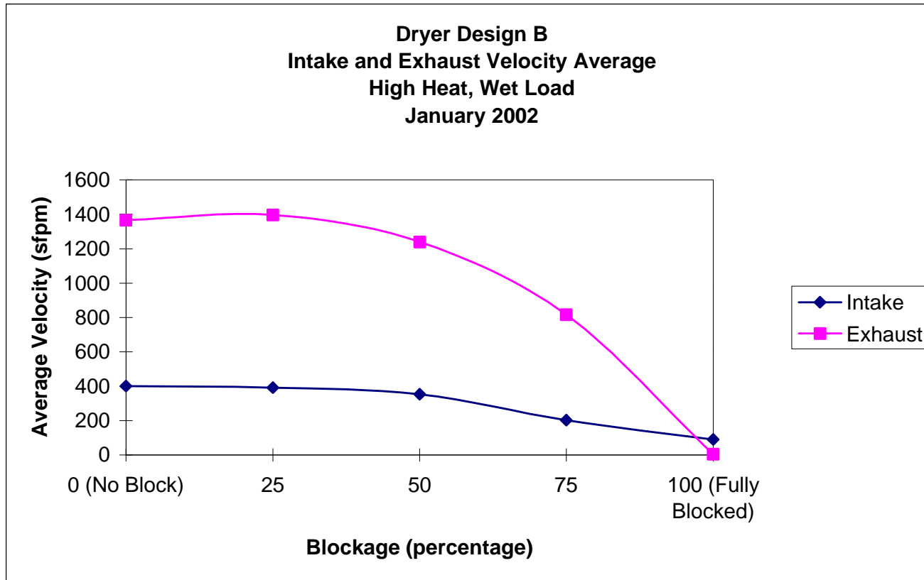
Figure 25. Dryer Design B – Average Airflow Velocities (High Heat and Wet Load)
