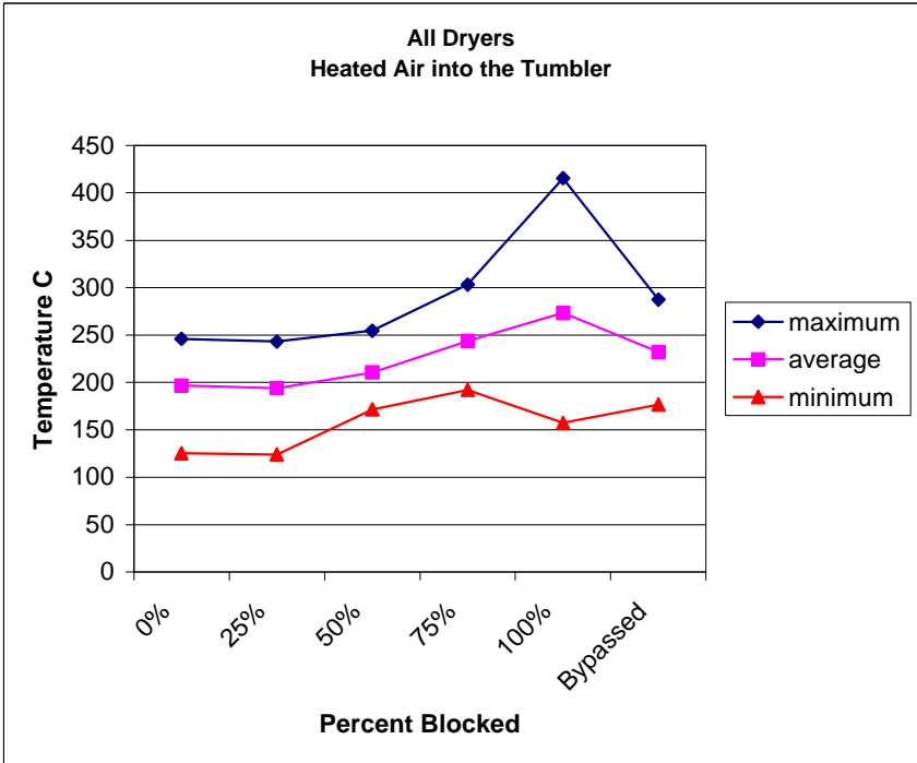
Figure 81. Intake into the Tumbler Temperature
