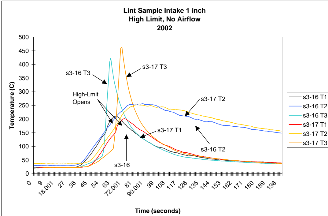
Figure 94. Lint Samples s3-16 and s3-17 Tested 1 Inch from the Heater Edge
