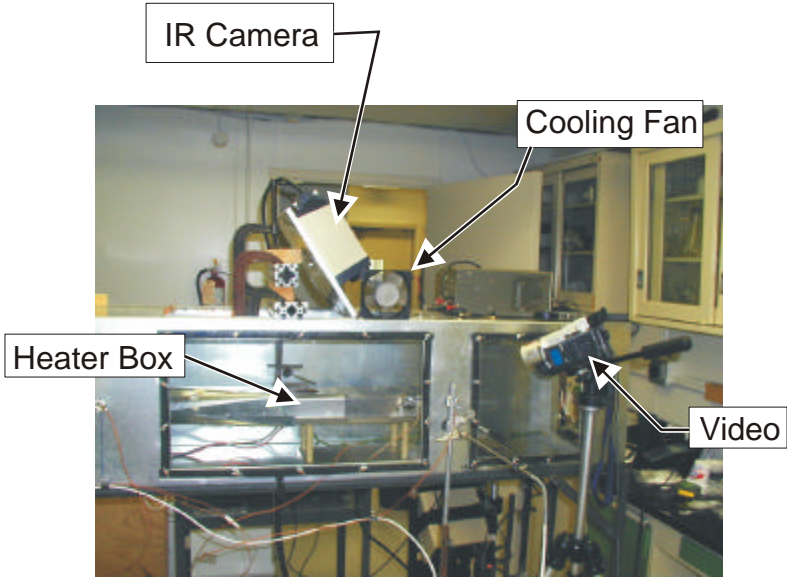
Figure 64. Infrared Camera Setup
