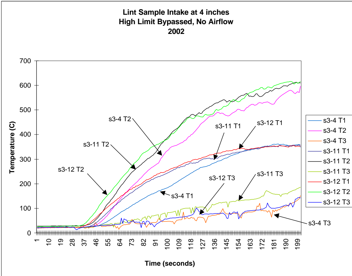
Figure 92. Lint Samples Tested 4 Inches from the Heater Housing Edge
