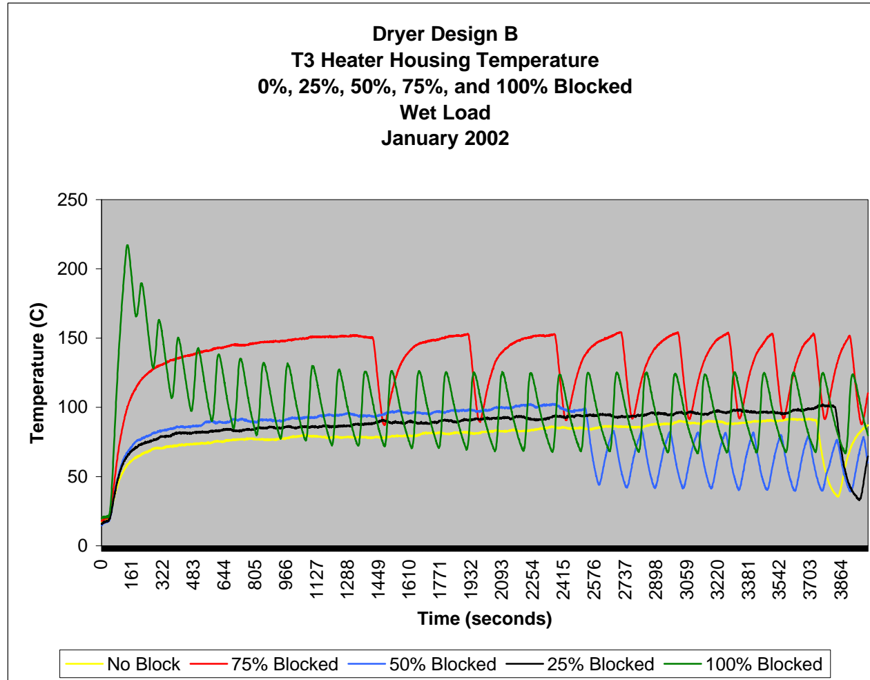
Figure 21. Dryer Design B – T3 Heater Housing Comparison
