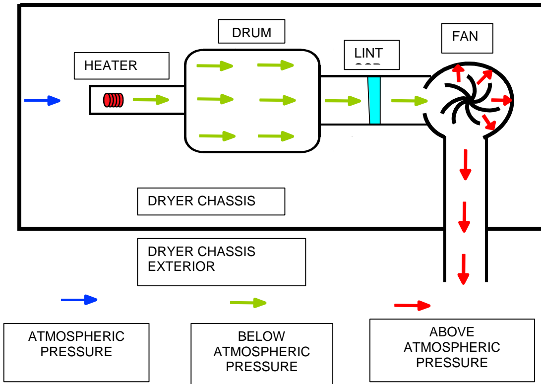
Figure 86. An Illustration of Airflow through the Dryer and Blower
