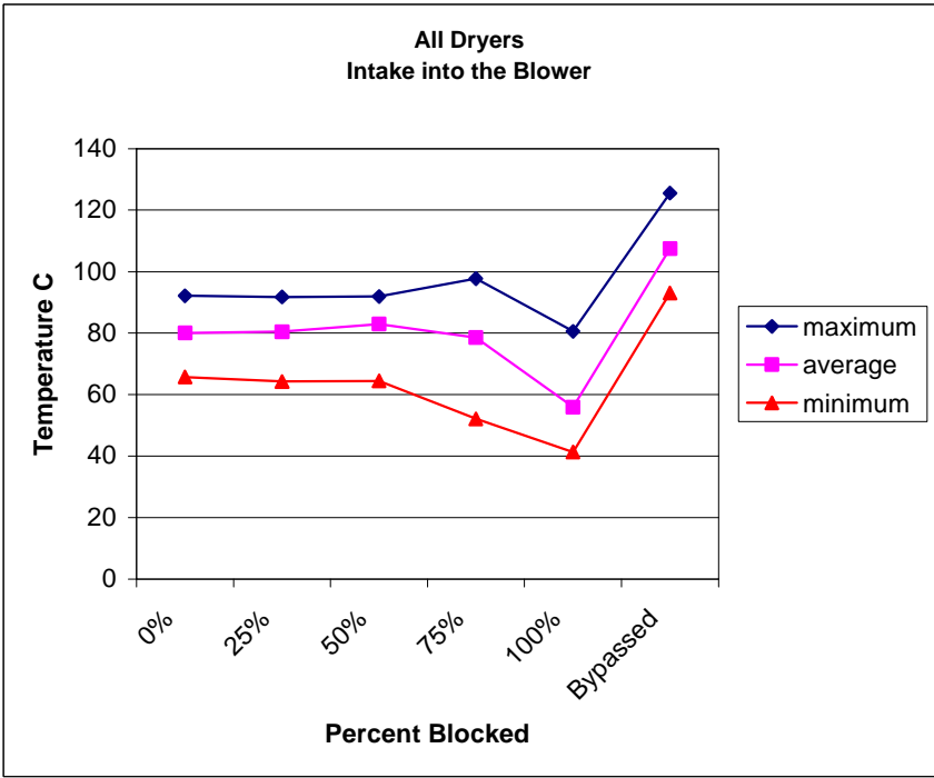
Figure 80. Intake into the Blower Temperature
