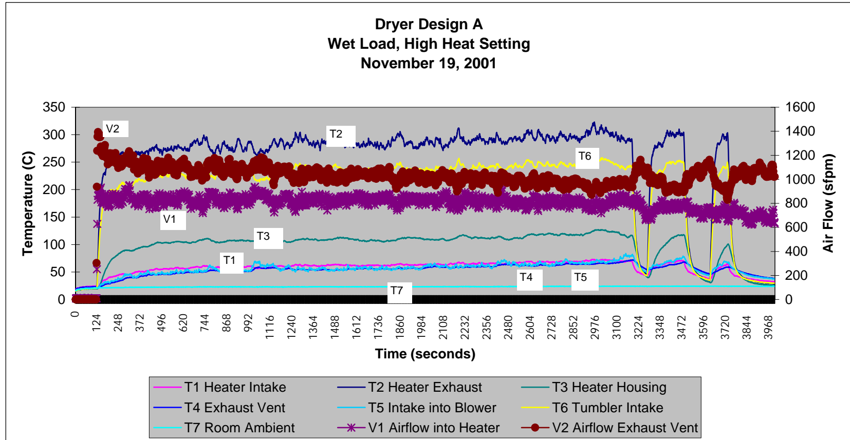
Figure 9. Dryer Design A – Thermocouple and Airflow Measurements with a Wet Load
