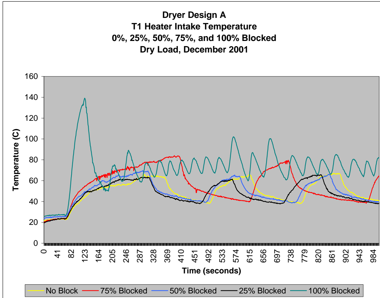
Figure 10. Dryer Design A – T1 Heater Intake Comparison
