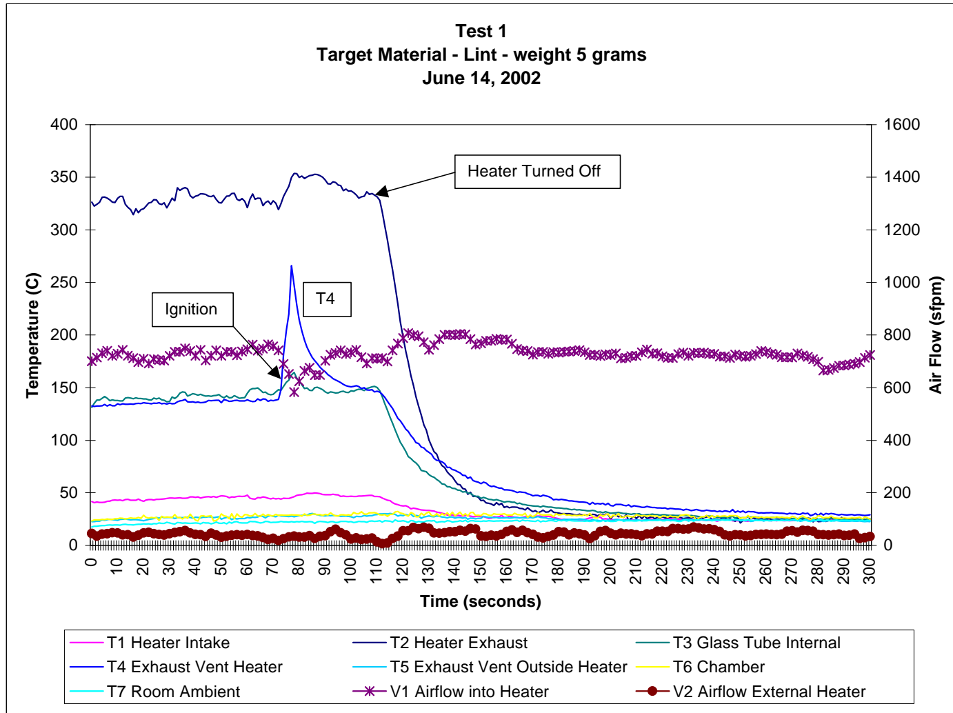
Figure 70. Test 1 – Thermocouple and Airflow Measurements Task 4- Test 1 (Ignition of Target Materials by Exhaust Embers)
