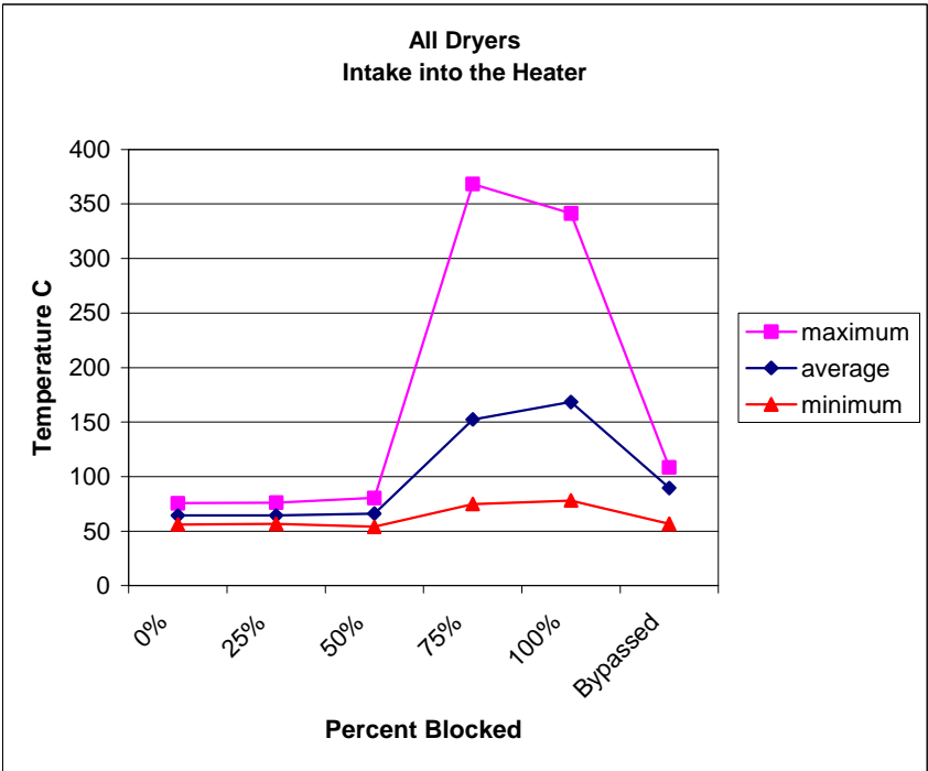
Figure 76. Intake into the Heater
