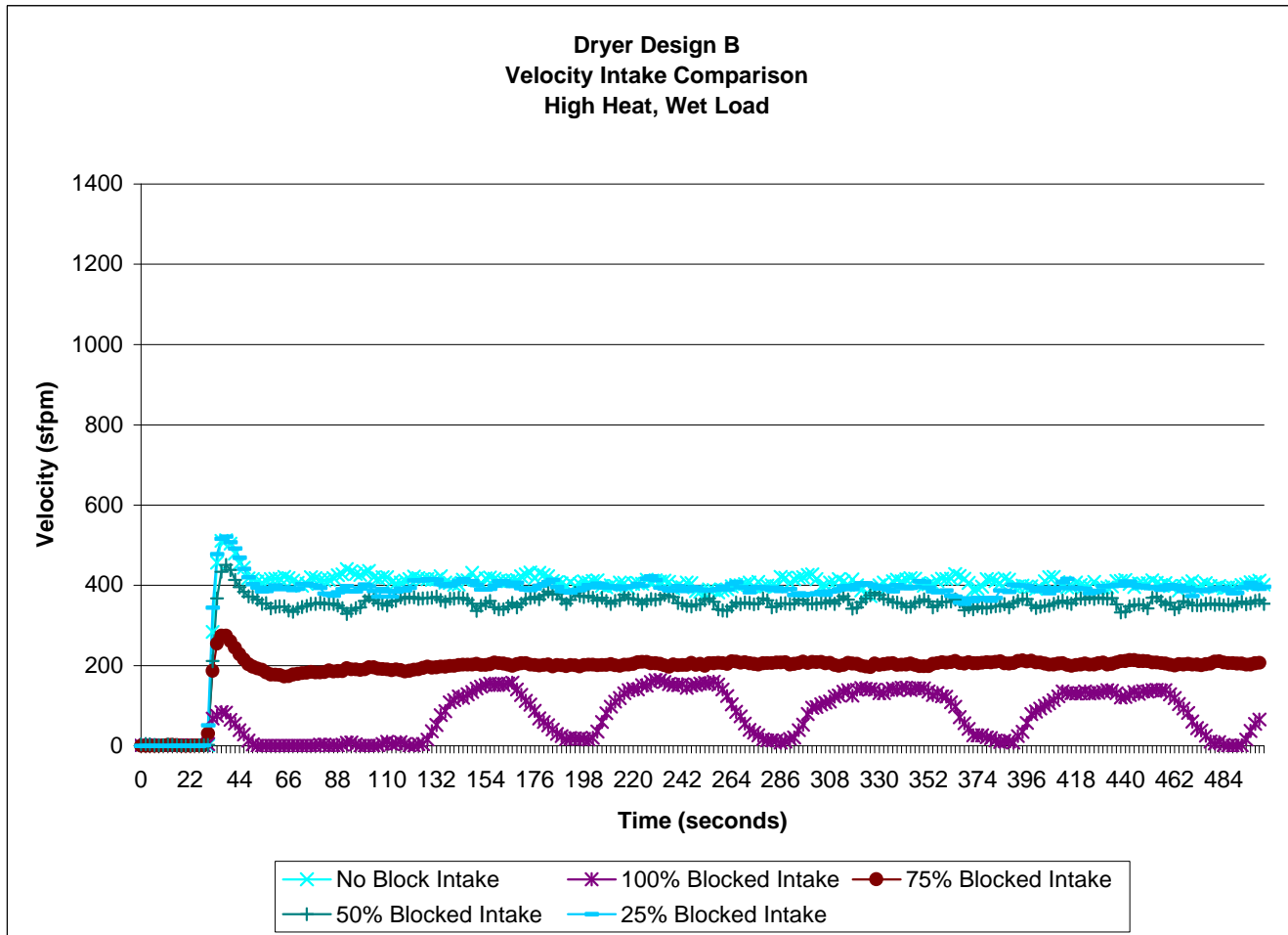
Figure 23. Dryer Design B – Intake Air Velocity
