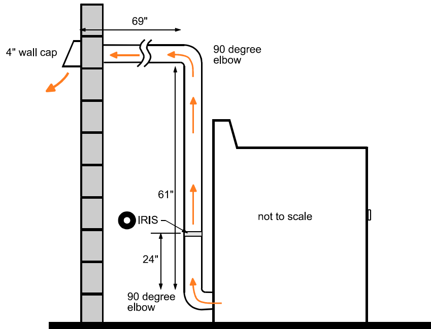
Figure 4. Exhaust Vent Setup
