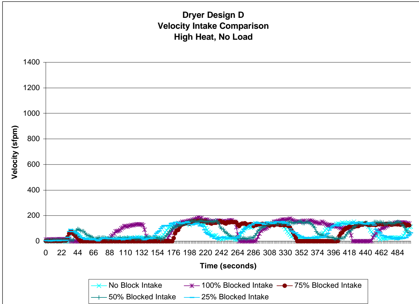
Figure 42. Dryer Design D – Intake Air Velocity
