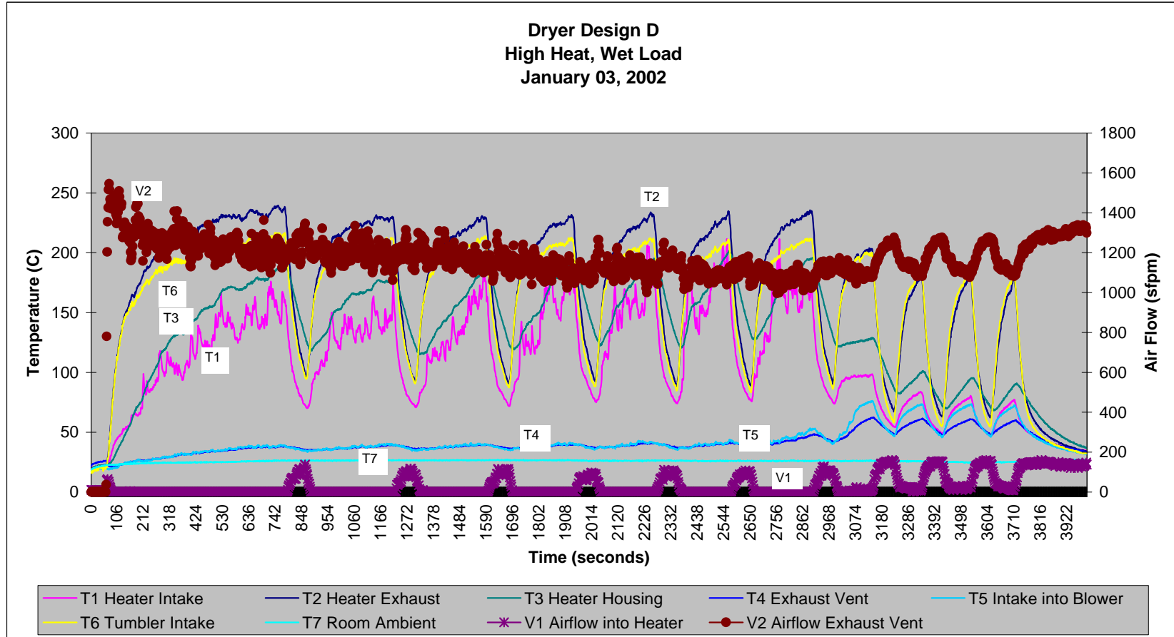
Figure 38. Dryer Design D – Thermocouple and Airflow Measurements (Wet Load)
