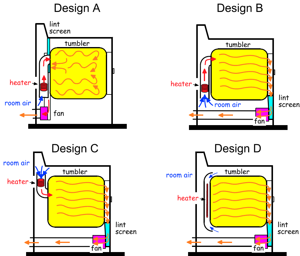
Figure 1. Dryer Design Characteristics (Not to scale)
