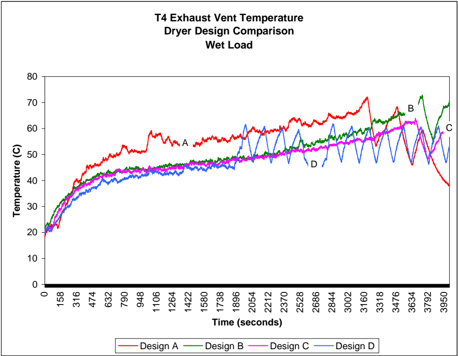
Figure 74. Dryer Design Comparison for T4, Exhaust Vent
