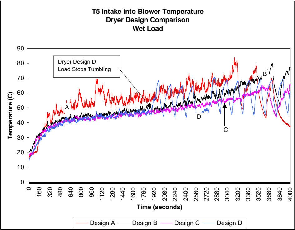
Figure 73. Dryer Design Comparison for T5, Blower Intake
