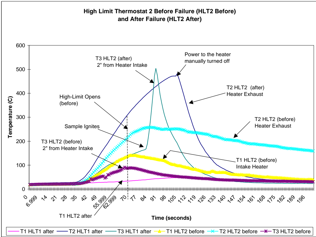
Figure 105. High-Limit Thermostat 2 (HLT2) before and after Failure
