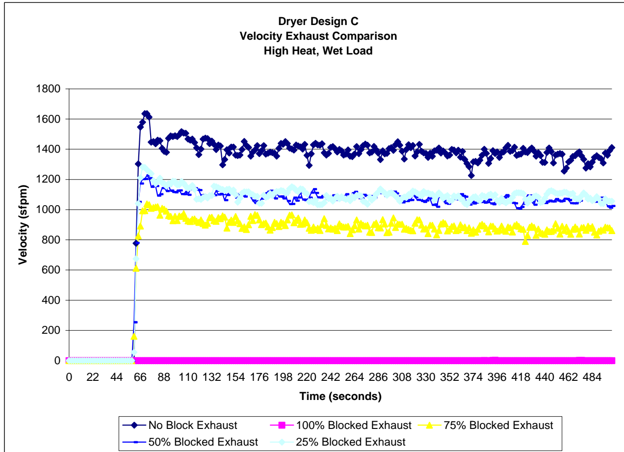
Figure 33. Dryer Design C – Exhaust Vent Air Velocity
