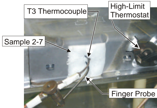
Figure 58. Sample s2-7 on the Side of the Heater Housing at Location C
