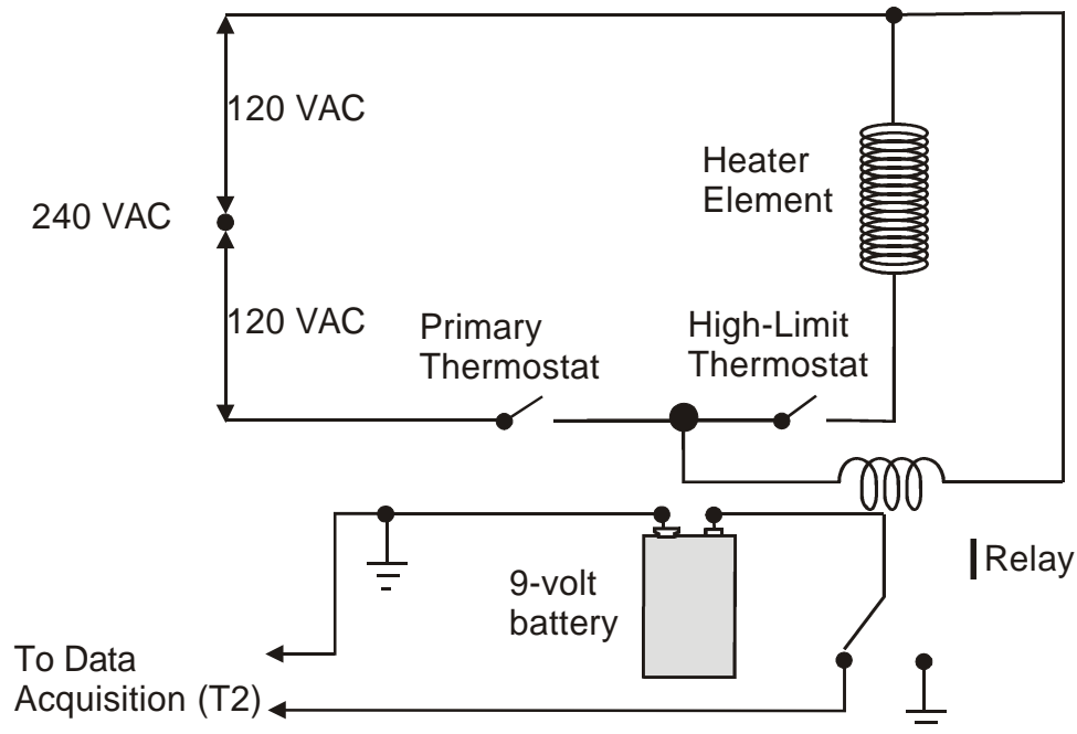
Figure 37. Setup with a Relay and Battery for T2 Analog
