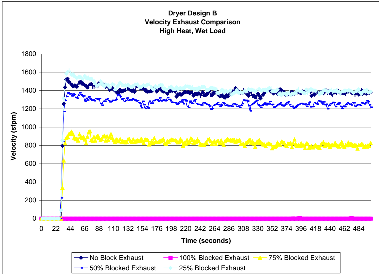
Figure 24. Dryer Design B – Exhaust Vent Air Velocity
