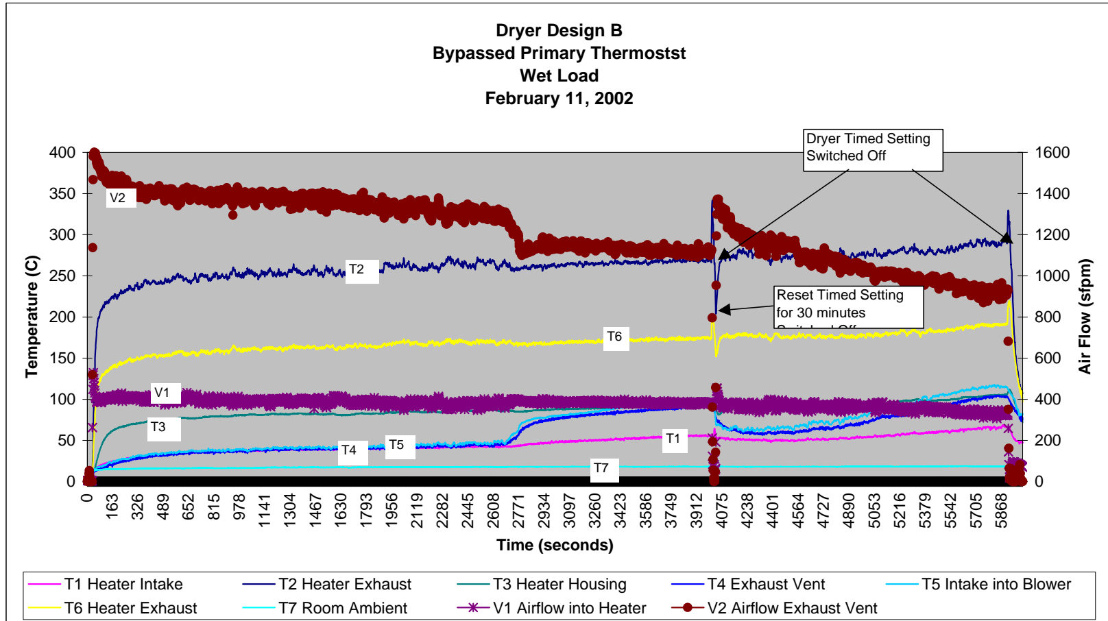
Figure 26. Dryer Design B – Primary Thermostat Bypassed
