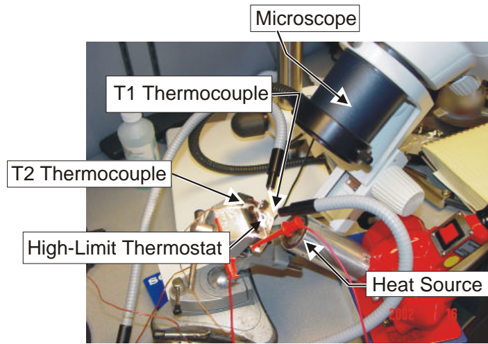
Figure 108. Setup for Testing High-Limit Thermostats
