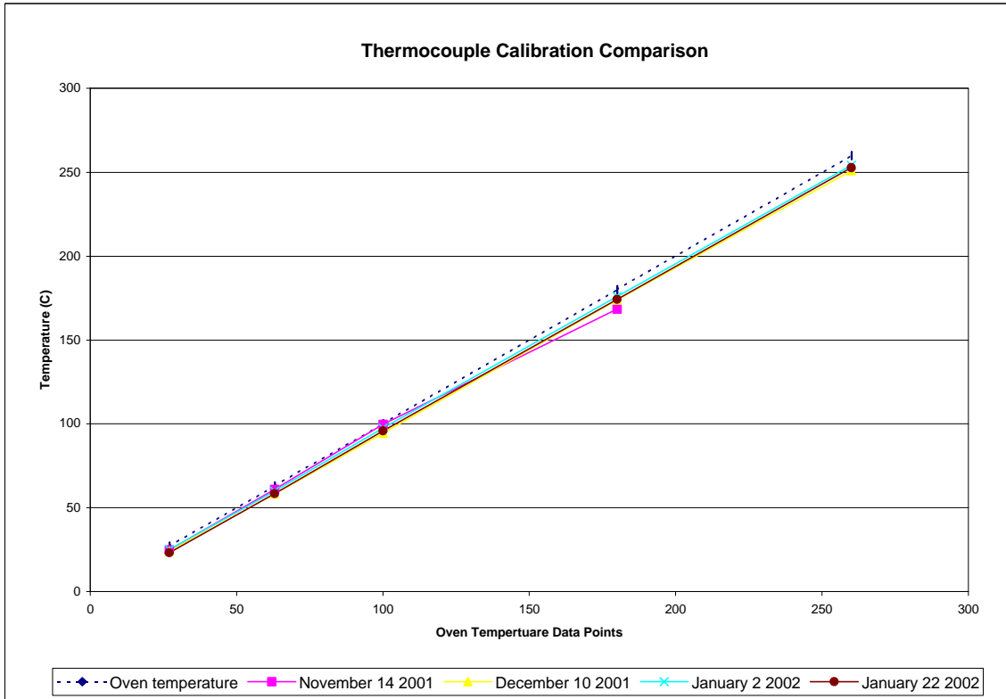
Figure 7. Average Responses per Oven Set Temperatures and Day
