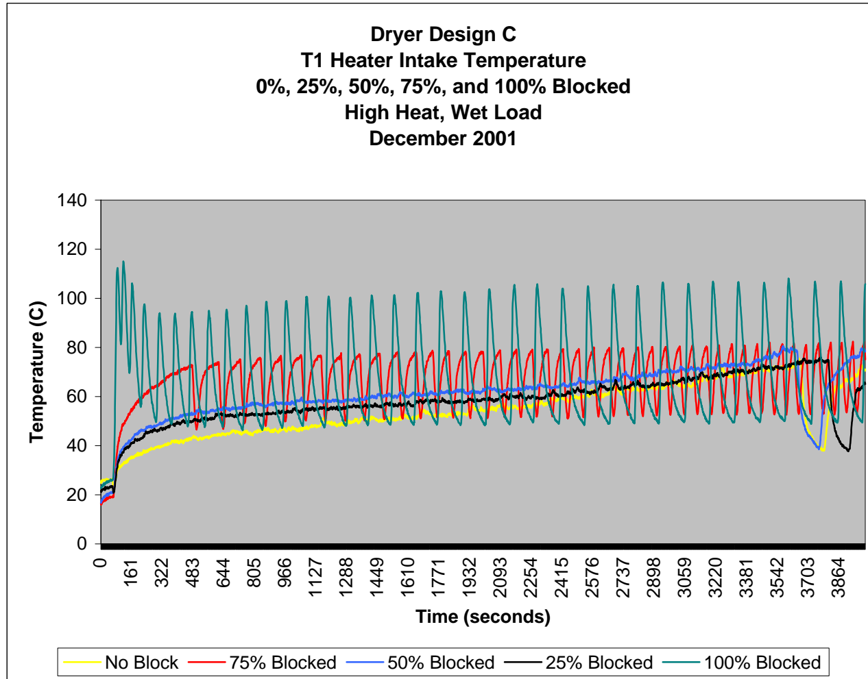
Figure 29. Dryer Design C – T1 Heater Intake Comparison
