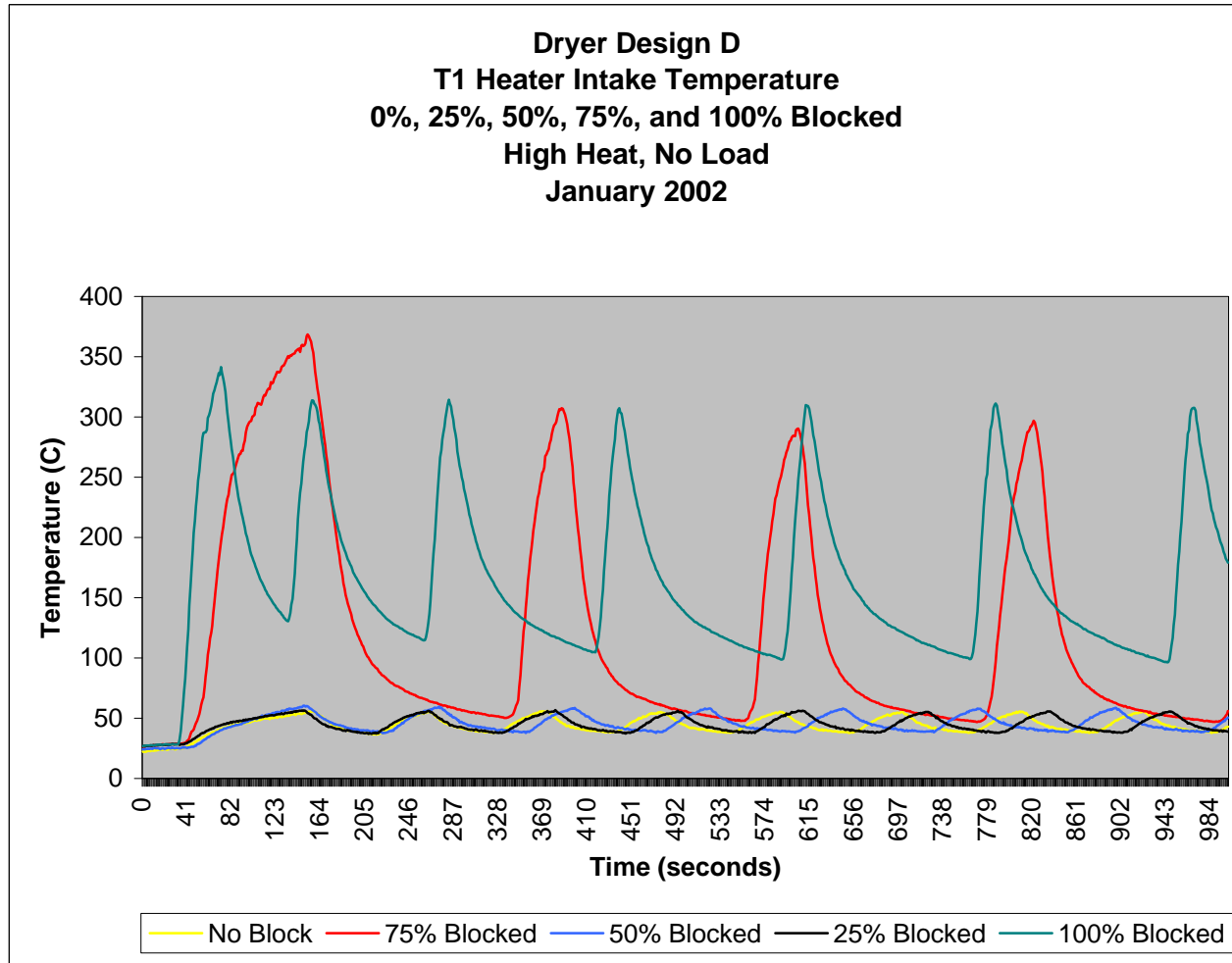
Figure 40. Dryer Design D – T1 Heater Intake Comparison
