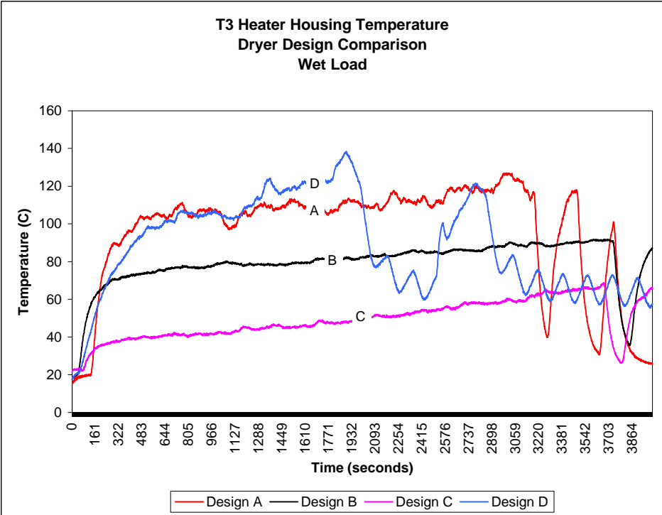
Figure 72. Dryer Design Comparison for T3, Heater Housing
