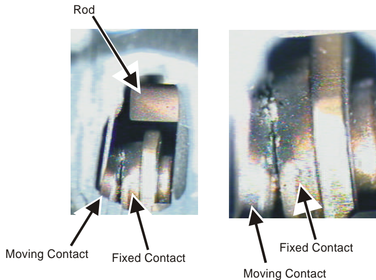
Figure 107. Internal View for High-Limit Thermostat 2
