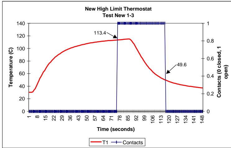
Figure 110. Thermocouple Data for the New High-Limit Thermostat
