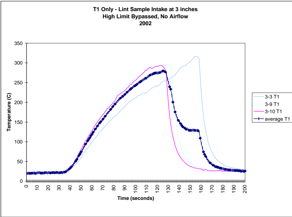
Figure 89. T1 Only - 3 Inches from the Heater Housing Edge
