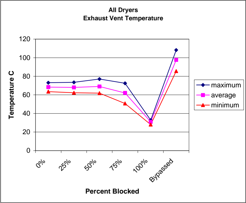
Figure 79. Exhaust Vent Temperature
