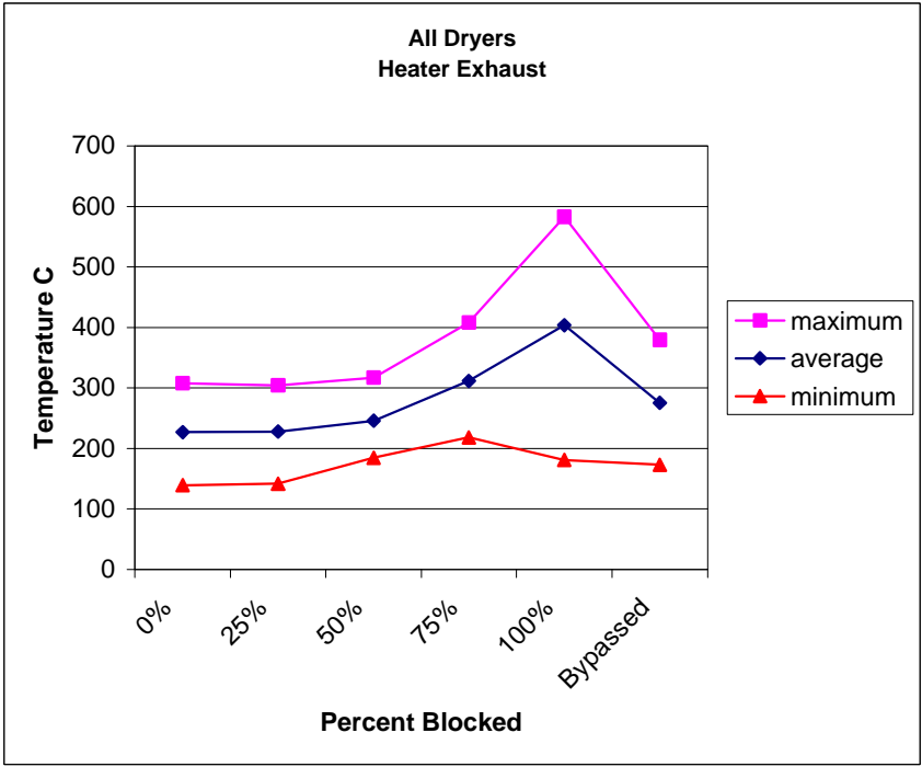
Figure 77. Heater Exhaust Temperature
