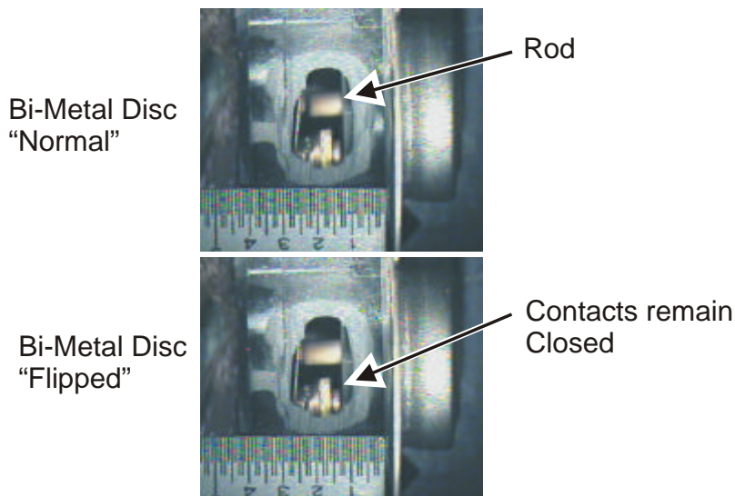
Figure 111. Second Failed High Limit Thermostat, HLT2
