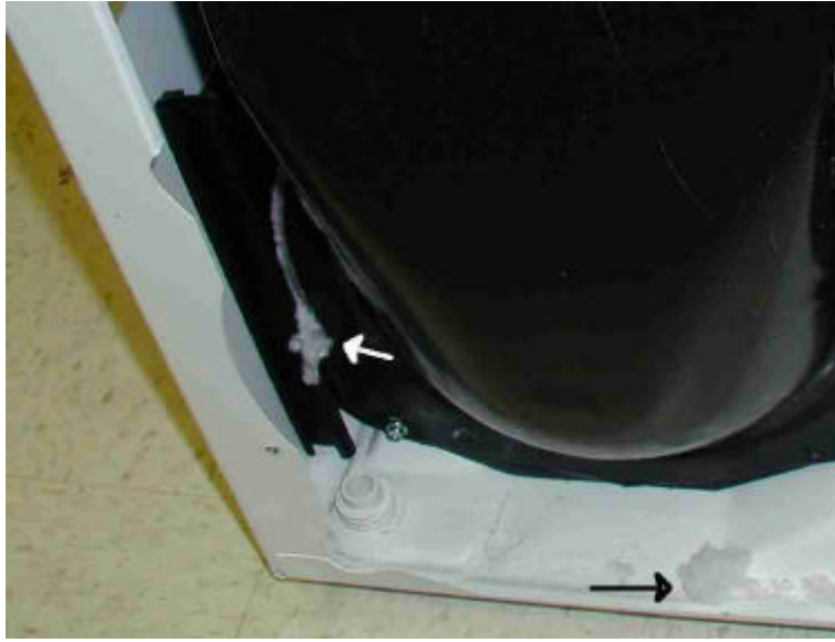
Figure 50. Lint Build-up at Blower Housing Seal and Dryer Floor
