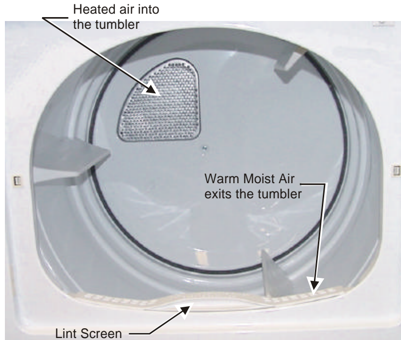
Figure 18. Dryer Design B – Air Flow Through the Tumbler
