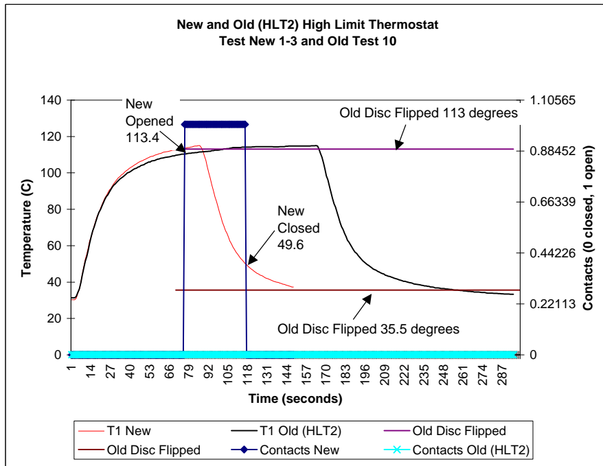
Figure 112. Comparison between New and Failed High Limit Thermostats
