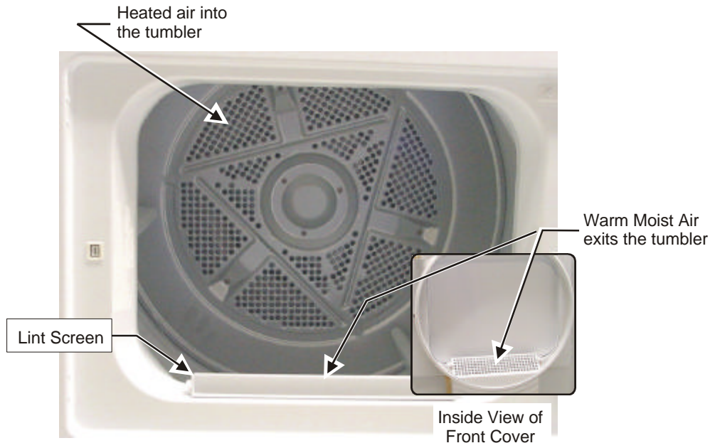
Figure 36. Dryer Design D – Airflow Through the Tumbler
