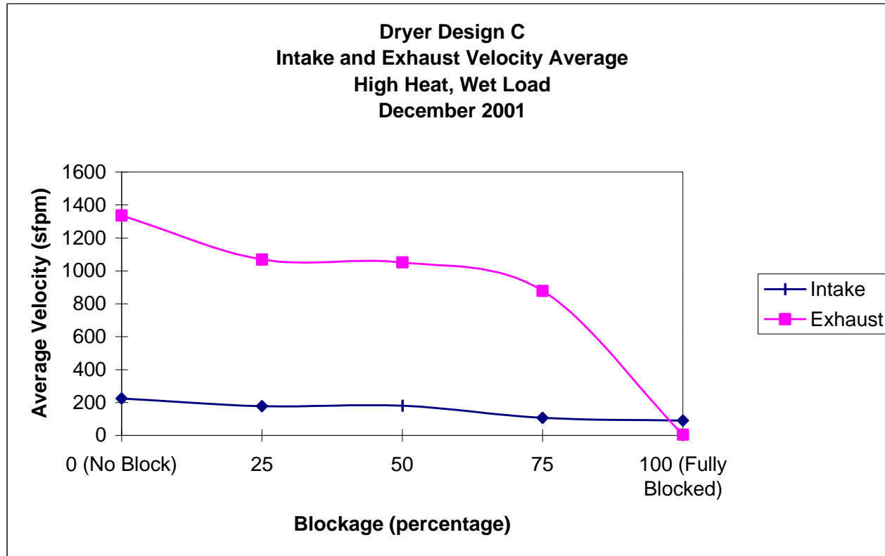
Figure 34. Dryer Design C – Average Airflow Velocities (High Heat and Wet Load)
