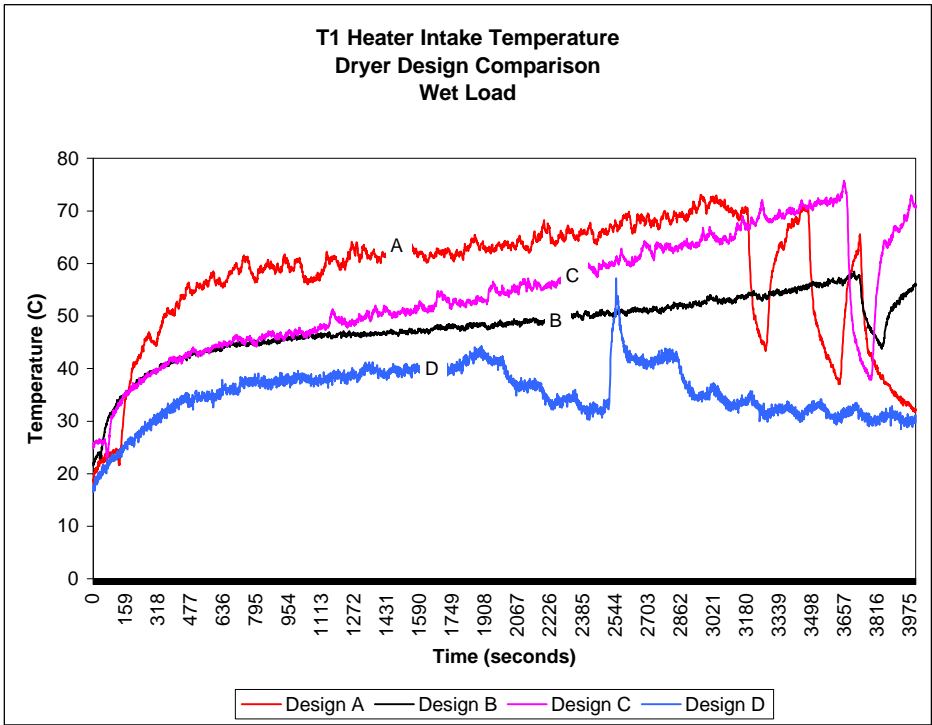
Figure 71. Dryer Design Comparison for T1, Heater Intake
