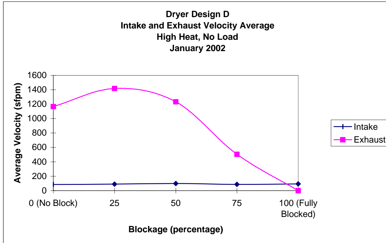
Figure 44. Dryer Design D –Average Airflow Velocities (High Heat and No Load)
