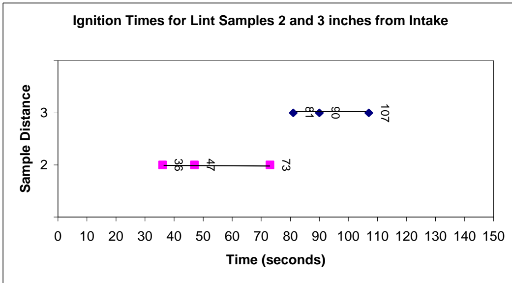
Figure 93. Ignition Time for 2 and 3 Inches from Heater Edge
