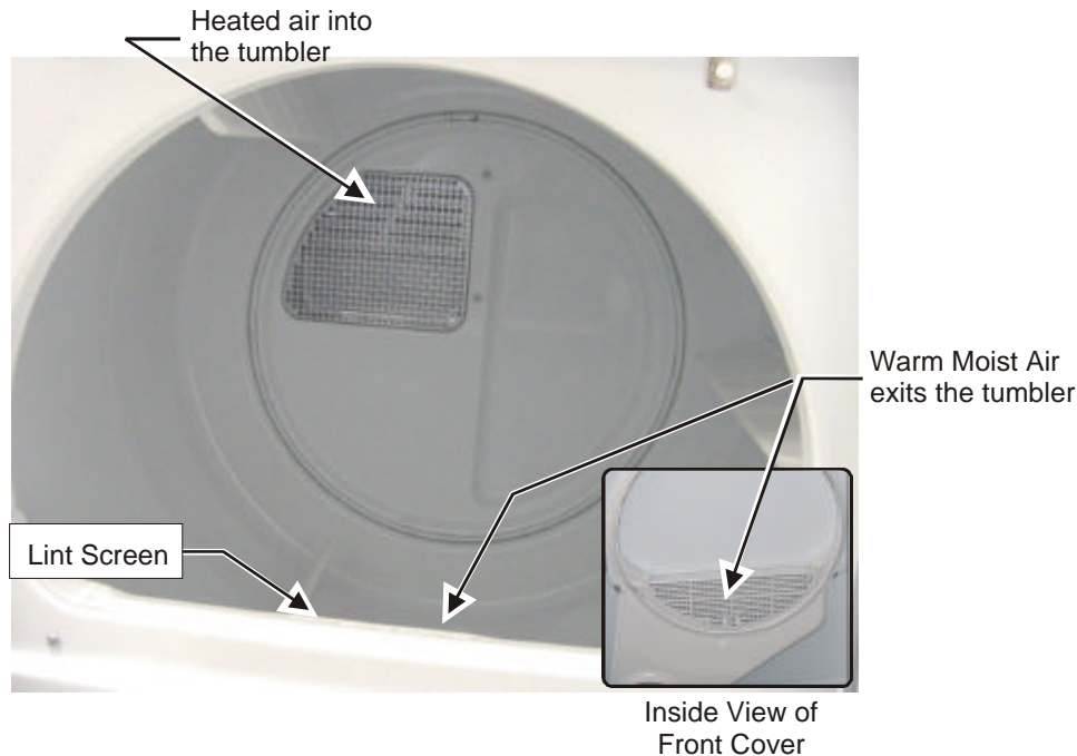
Figure 27. Dryer Design C – Airflow through the Tumbler
