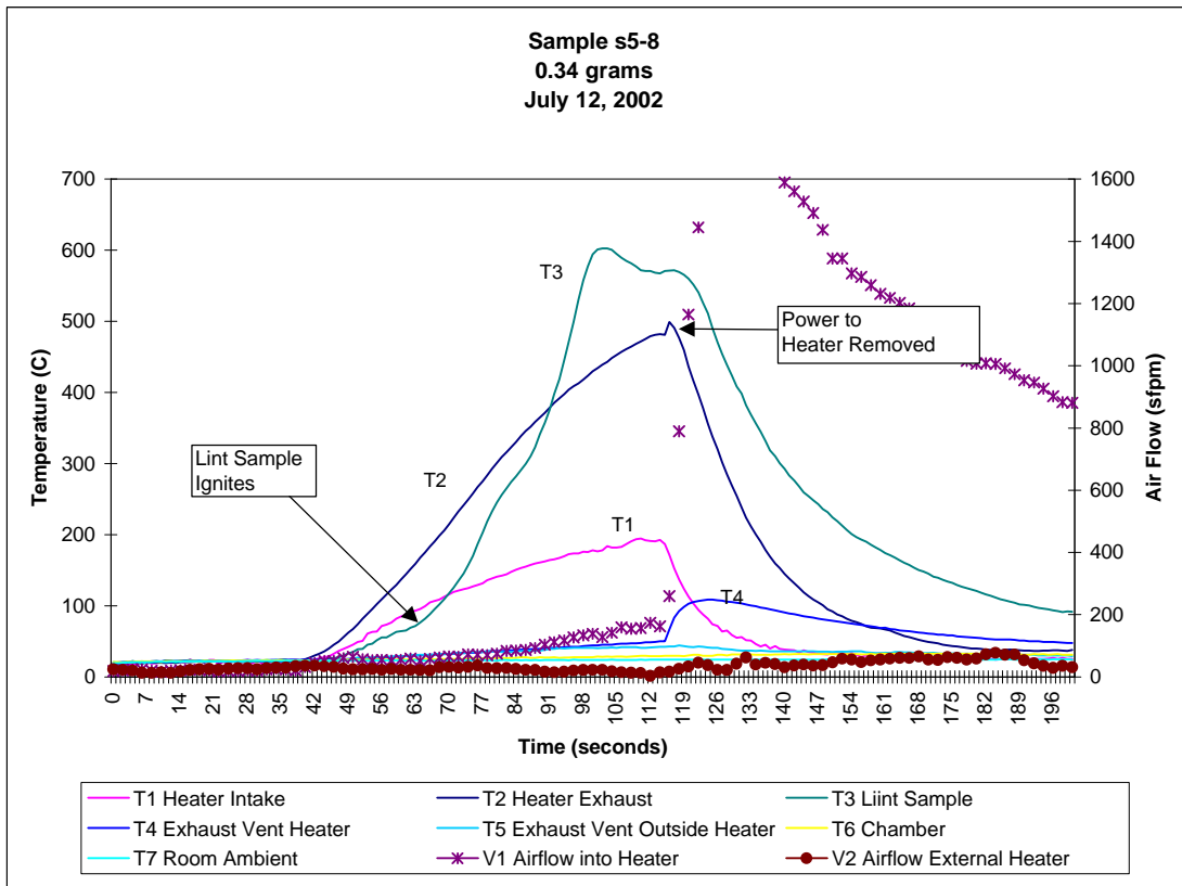
Figure 57. Thermocouple Data for Sample s5-8
