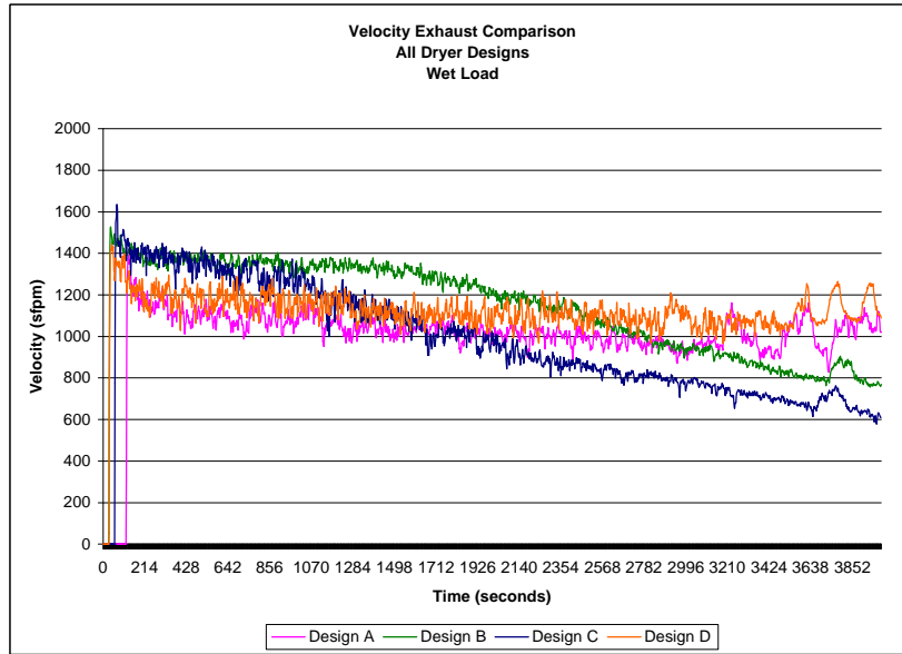
Figure 83. Comparison of Exhaust Air Velocity for all Dryer Designs
