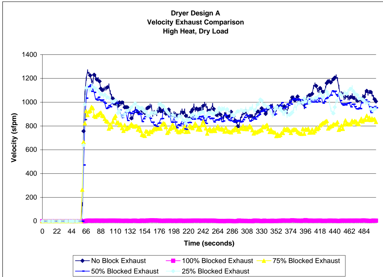
Figure 14. Dryer Design A – Exhaust Air Velocity
