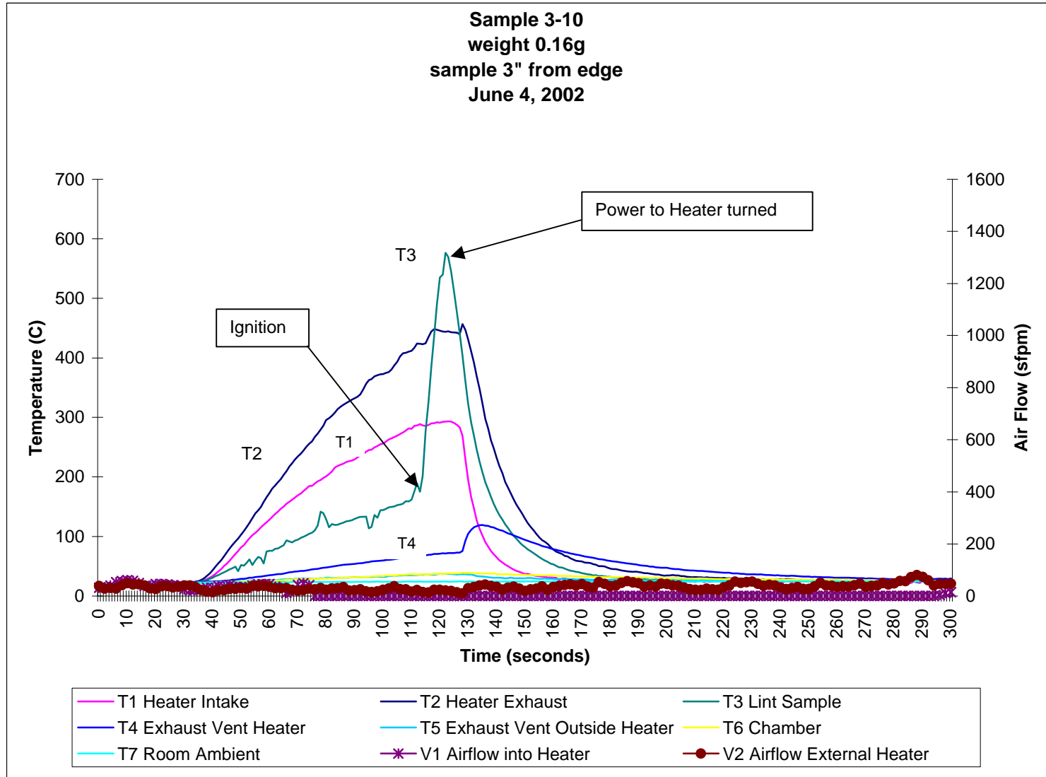
Figure 66. Sample s3-10 – Thermocouple and Airflow Data
