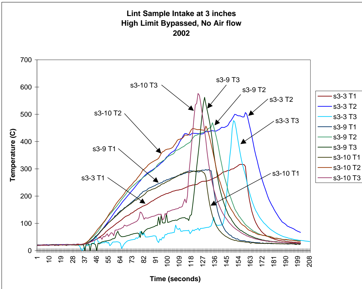
Figure 88. Lint Samples Tested 3 Inches from the Heater Housing Edge
