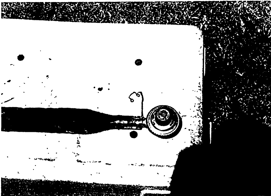
PHOTOGRAPH 26: One solution to the detachment problem: Seen here is a domestically made competitor's model. There are two differences between this unit and the subject grill: (1): The gas control connects directly to the burner without first going through a tube. (2): The assembly is provided with a locking device.
