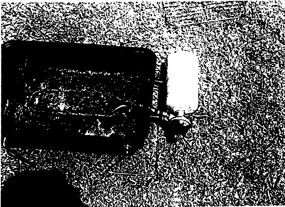
PHOTOGRAPH 14: Sequence of events: When the burner tube fell out of the grill burner and slid to the position seen here (and in Photograph 12), the burner tube hit the side of the hole in the metal housing and stayed there for a moment before falling completely out.
