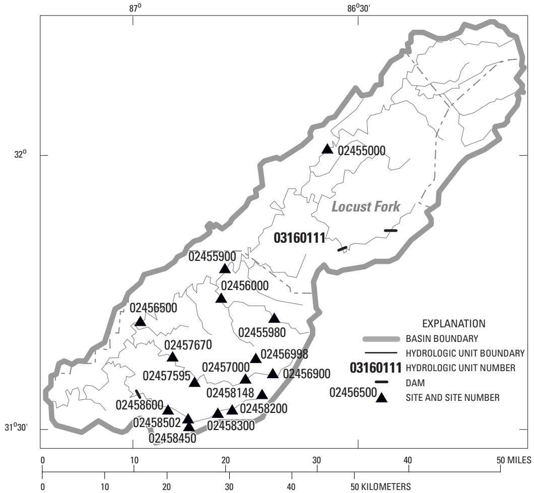
Figure 12. Location of surface-water stations in Locust Fork River basin.
