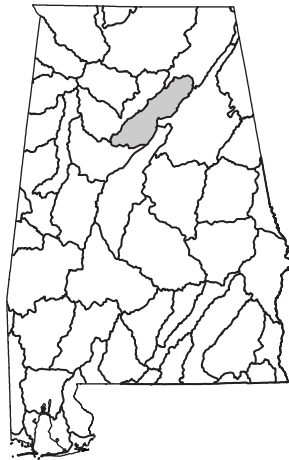
LOCATION OF SELECTED HYDROLOGIC UNITS IN ALABAMA
