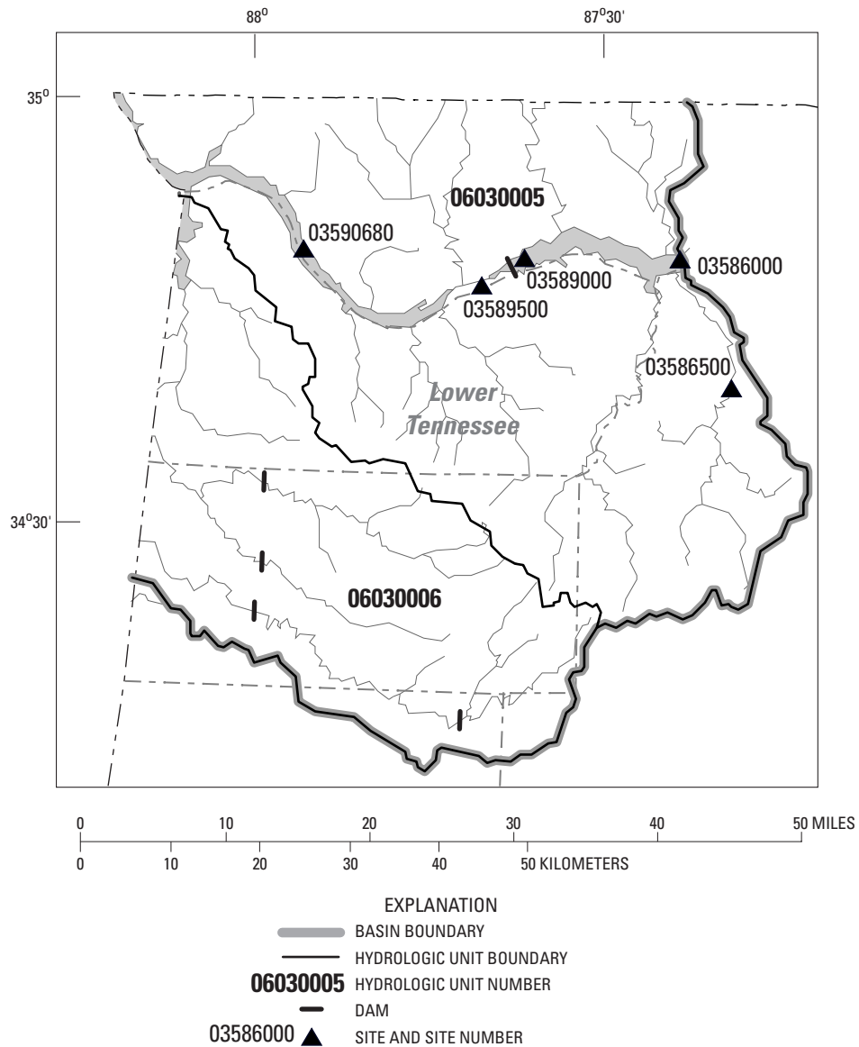
Figure 19. Location of surface-water stations in Lower Tennessee River basin.
