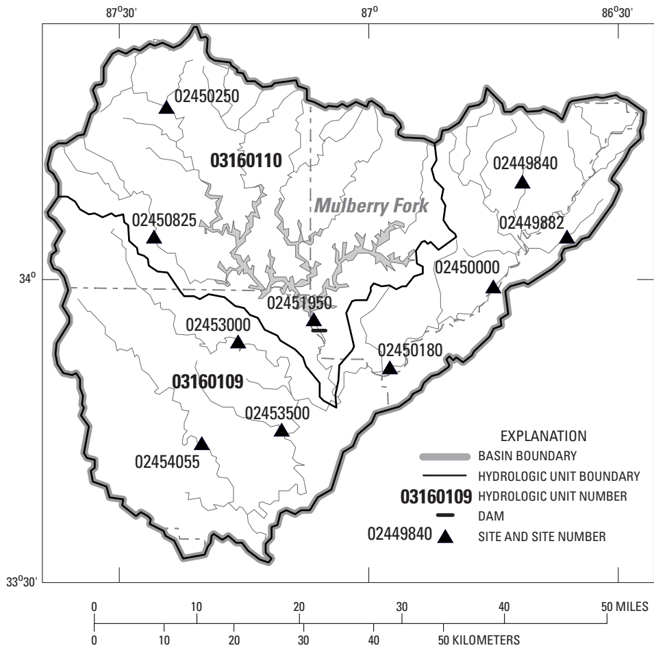
Figure 11. Location of surface-water stations in Mulberry Fork River basin.
