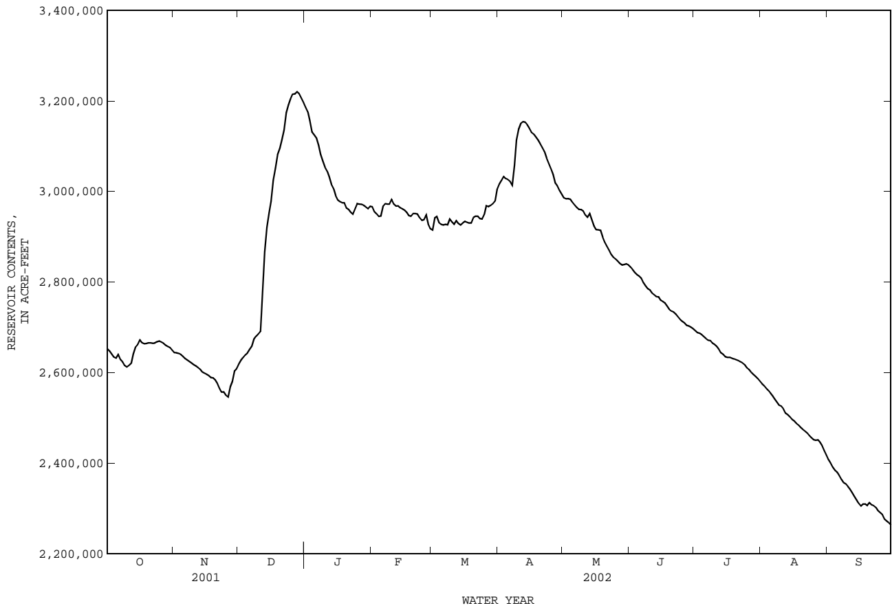
08039300 Sam Rayburn Reservoir near Jasper, TX--Continued
