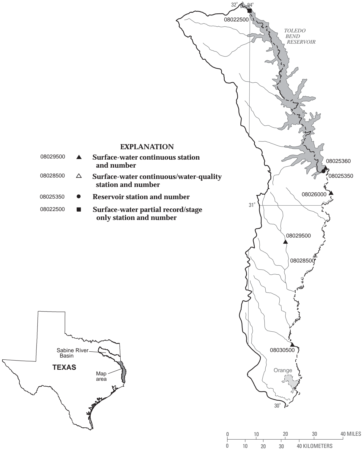
Figure 9.--Map showing location of gaging stations in the second section of the Sabine River Basin
