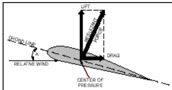
FIGURE 1.—Lift Vector.
