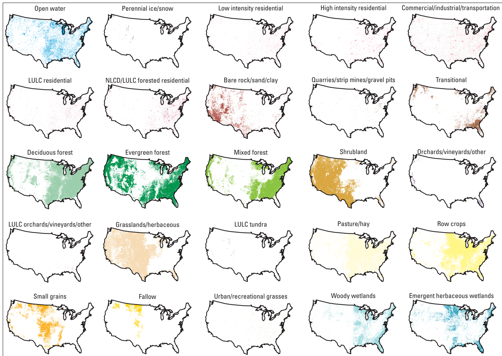
Figure 5. The complete set of 1-km resolution national grids of percentage land cover derived from the 30-m resolution “enhanced” National Land Cover Data 1992 (NLCDe 92). LULC, Land Use and Land Cover; NLCD, National Land Cover Data. These maps, with the exception of the map showing the “commercial/industrial/transportation” classification, were generated by coloring all grid cells where the percentage value of a land cover class (or grid cell value) is greater than or equal to 1. The map for the “commercial/industrial/transportation” classification was generated by coloring all grid cells where the percentage value of a land cover class is greater than or equal to 5.
