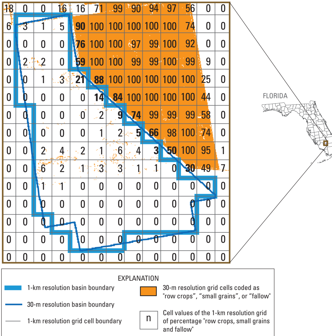
Figure 12. The 30-m and 1-km resolution drainage basin boundaries, distribution of 30-m resolution "row crops," "small grains," and "fallow" from the "enhanced" National Land Cover Data 1992 (NLCDe 92), and selected cell values of the 1-km resolution national grid of percentage "row crops, small grains, and fallow" in the vicinity of the drainage basin (Basin ID 02289034) for the U.S. Geological Survey's station U.S. Sugar Outflow Canal near Clewiston, Florida.
