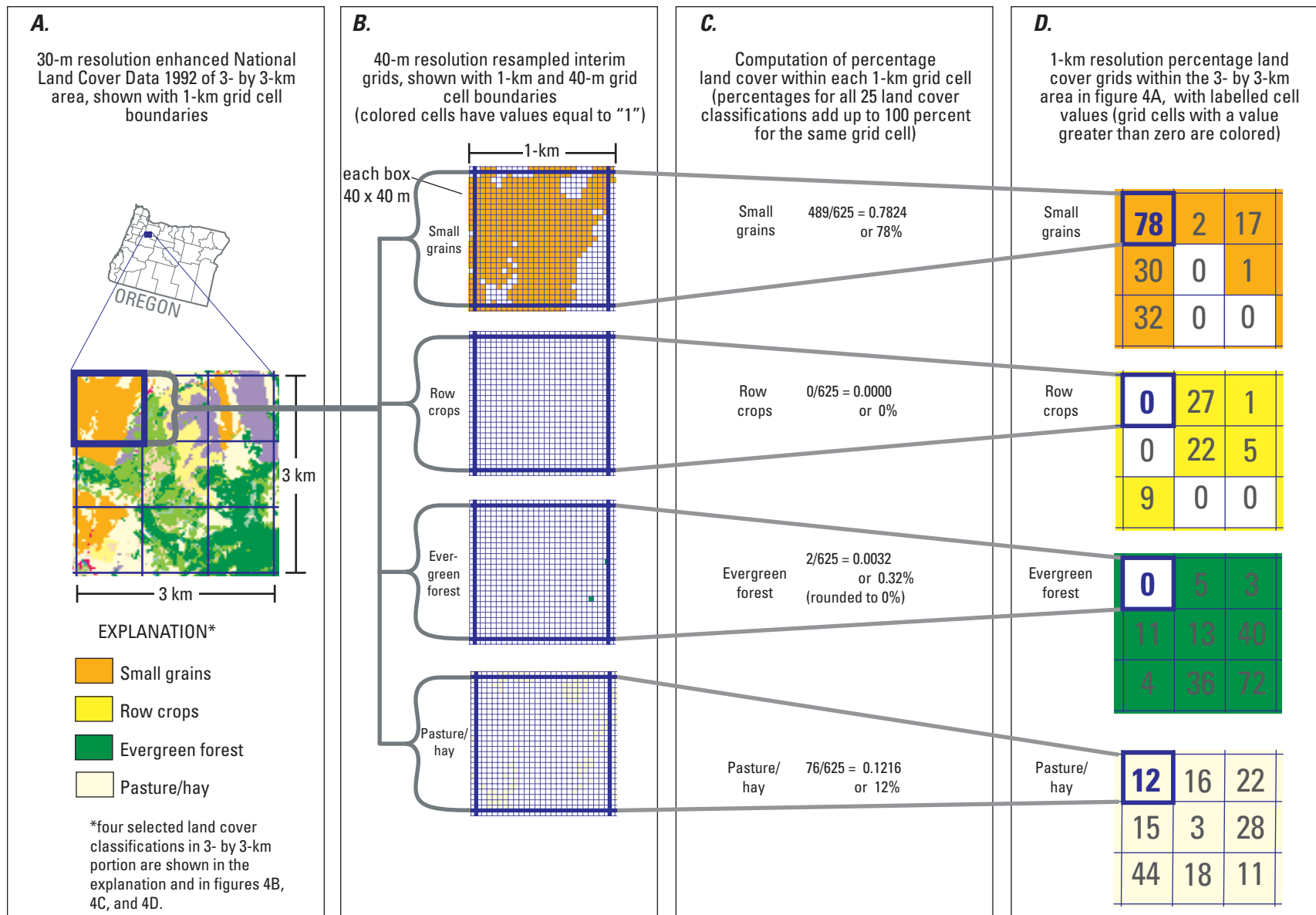
Figure 4. The process of creating 1-km resolution national grids of percentage land cover from the 30-m resolution "enhanced" National Land Cover Data 1992 (NLCDe 92) [15].
