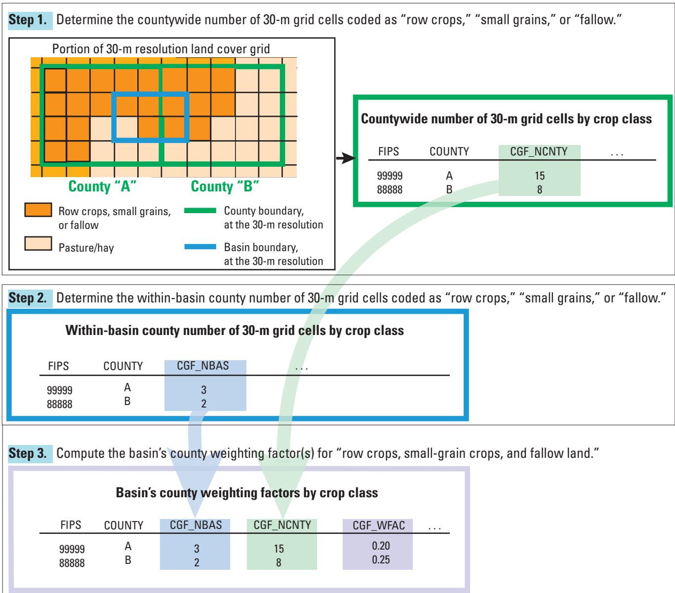
Figure 10. Steps to estimate 30-m resolution basin atrazine use on crops associated with the crop class “row crops, small-grain crops, and fallow land” (using fictitious data). A. Steps 1–3. B. Step 4, and C. Step 5. The 30-m basin atrazine estimates were derived from the 1992 county tabular file of atrazine use estimates by crop class and the 30-m resolution grids of the (1) “enhanced” National Land Cover Data 1992 (NLCDe 92), (2) 1990 county boundaries, and (3) drainage basin boundaries. FIPS stores the unique 5-digit numeric code for a county; COUNTY stores the name of the county; CGF_NCNTY stores the countywide number of 30-m grid cells classified as “row crops,” “small grains,” or “fallow”; CGF_NBAS stores the within-basin county number of 30-m grid cells that are classified as “row crops,” “small grains,” or “fallow”; CGF_WFAC stores the basin’s county weighting factor for the crop class, “row crops, small-grain crops, and fallow land”; CGF_KG in step 4 stores the estimated amount of atrazine in kilograms per county applied to crops associated with the crop class “row crops, small-grain crops, and fallow land”; CGF_APPKG stores the basin’s county apportioned atrazine use estimate on crops associated with the crop class “row crops, small-grain crops, and fallow land”; BASINID stores the basin’s unique identification number; BAS_CGFKG in step 5 is the basin’s estimate of atrazine use on crops associated with the crop class “row crops, small-grain crops, and fallow land.”
