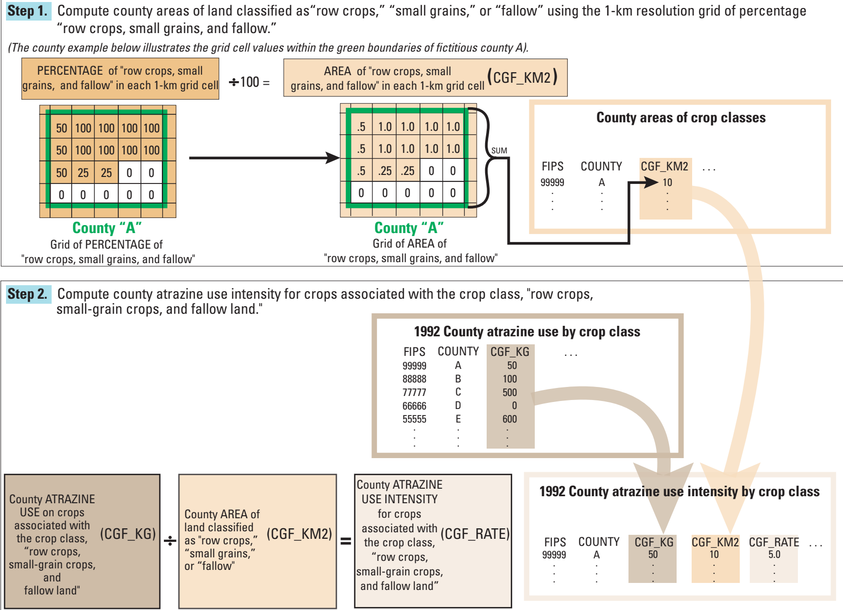
Figure 7. Steps to generate a 1-km resolution grid of estimated atrazine use on crops associated with the crop class "row crops, small-grain crops, and fallow land" (using fictitious data). A. Steps 1–2. B. Step 3. FIPS stores the unique 5-digit numeric code for a county; COUNTY stores the name of the county; CGF_KM2 stores the county area in square kilometers of land classified as "row crops," "small grains," or "fallow"; CGF_KG stores atrazine in kilograms per county applied to crops associated with the crop class "row crops, small-grain crops, and fallow land"; CGF_RATE contains the county rate of application of atrazine or atrazine use intensity on crops associated with the crop class "row crops, small-grain crops, and fallow land."
