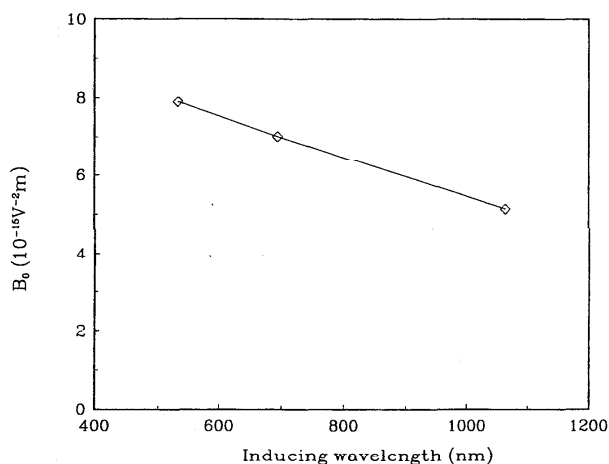
FIG. 1. The wavelength dispersion of B_0 for benzene with inducing beam wavelength. Data taken from Refs. 4 and 18.
