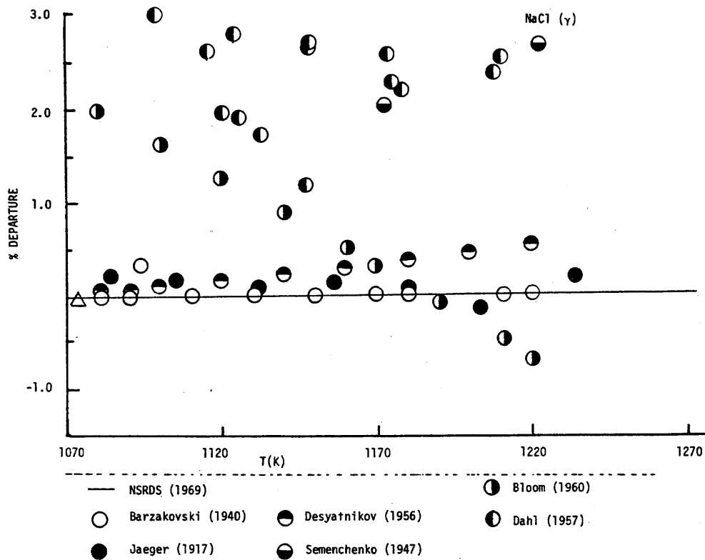
Figure 21 NaCl surface tension data for the period 1917-1960, shown as a percent departure analysis with the 1969 NSRDS recommended data base (Sokolova, Voskrenenskaya [1962]) as comparison standard.
