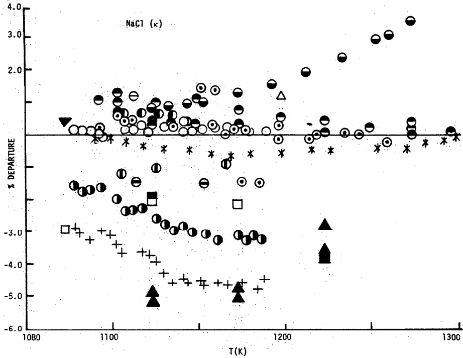
Figure 24 NaCl conductance data for the period 1960-1979, shown as a percent departure analysis with Emons and Brautigam data base (1976) as comparison standard.
