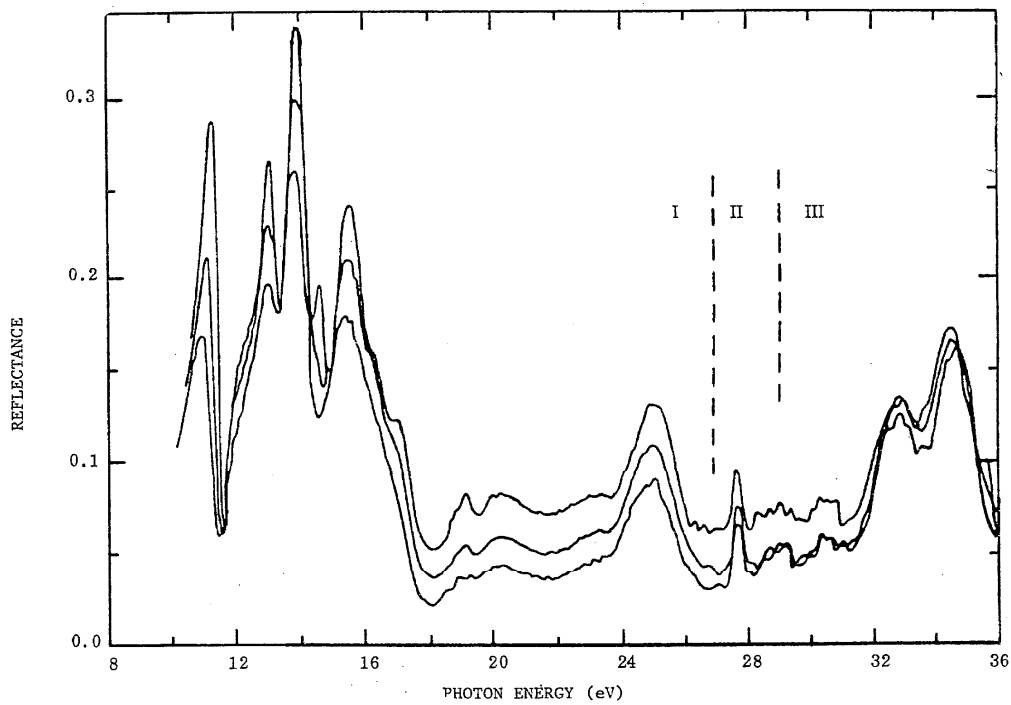
Figure 4. Near-Normal Incidence ( \approx 6^\circ ) Reflectance Spectrum of CaF 2 Crystal in the Far Ultraviolet [24].
