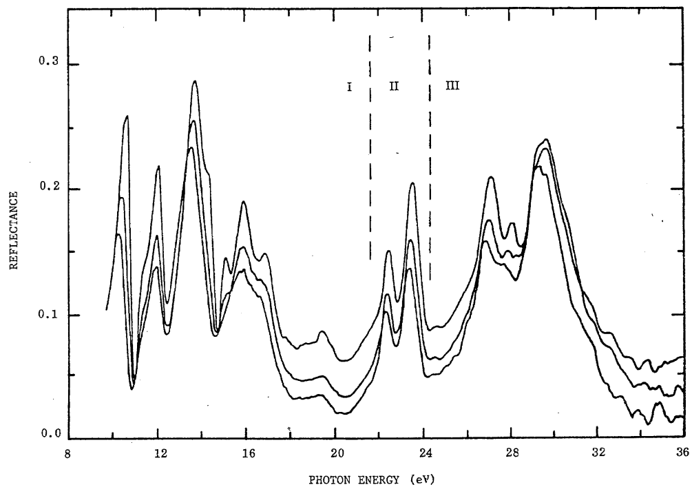
Figure 5. Near-Normal Incidence ( \approx 6^\circ ) Reflectance Spectrum of SrF 2 Crystal in the Far Ultraviolet [24].
