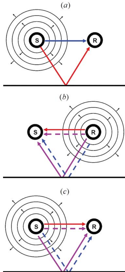
Fig. 6. Pictorial demonstration of two different implementations of Time Reversal (TR): (a) source emission, (b) standard TR and (c) reciprocal TR. Colors correspond to those found in Fig. 5. The solid lines correspond to the first emission of energy (red colored pulse in Fig 5c), while the dashed lines correspond to the second emission of energy (blue colored pulse in Fig 5c).
