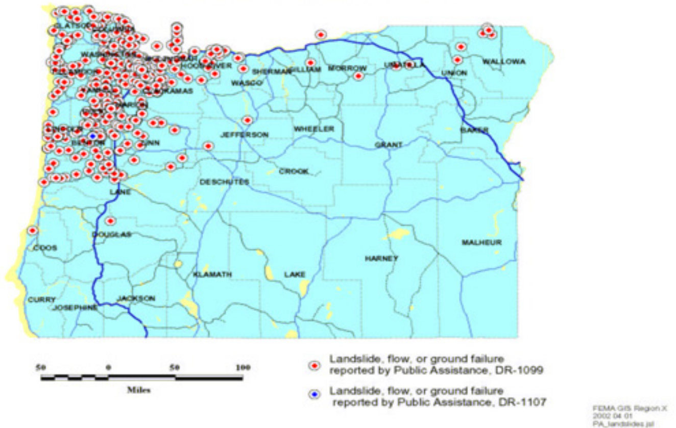
Figure 7. FEMA map showing probable landslides from two declared disasters, FEMA-DR-1107-OR and FEMA-DR-1099-OR. Source: FEMA
