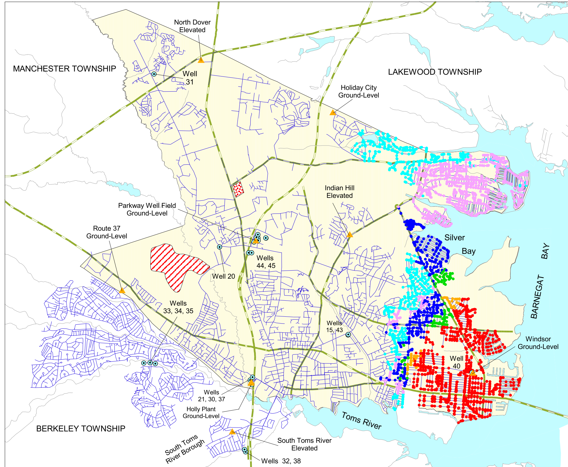
PLATE 22. AREAL DISTRIBUTION OF SIMULATED PROPORTIONATE CONTRIBUTION OF WATER FROM THE WINDSOR GROUND-LEVEL STORAGE TANK TO LOCATIONS IN THE DOVER TOWNSHIP AREA, NEW JERSEY AUGUST 1998 CONDITIONS By Morris L. Maslia, Jason B. Sautner, and Mustafa M. Aral
