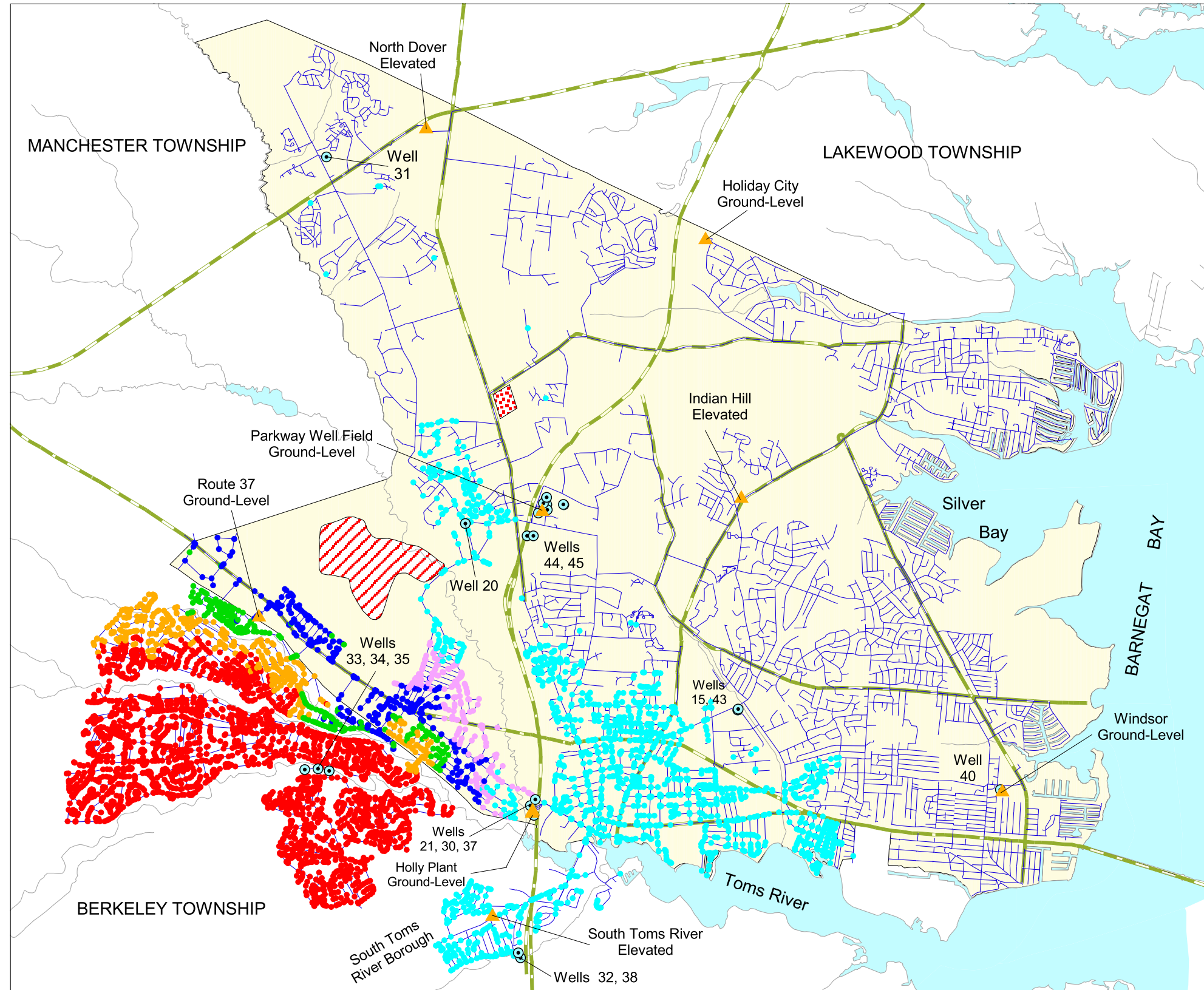
PLATE 17. AREAL DISTRIBUTION OF SIMULATED PROPORTIONATE CONTRIBUTION OF WATER FROM THE BERKELEY WELLS (33, 34, 35) TO LOCATIONS IN THE DOVER TOWNSHIP AREA, NEW JERSEY AUGUST 1998 CONDITIONS By Morris L. Maslia, Jason B. Sautner, and Mustafa M. Aral
