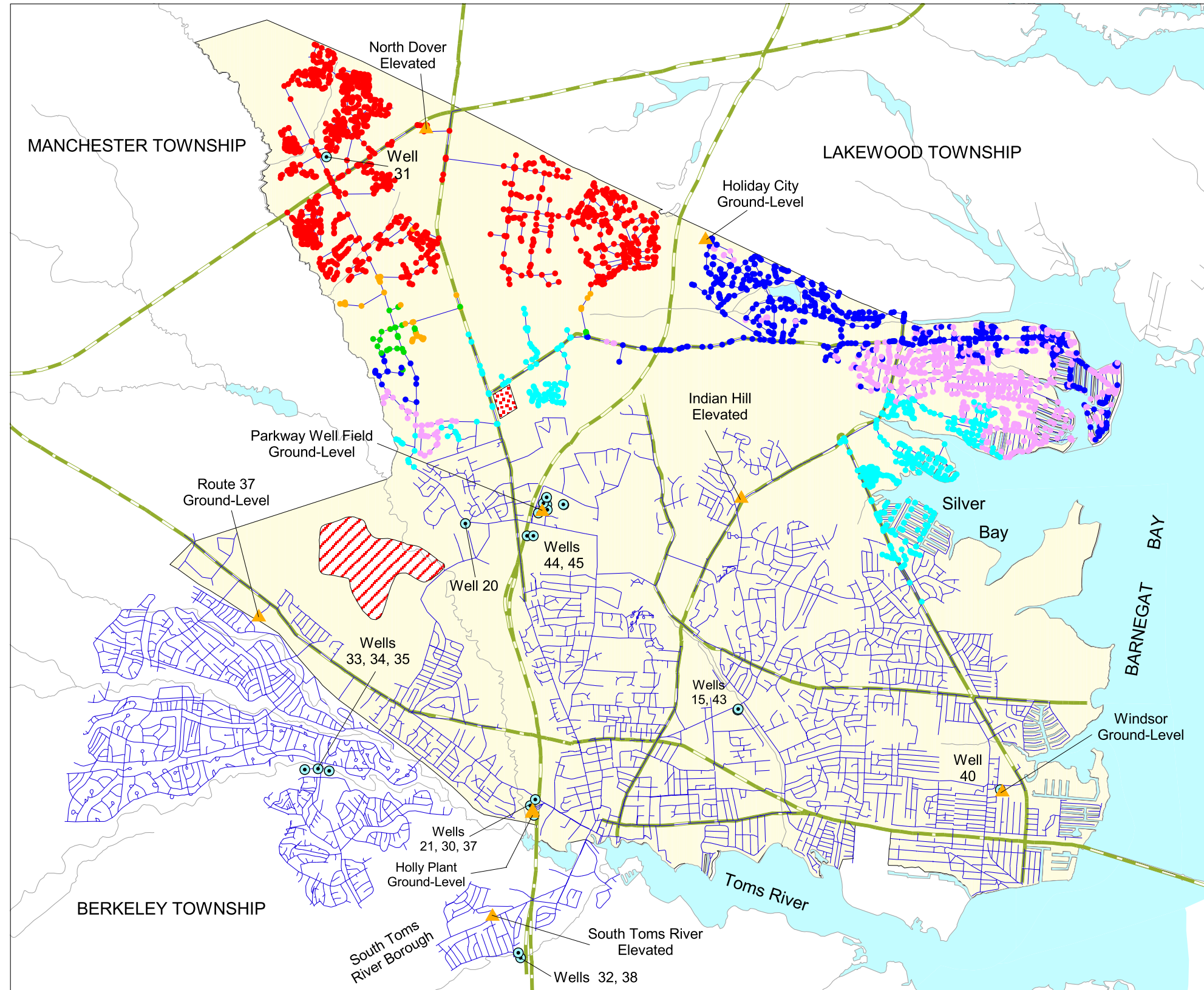
PLATE 15. AREAL DISTRIBUTION OF SIMULATED PROPORTIONATE CONTRIBUTION OF WATER FROM THE ROUTE 70 WELL (31) TO LOCATIONS IN THE DOVER TOWNSHIP AREA, NEW JERSEY MARCH 1998 CONDITIONS By Morris L. Maslia, Jason B. Sautner, and Mustafa M. Aral
