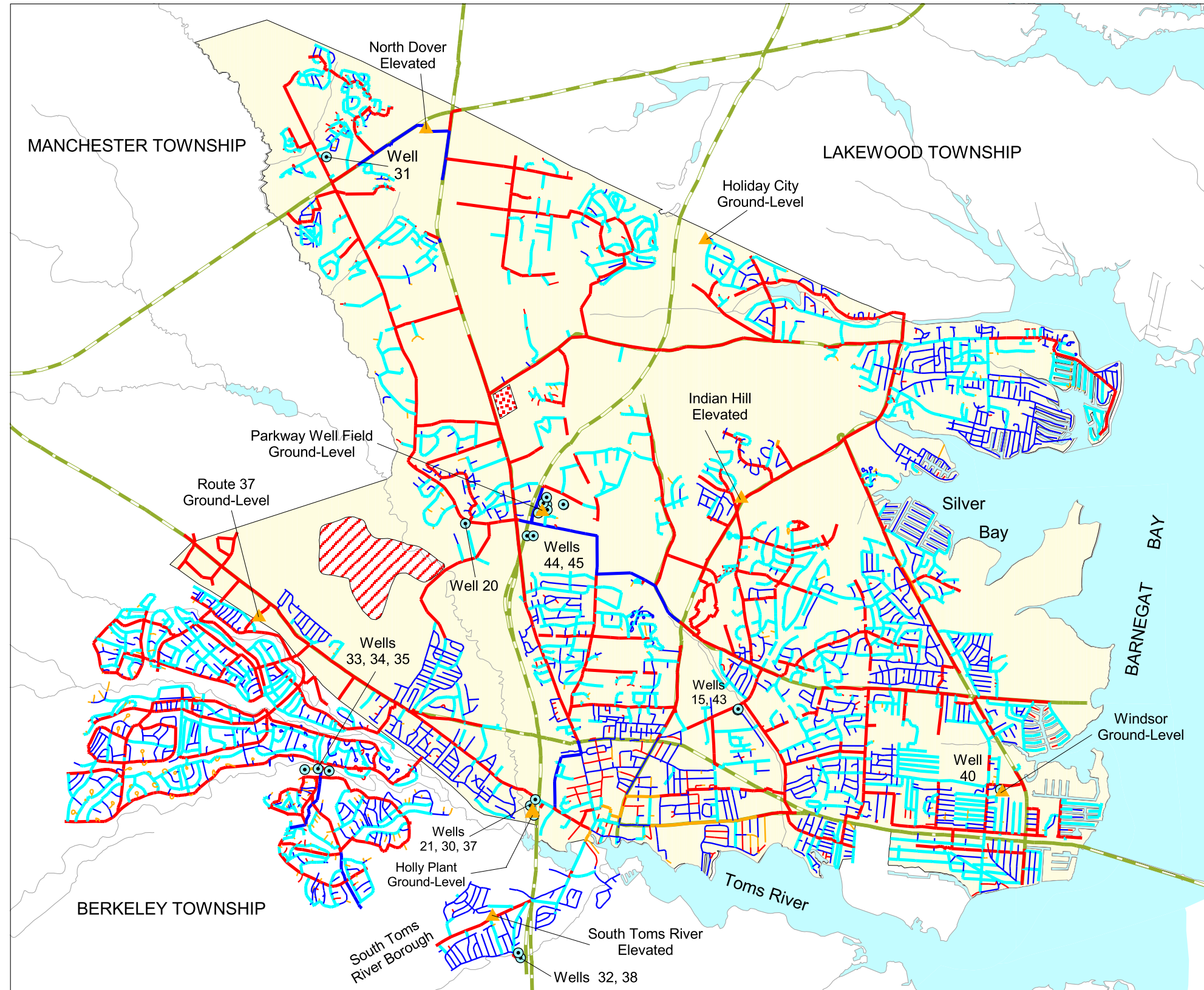
PLATE 8. DISTRIBUTION OF PIPELINE DIAMETERS USED TO MODEL THE 1998 WATER-DISTRIBUTION SYSTEM SERVING THE DOVER TOWNSHIP AREA, NEW JERSEY
