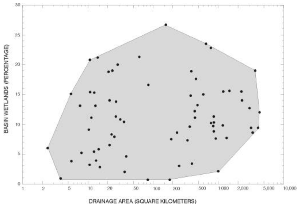
Figure 3. Two-dimensional range of explanatory variables for the full regression equations.
