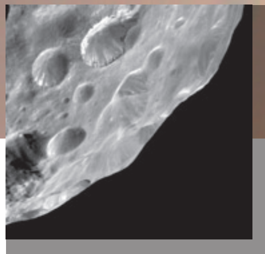
An image of part of Saturn's small icy moon Phoebe, taken as the Cassini spacecraft flew by, shows many craters.
