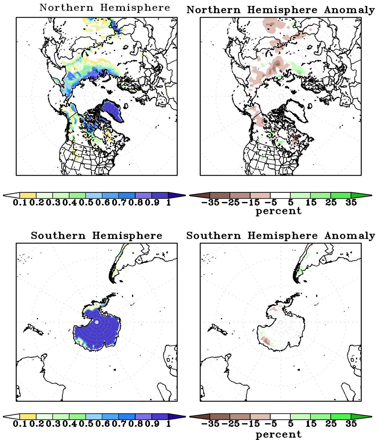
FIGURE A2.2. SSM/I derived snow cover frequency (%) (left) and snow cover anomaly (%) (right) for the month of MAY 2008 based on 1987 - 2006 base period for the Northern Hemisphere (top) and Southern Hemisphere (bottom). It is generated using the algorithm described by Ferraro et. al, 1996, Bull. Amer. Meteor. Soc., vol 77, 891-905.
