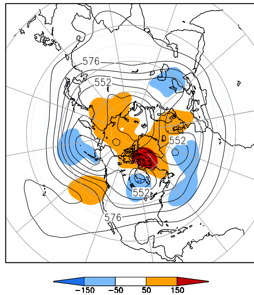
500-hPa Height (dm) & Anomalies (m) (May 1–15, 2008)
