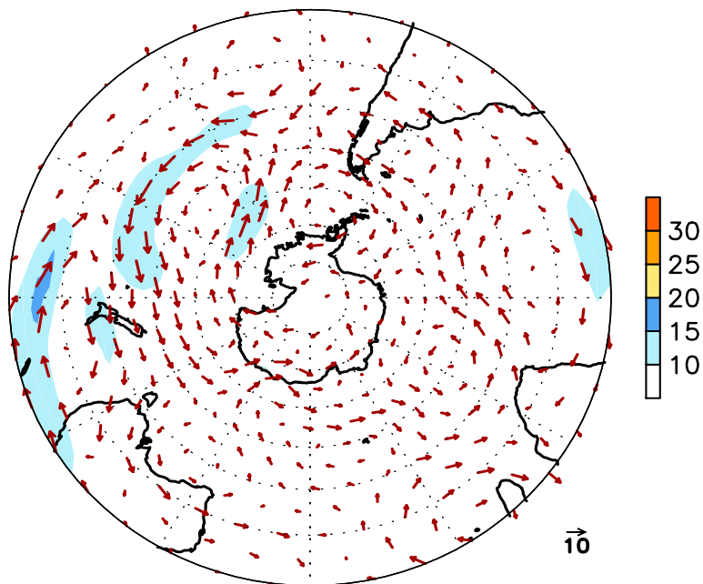
FIGURE E16. Southern Hemisphere mean (left) and anomalous (right) 300-hPa vector wind (CDAS/Reanalysis) for MAY 2008. Mean (anomaly) isotach contour interval is 10 (5) \text{ms}^{-1} . Values greater than 30 \text{ms}^{-1} (left) and 10 \text{ms}^{-1} (rights) are shaded. Anomalies are departures from the 1979-95 base period monthly means.
