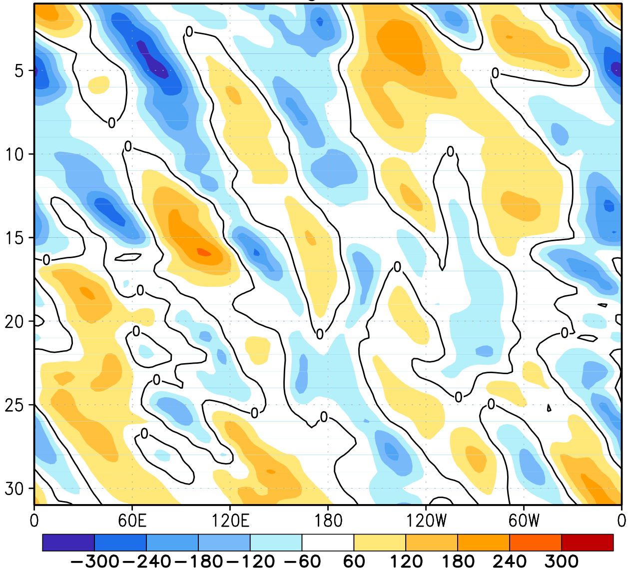
FIGURE E18. Southern Hemisphere: Daily 500-hPa height anomalies for MAY 2008 averaged over the 5° latitude band centered on 40°S. Positive values are indicated by solid contours and dark shading. Negative values are indicated by dashed contours and light shading. Contour interval is 60 m. Anomalies are departures from the 1979-95 base period daily means.
