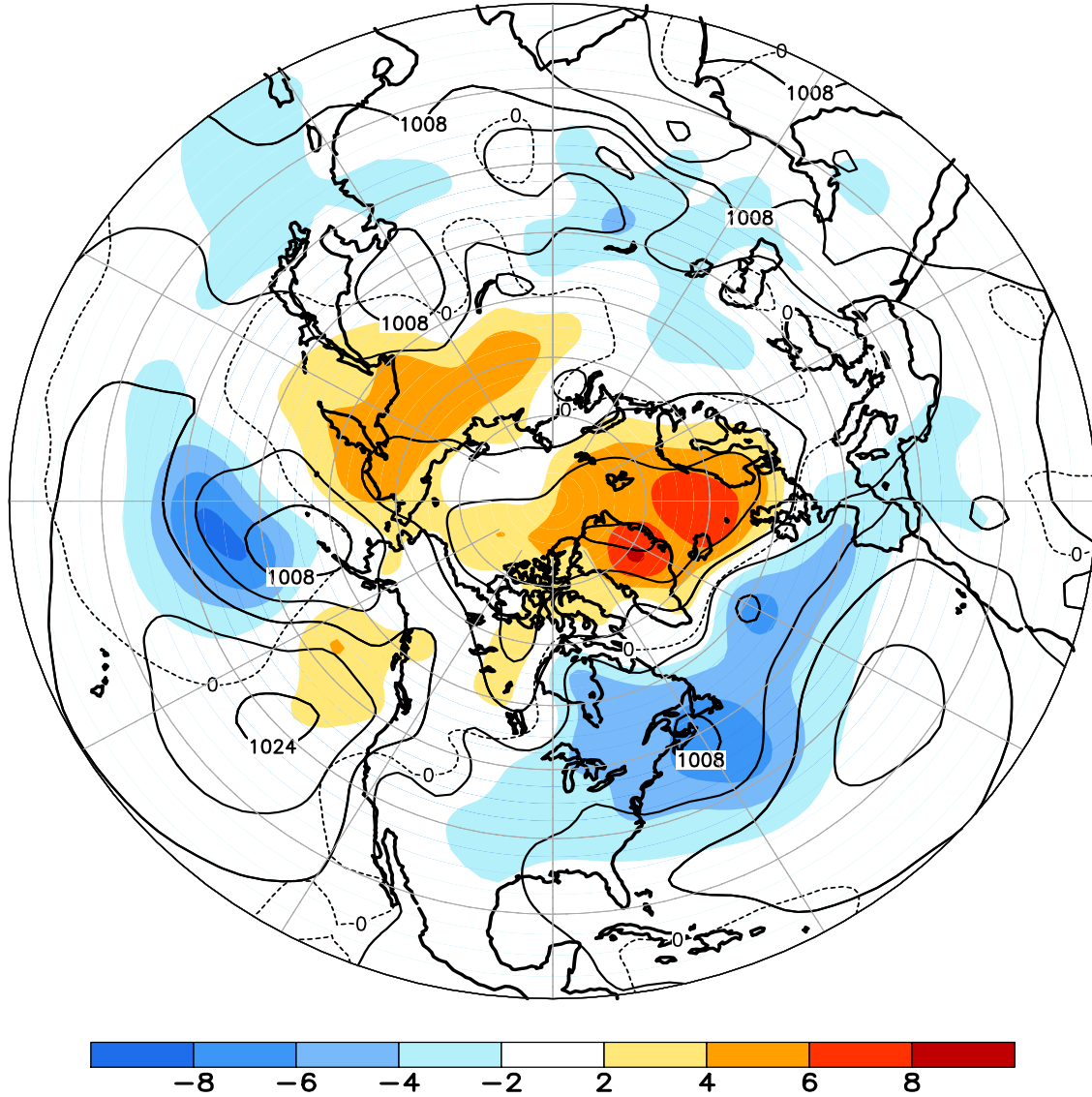
FIGURE E8. Northern Hemisphere mean and anomalous sea level pressure (CDAS/Reanalysis) for MAY 2008. Mean values are denoted by solid contours drawn at an interval of 4 hPa. Anomaly contour interval is 2 hPa with values less (greater) than -2 hPa (2 hPa) indicated by dark (light) shading. Anomalies are calculated as departures from the 1979-95 base period monthly means.
