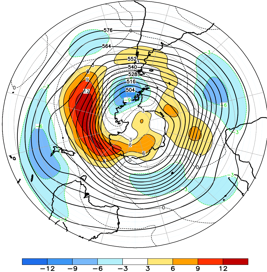
FIGURE E15. Southern Hemisphere mean and anomalous 500-hPa geopotential height (CDAS/Reanalysis) for MAY 2008. Mean heights are denoted by solid contours drawn at an interval of 6 dam. Anomaly contour interval is 3 dam with values less (greater) than -3 dam (3 dam) indicated by dark (light) shading. Anomalies are calculated as departures from the 1979-95 base period monthly means.
