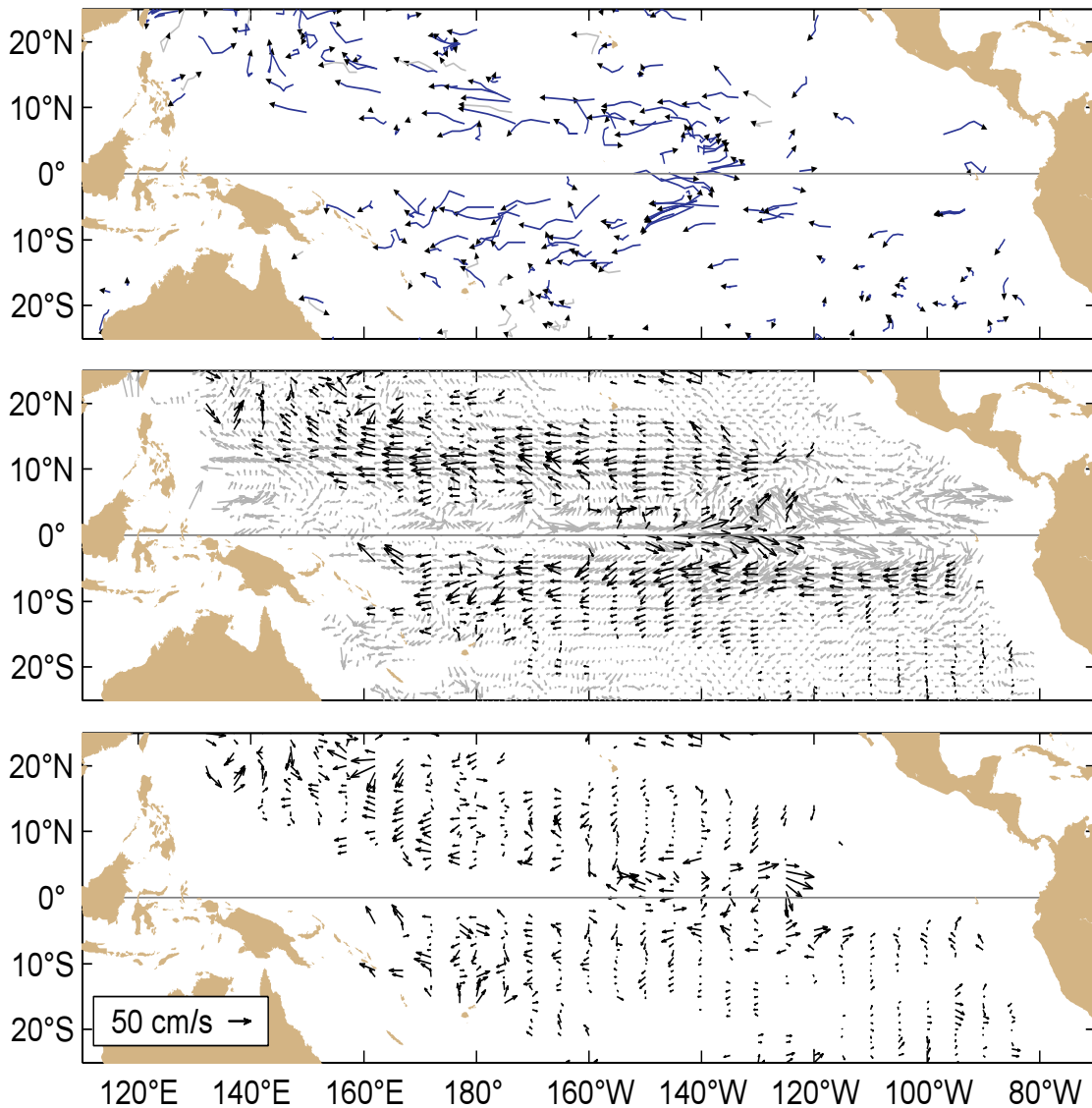
Figure A1.1 Top: Movements of drifting buoys in the tropical Pacific Ocean during May2008. The linear segments of each trajectory represent a one week displacement. Trajectories of buoys which have lost their subsurface drogues are gray; those with drogues are black.
