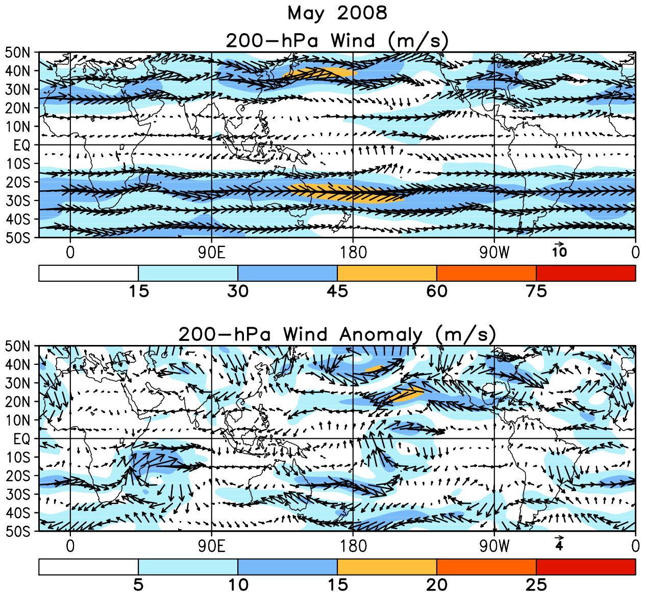
FIGURE T21. Mean (top) and anomalous (bottom) 200-hPa vector wind (CDAS/Reanalysis) for MAY 2008. Contour interval for isotachs is 15 \text{ ms}^{-1} (top) and 5 \text{ ms}^{-1} (bottom). Anomalies are departures from 1979–95 base period monthly means.
