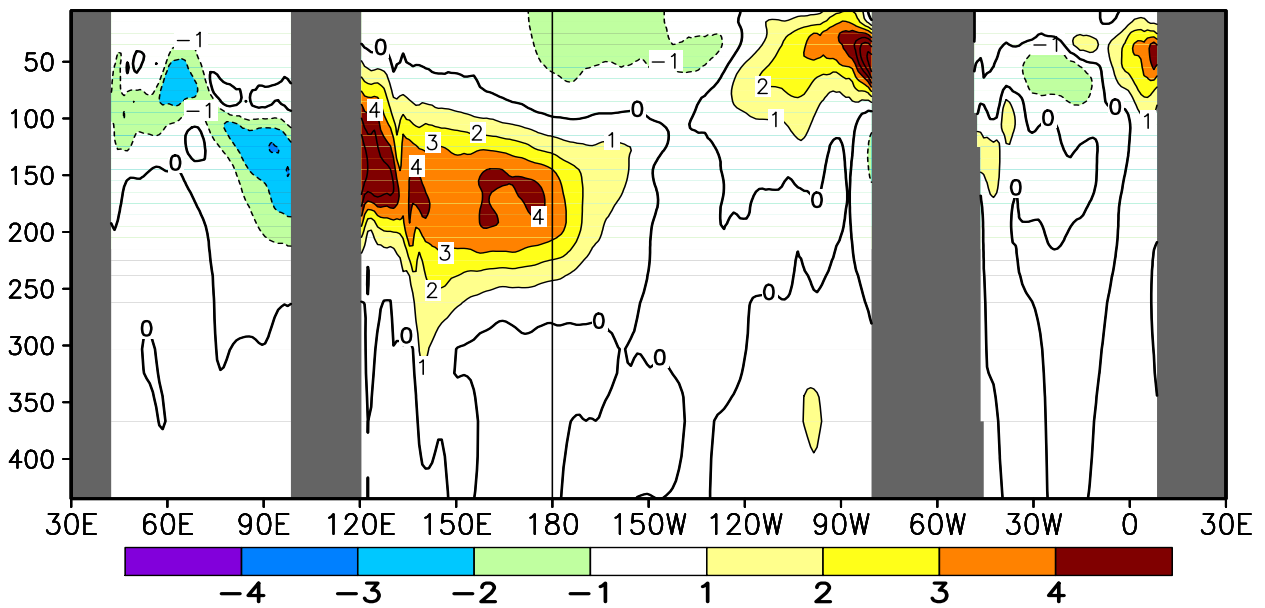
FIGURE T17. Equatorial depth–longitude section of ocean temperature (top) and ocean temperature anomalies (bottom) for MAY 2008. Contour interval is 1°C. Dashed contours in bottom panel indicate negative anomalies. Data are derived from the NCEP’s global ocean data assimilation system version 2 which assimilates oceanic observations into an oceanic GCM (Xue, Y. and Behringer, D.W., 2006: Operational global ocean data assimilation system at NCEP, to be submitted to BAMS). Anomalies are departures from the 1982–2004 base period means.
