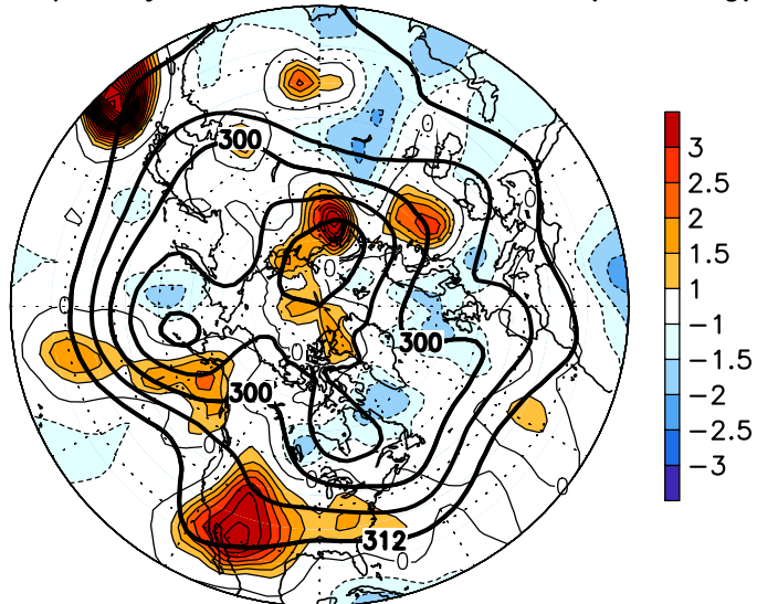
FIGURE E13. Northern Hemisphere: 700-hPa heights for MAY 2008 overlaid with standard deviation of high-pass filtered height (left) and normalized anomalous variance of high-pass filtered height (right). Heights are indicated by thick solid contours in both panels (interval is 60 m). High-pass filtered fields reflect fluctuations having periods less than 10 days, and are indicated by thin contours and shading. Contour interval for standard deviation is 15 m with values > 45 m shaded. Contour interval for normalized variance is 1 standard deviation, with positive values shown by solid contours and dark shading and negative values shown by dashed contours and light shading. Anomalies are departures from the 1964-93 base period monthly means.
