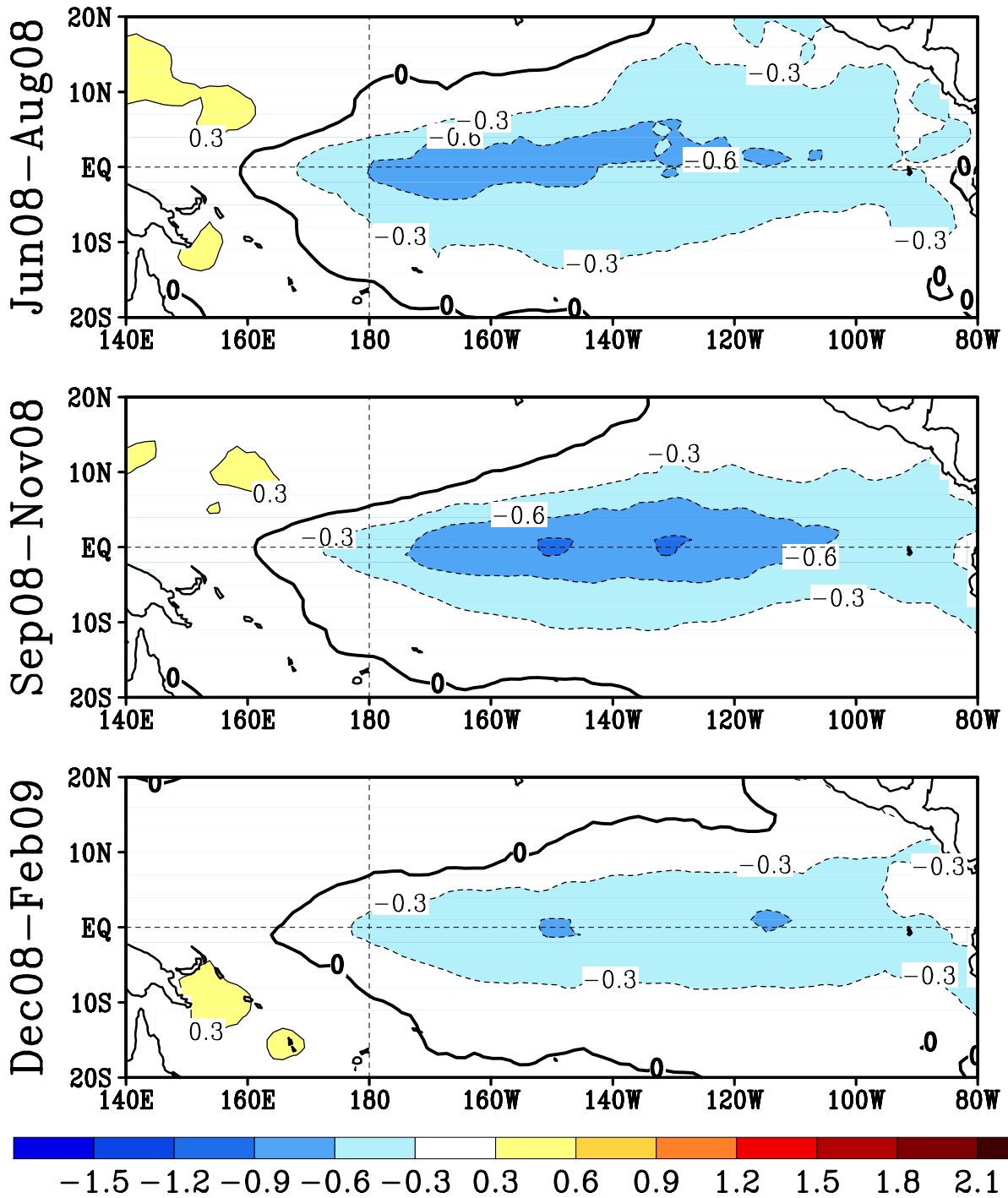
FIGURE F5. Predicted 3-month average sea surface temperature anomalies from the NCEP/CPC Markov model (Xue et al. 2000, J. Climate , 13 , 849-871). The forecast is initiated in MAY 2008 . Contour interval is 0.3C and negative anomalies are indicated by dashed contours. Anomalies are calculated relative to the 1971-2000 climatology.
