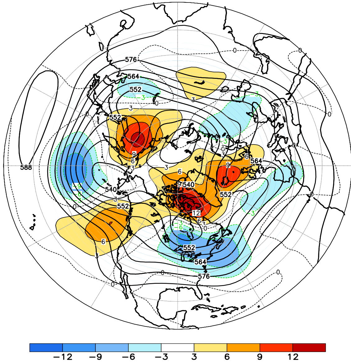
FIGURE E9. Northern Hemisphere mean and anomalous 500-hPa geopotential height (CDAS/Reanalysis) for MAY 2008. Mean heights are denoted by solid contours drawn at an interval of 6 dam. Anomaly contour interval is 3 dam with values less (greater) than -3 dam (3 dam) indicated by dark (light) shading. Anomalies are calculated as departures from the 1979-95 base period monthly means.
