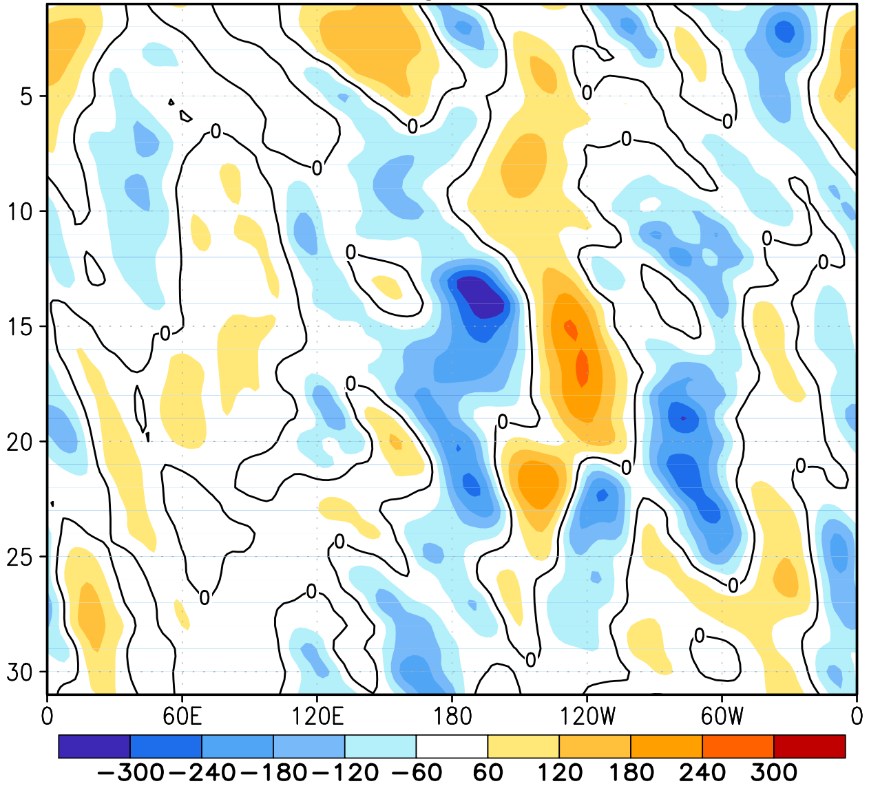
FIGURE E12. Northern Hemisphere: Daily 500-hPa height anomalies for MAY 2008 averaged over the 5° latitude band centered on 40°N. Positive values are indicated by solid contours and dark shading. Negative values are indicated by dashed contours and light shading. Contour interval is 60 m. Anomalies are departures from the 1979-95 base period daily means.
