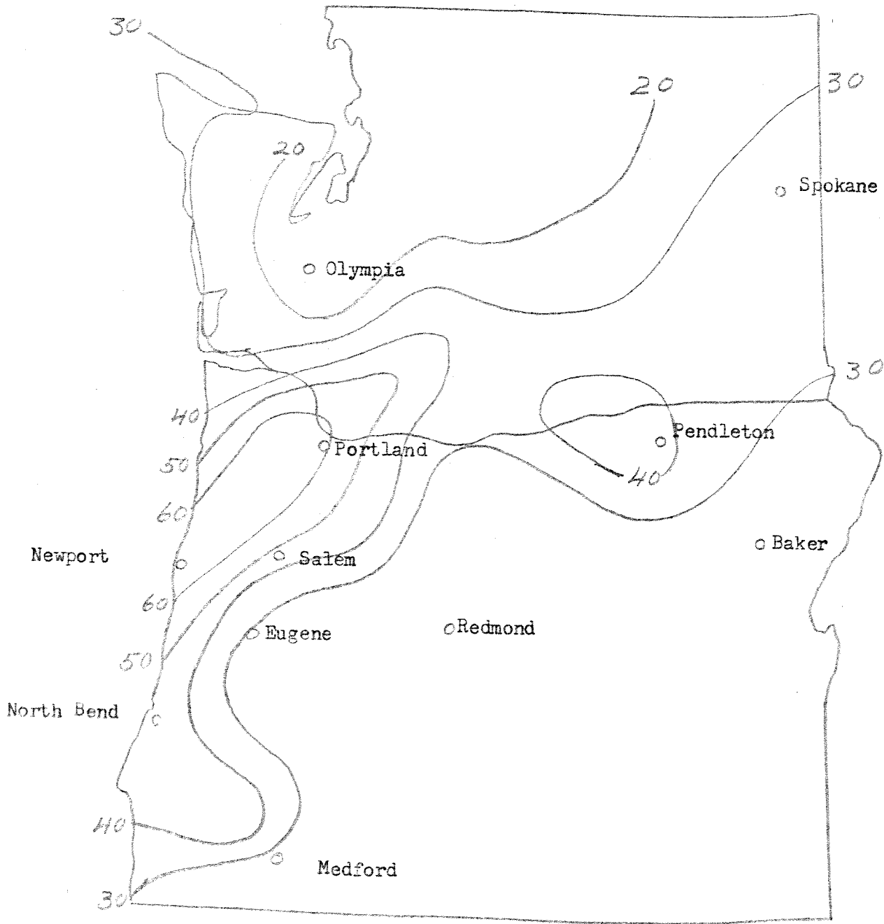
MAXIMUM TWO MINUTE WIND SPEEDS (mph) February 5, 1965
