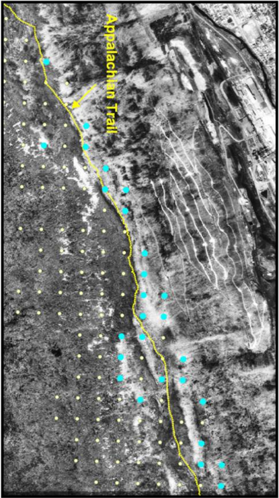
Aerial digital orthoquad showing the extent of the barren areas on Blue Mountain as of 1992. Sampling locations corresponding with mostly barren areas (light colored) are highlighted in blue.
