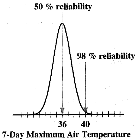
Figure III-1. Distribution of Annual Seven-Day Maximum Air Temperature for Topeka, KS
