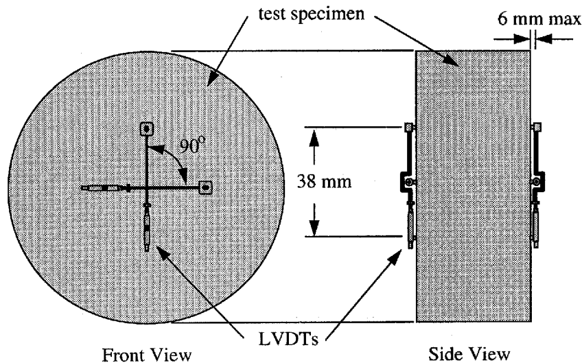
Figure VII-15. Specimen Instrumentation for IDT
