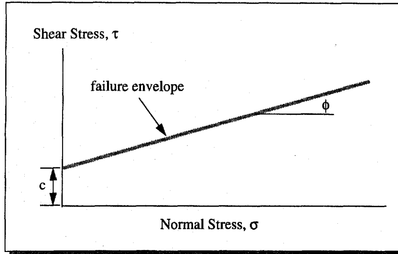
Figure I-6. Mohr-Coulomb Theory
