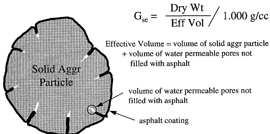
Figure IV-4. Effective Specific Gravity of Aggregate
