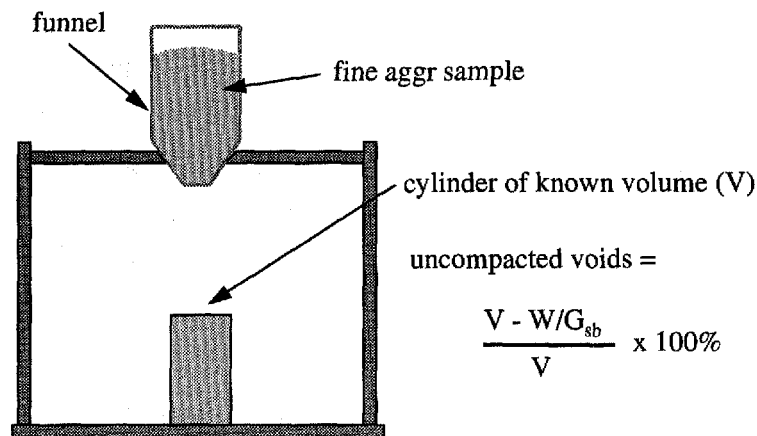
Figure III-5. Fine Aggregate Angularity Apparatus
