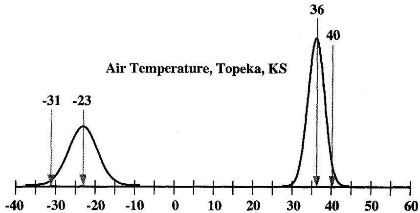
Figure III-2. Distribution of High and Low Design Air Temperatures for Topeka, KS
