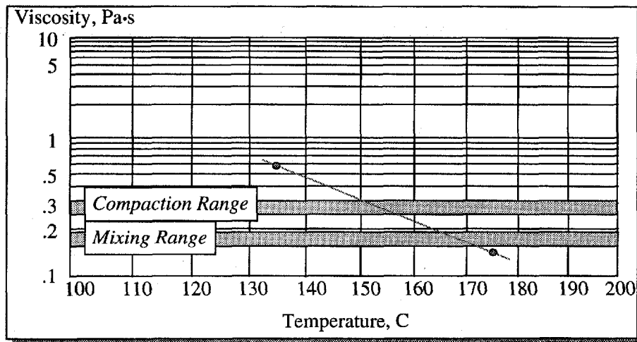
Figure V-4. Temperature-Viscosity Relationship
