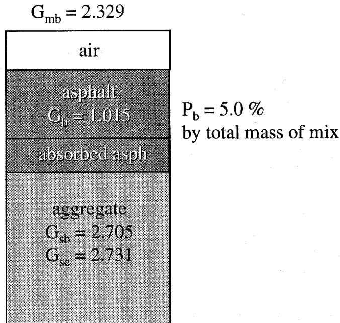
Figure IV-5. Known Items for Example
