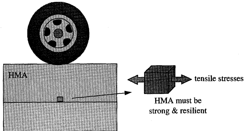
Figure I-13. Tensile Stresses at Bottom of HMA Layer
