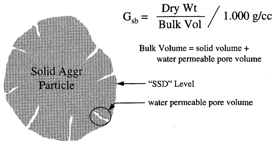
Figure IV-2. Bulk Specific Gravity of Aggregate
