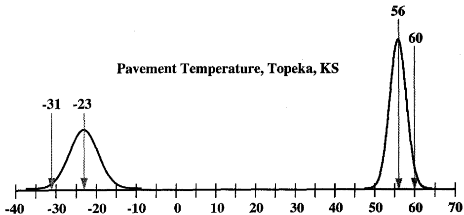
Figure III-3. Distribution of High and Low Design Pavement Temperatures for Topeka, KS
