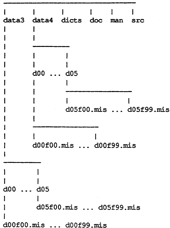
Figure 3. CD-ROM directory tree structure.
