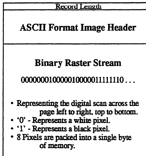
Figure 4. IHead file layout.
