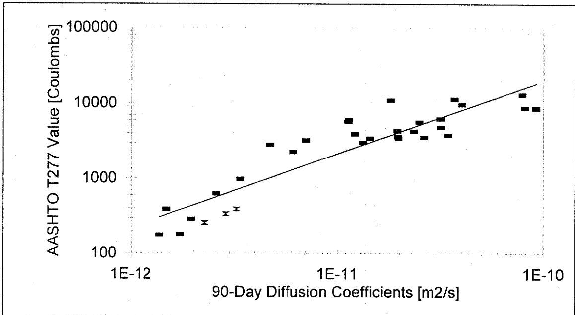
Figure 54. AASHTO T277 – 28 Days vs. 90-Day Bulk Diffusion Highlighting Metakaolin Subset ( X ).
