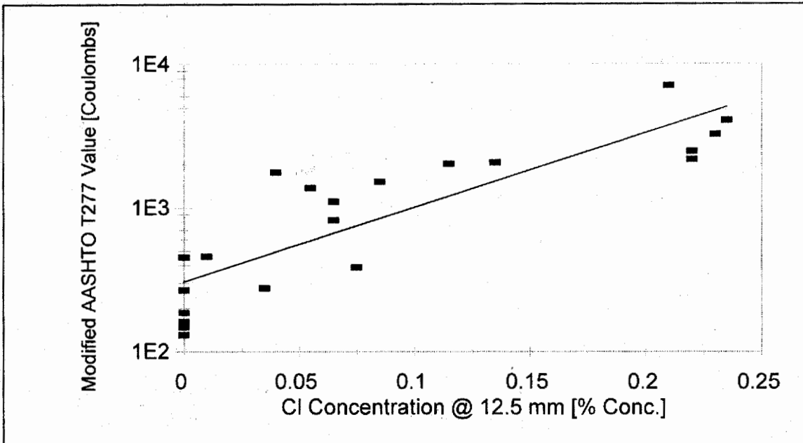
Figure 75. Modified AASHTO T277 – 393 Days vs. Salt Ponding Evaluation.
