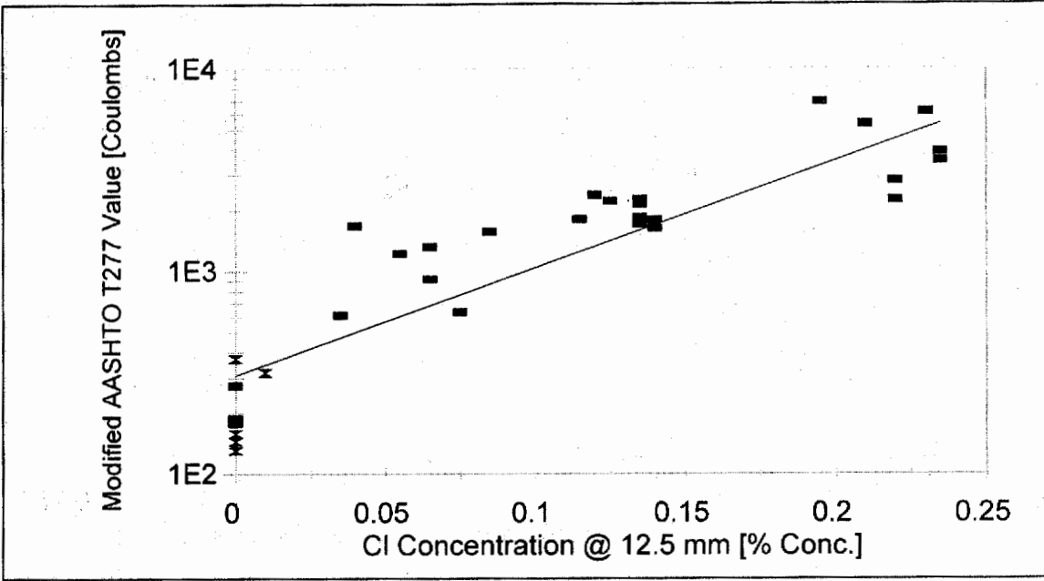
Figure 74. Modified AASHTO T277 – 118 Days vs. Salt Ponding Evaluation Highlighting Silica Fume Subset ( X ).
