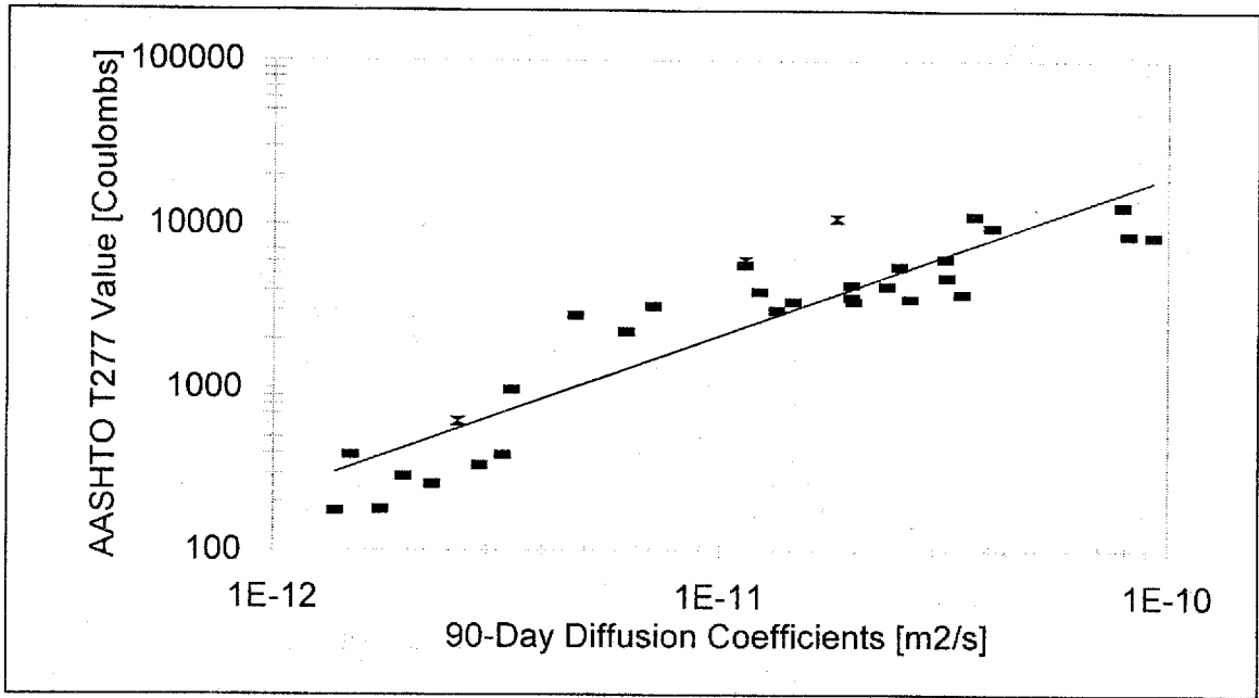
Figure 53. AASHTO T277 – 28 Days vs. 90-Day Bulk Diffusion Highlighting DCI Subset ( X ).
