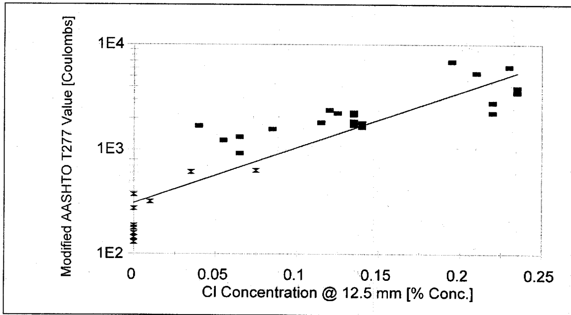
Figure 73. Modified AASHTO T277 – 118 Days vs. Salt Ponding Evaluation Highlighting SCM Subset ( X ).
