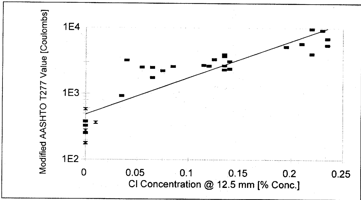
Figure 72. Modified AASHTO T277 – 28 Days vs. Salt Ponding Evaluation Highlighting Silica Fume Subset ( X ).
