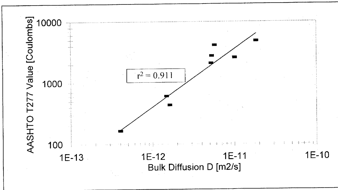
Figure 14. AASHTO T277 vs. 365-Day Bulk Diffusion.
