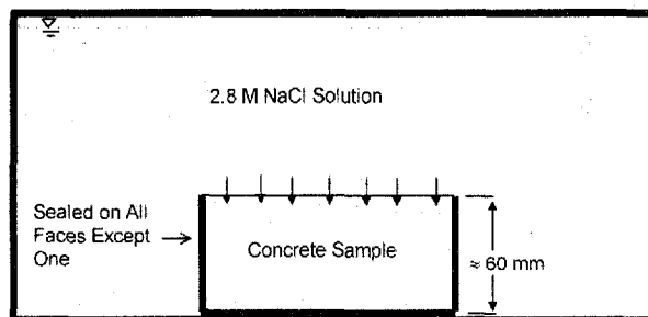
Figure 2. NordTest Setup.
