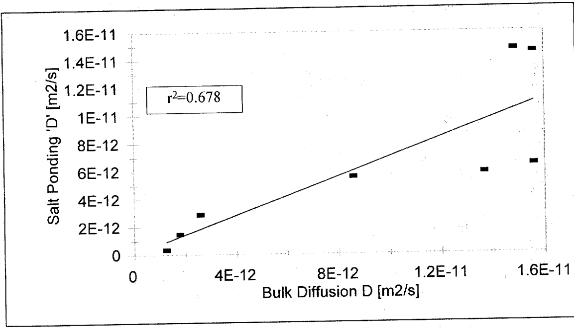
Figure 5. Salt Ponging Pseudo-D vs. 40-Day Bulk Diffusion.
