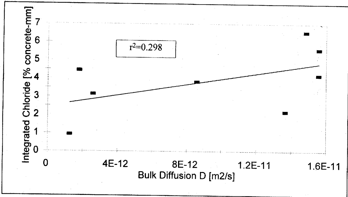
Figure 3. Salt Ponding Integrated Chloride vs. 40-Day Bulk Diffusion.
