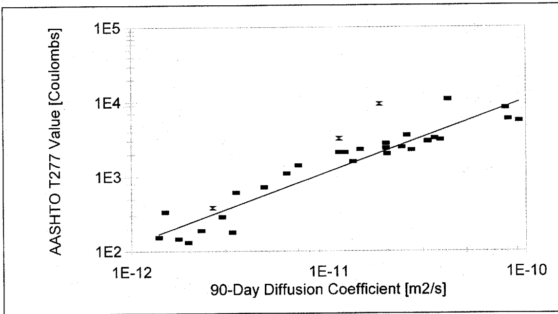
Figure 55. AASHTO T277 – 118 Days vs. 90-Day Bulk Diffusion Highlighting DCI Subset ( X ).
