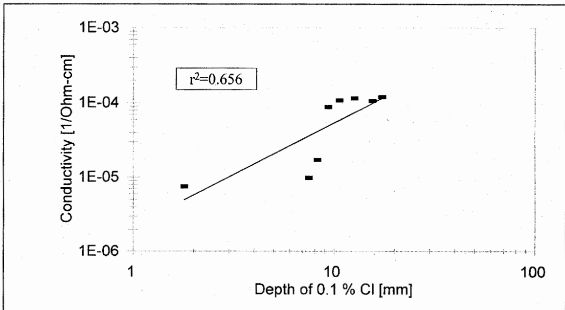
Figure 37. Conductivity (Monfore) vs. 90-Day Salt Ponding Depth of Penetration.
