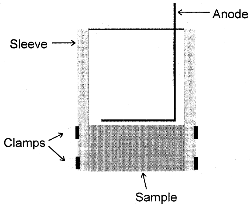
Figure 2. Assembly Diagram.
