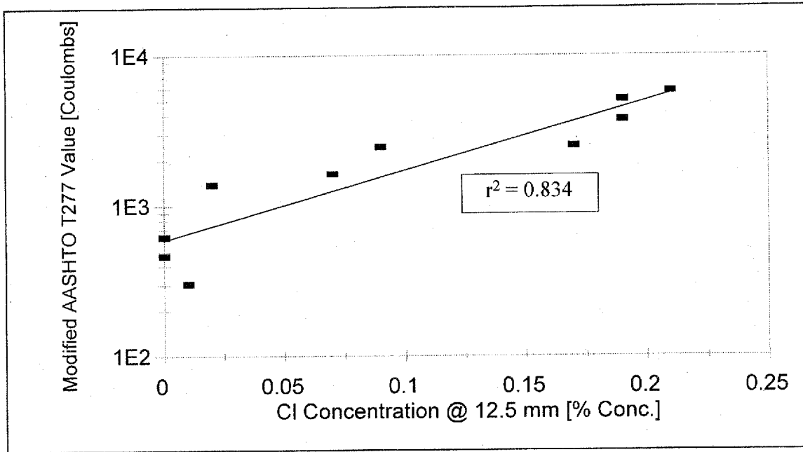
Figure 105. Modified AASHTO T277, 28 Days vs. Salt Ponding Evaluation.
