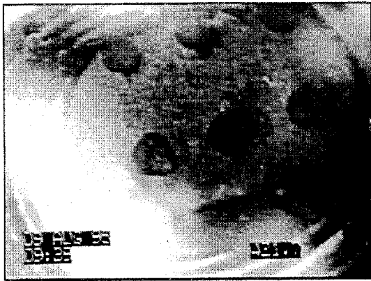
Here is a case where only the first 20 ft of the edgedrain was pipe. After this the edgedrain was an aggregate trench (French Drain). This individual wanted to keep the aggregate material out of the pipe so he used a brick as a stopper. Yet he wanted the aggregate trench to drain into the pipe so he used a brick with holes in it.
